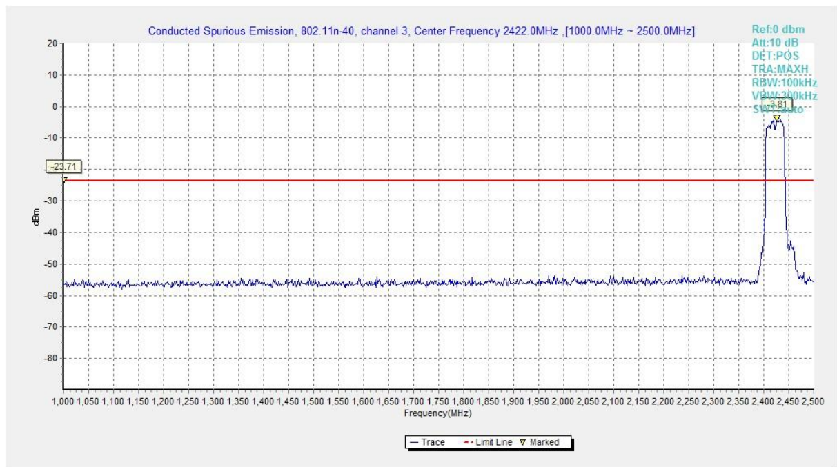
Fig.A.7.1.75 Conducted Spurious Emission (802.11n-HT40, Ch3, 1 GHz-2.5 GHz)
