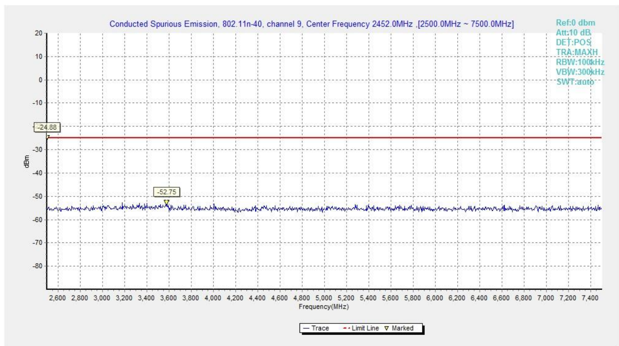
Fig.A.7.1.92 Conducted Spurious Emission (802.11n-HT40, Ch9, 2.5 GHz-7.5 GHz)
