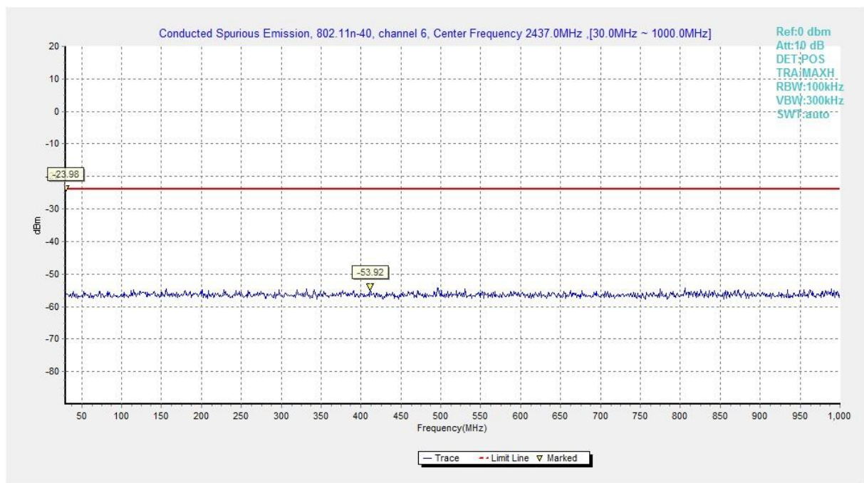
Fig.A.7.1.82 Conducted Spurious Emission (802.11n-HT40, Ch6, 30 MHz-1 GHz)
