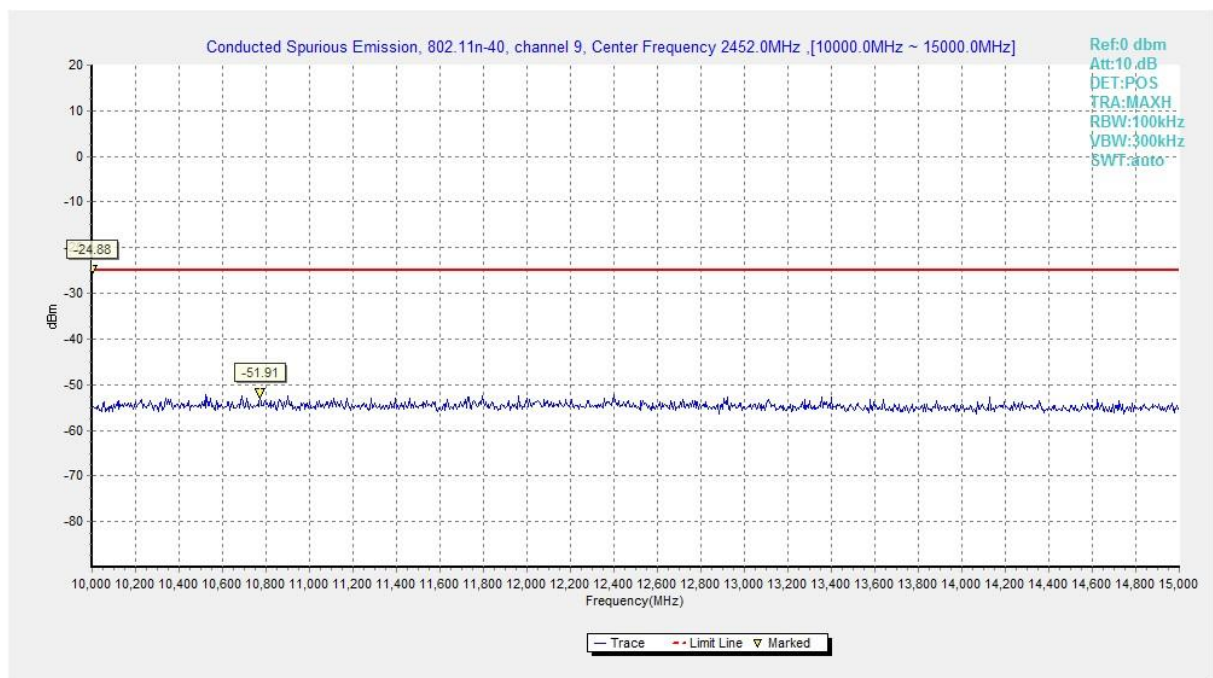
Fig.A.7.1.94 Conducted Spurious Emission (802.11n-HT40, Ch9, 10 GHz-15 GHz)
