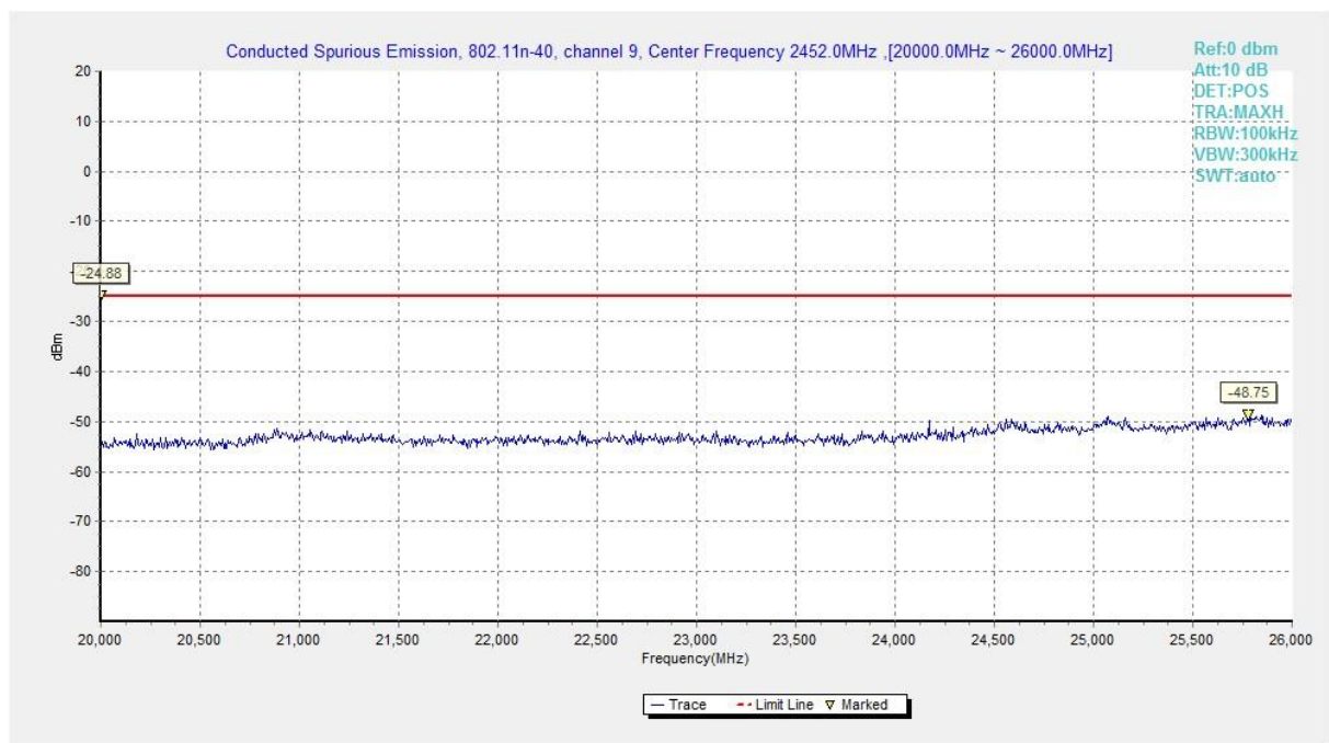
Fig.A.7.1.96 Conducted Spurious Emission (802.11n-HT40, Ch9, 20 GHz-26 GHz)
