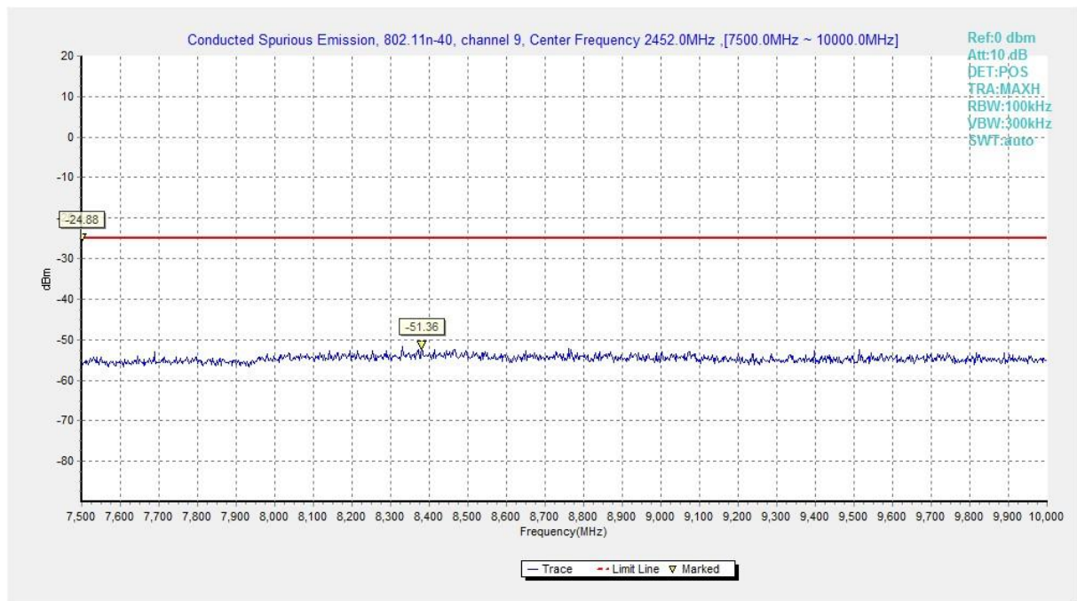
Fig.A.7.1.93 Conducted Spurious Emission (802.11n-HT40, Ch9, 7.5 GHz-10 GHz)
