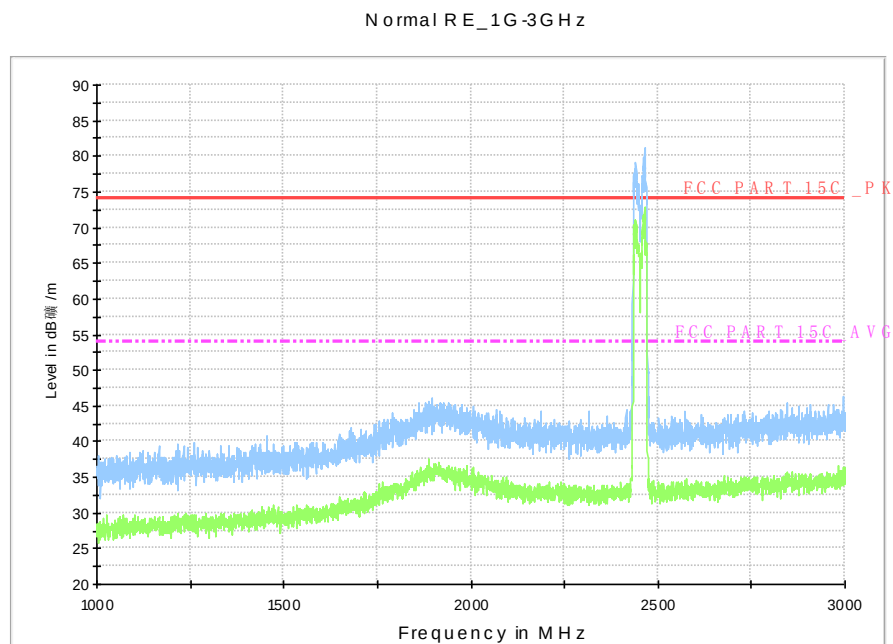
Fig.A.7.2.43 Radiated Spurious Emission (802.11n-HT40, ch9, 1 GHz-3 GHz)
