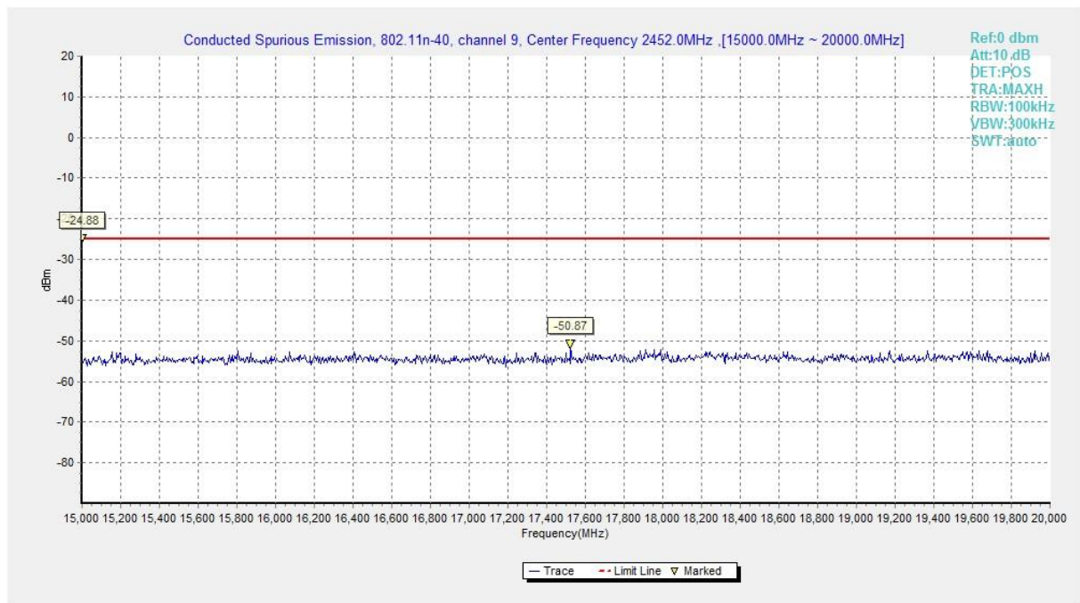
Fig.A.7.1.95 Conducted Spurious Emission (802.11n-HT40, Ch9, 15 GHz-20 GHz)
