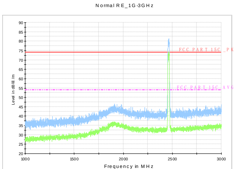
Fig.A.7.2.32 Radiated Spurious Emission (802.11n-HT20, Ch11, 1 GHz-3 GHz)
