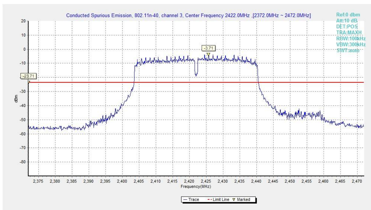
Fig.A.7.1.73 Conducted Spurious Emission (802.11n-HT40, Ch3, Center Frequency)
