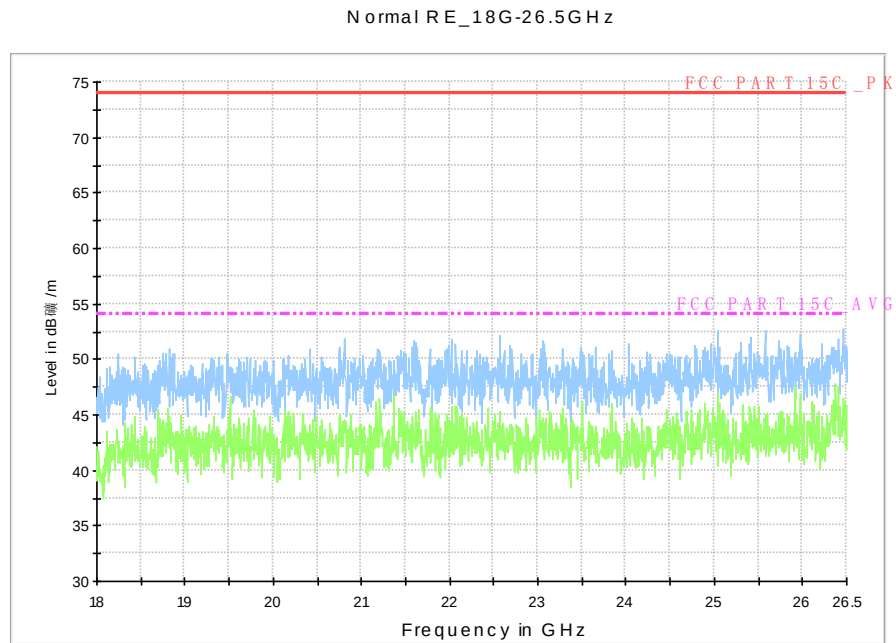
Fig.A.7.2.45 Radiated Spurious Emission (All channels): 18GHz – 26.5GHz
