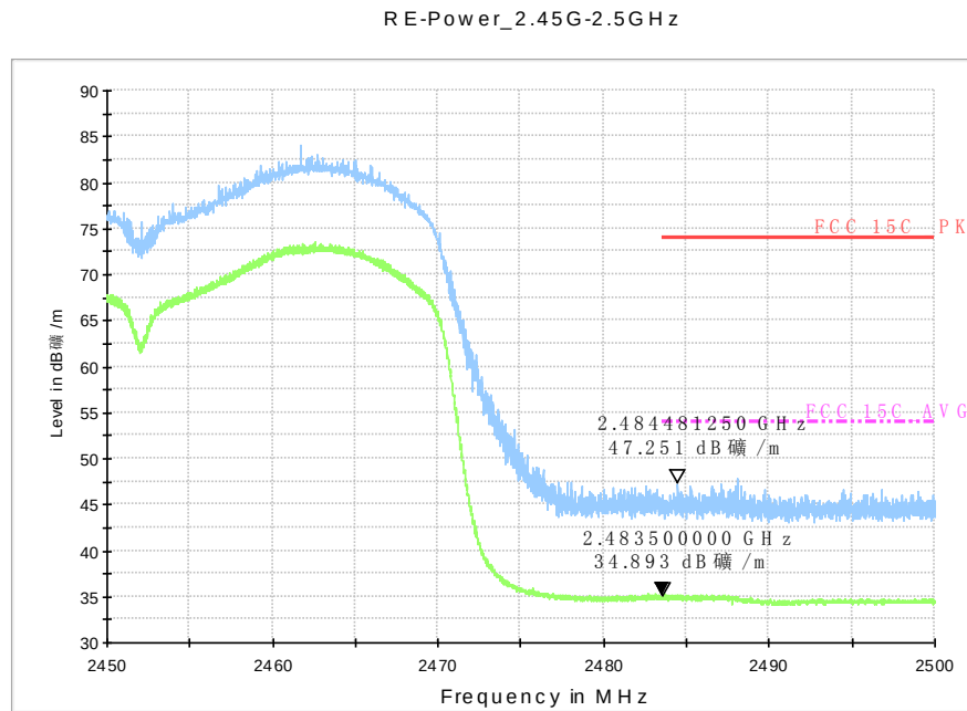
Fig.A.7.2.41 Radiated Spurious Emission (Power): 802.11n-HT40, ch9, 2.45 GHz - 2.50GHz
