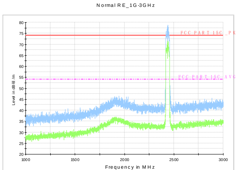
Fig.A.7.2.39 Radiated Spurious Emission (802.11n-HT40, Ch6, 1 GHz-3 GHz)
