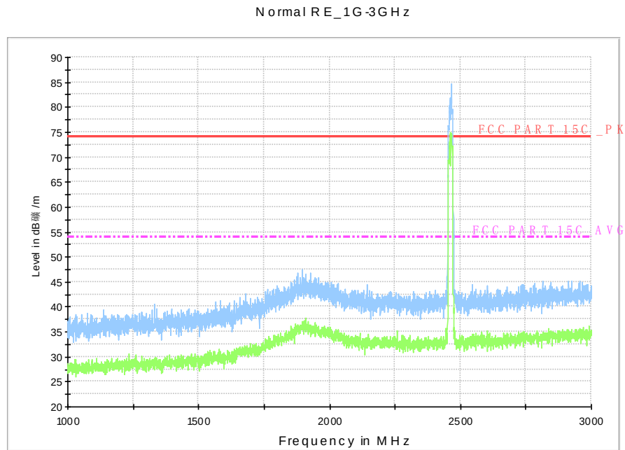
Fig.A.7.2.21 Radiated Spurious Emission (802.11g, Ch11, 1 GHz-3 GHz)
