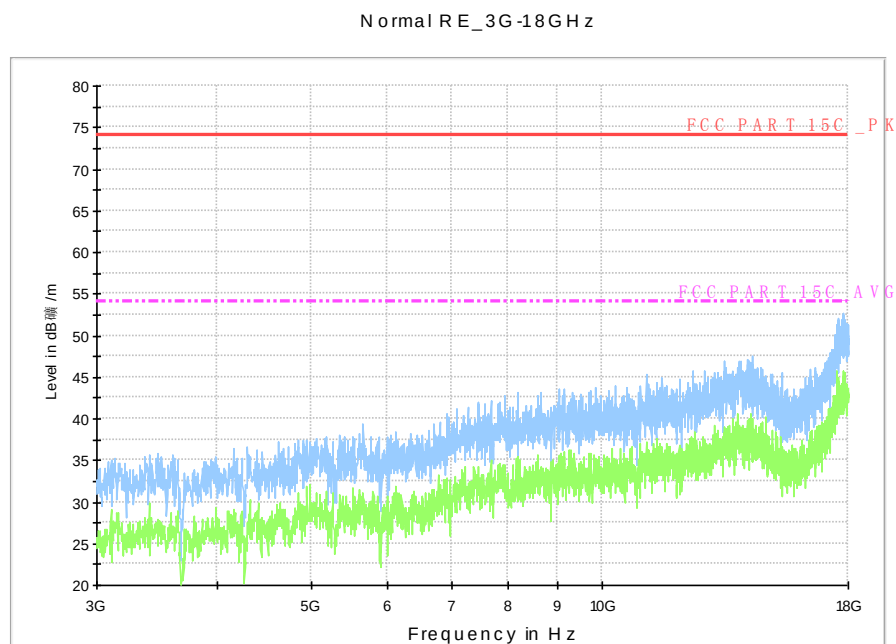
Fig.A.7.2.26 Radiated Spurious Emission (802.11n-HT20, Ch1, 3 GHz-18 GHz)
