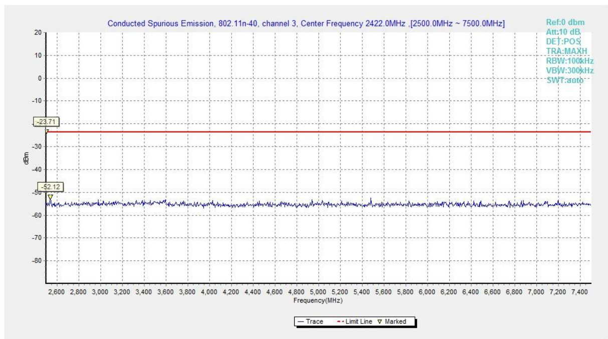
Fig.A.7.1.76 Conducted Spurious Emission (802.11n-HT40, Ch3, 2.5 GHz-7.5 GHz)
