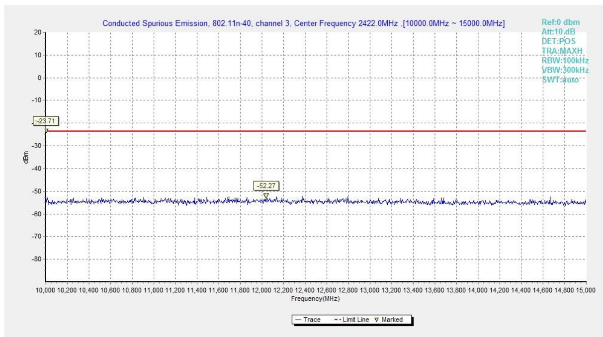
Fig.A.7.1.78 Conducted Spurious Emission (802.11n-HT40, Ch3, 10 GHz-15 GHz)
