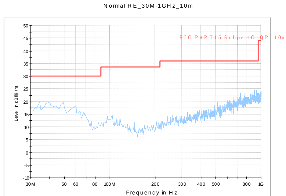
Fig.A.7.2.38 Radiated Spurious Emission (802.11n-HT40, Ch6, 30 MHz-1 GHz)
