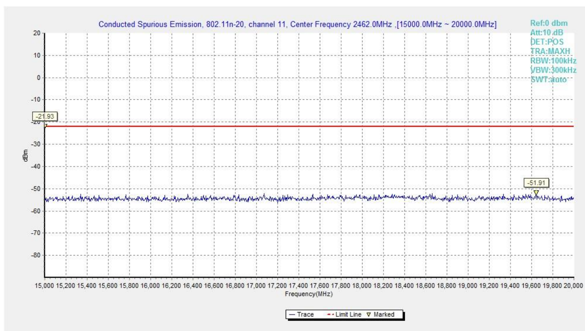
Fig.A.7.1.71 Conducted Spurious Emission (802.11n-HT20, Ch11, 15 GHz-20 GHz)
