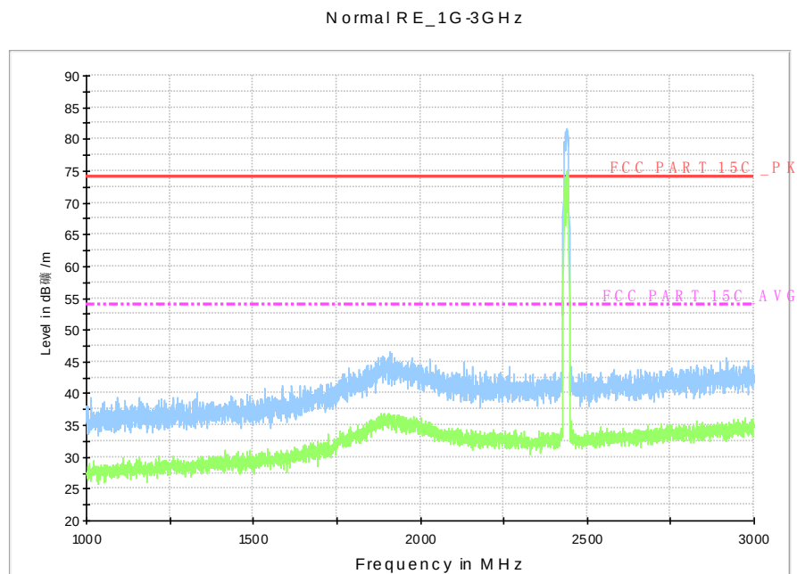
Fig.A.7.2.17 Radiated Spurious Emission (802.11g, Ch6, 1 GHz-3 GHz)
