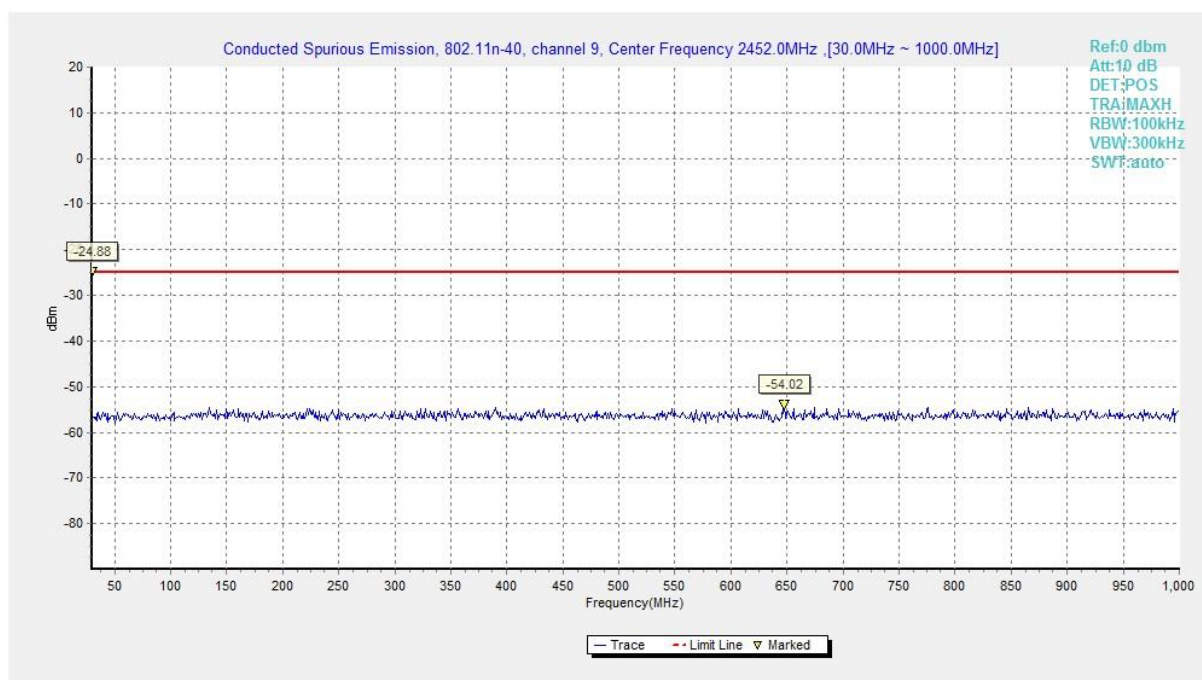
Fig.A.7.1.90 Conducted Spurious Emission (802.11n-HT40, Ch9, 30 MHz-1 GHz)
