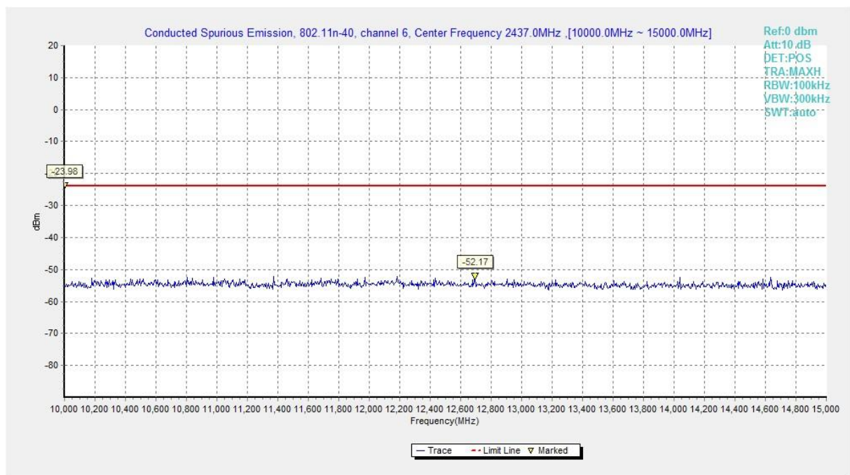
Fig.A.7.1.86 Conducted Spurious Emission (802.11n-HT40, Ch6, 10 GHz-15 GHz)
