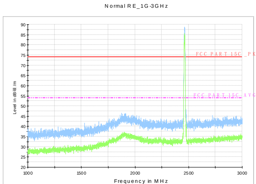
Fig.A.7.2.10 Radiated Spurious Emission (802.11b, Ch11, 1 GHz-3 GHz)
