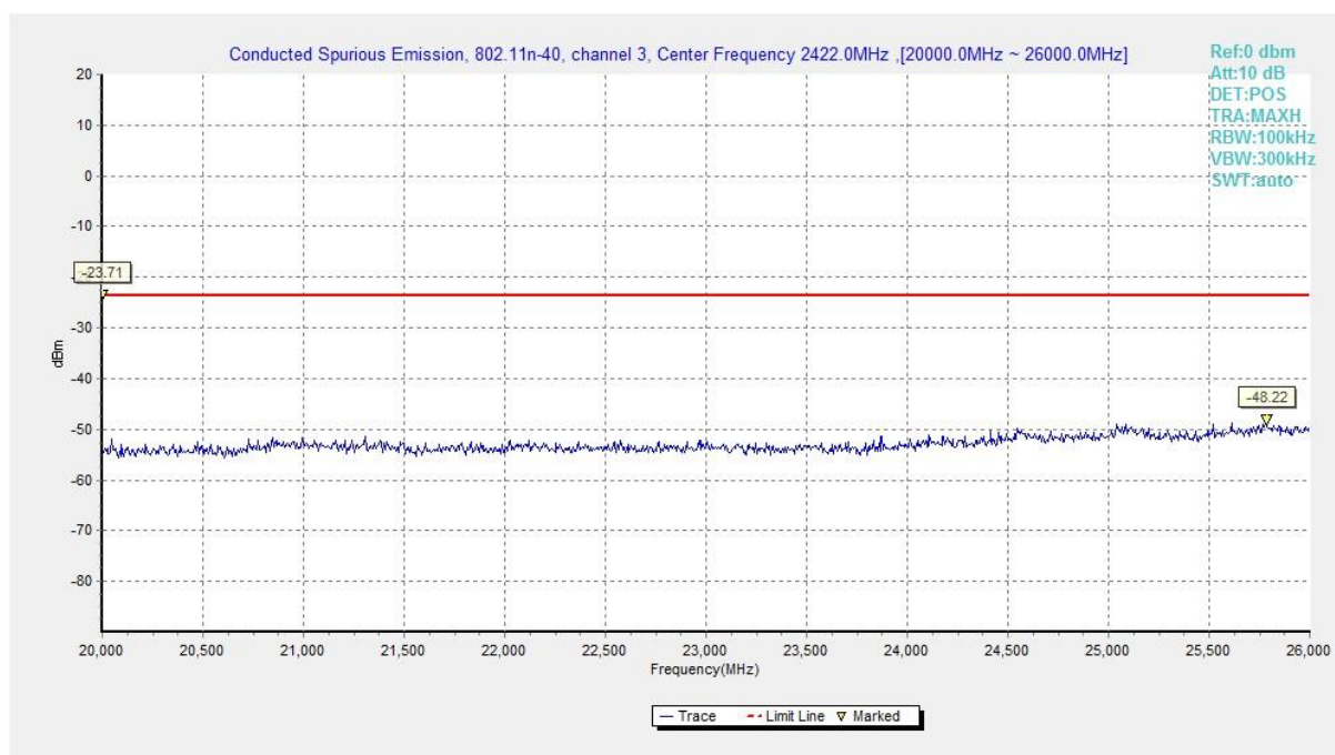
Fig.A.7.1.80 Conducted Spurious Emission (802.11n-HT40, Ch3, 20 GHz-26 GHz)
