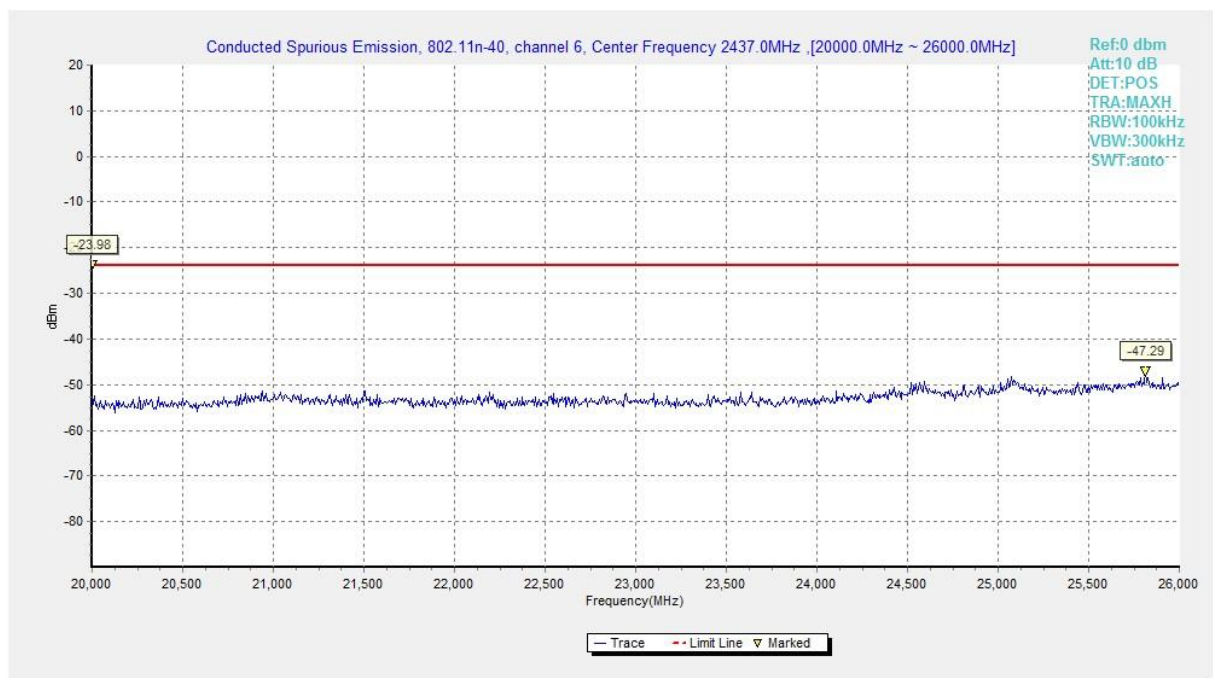
Fig.A.7.1.88 Conducted Spurious Emission (802.11n-HT40, Ch6, 20 GHz-26 GHz)
