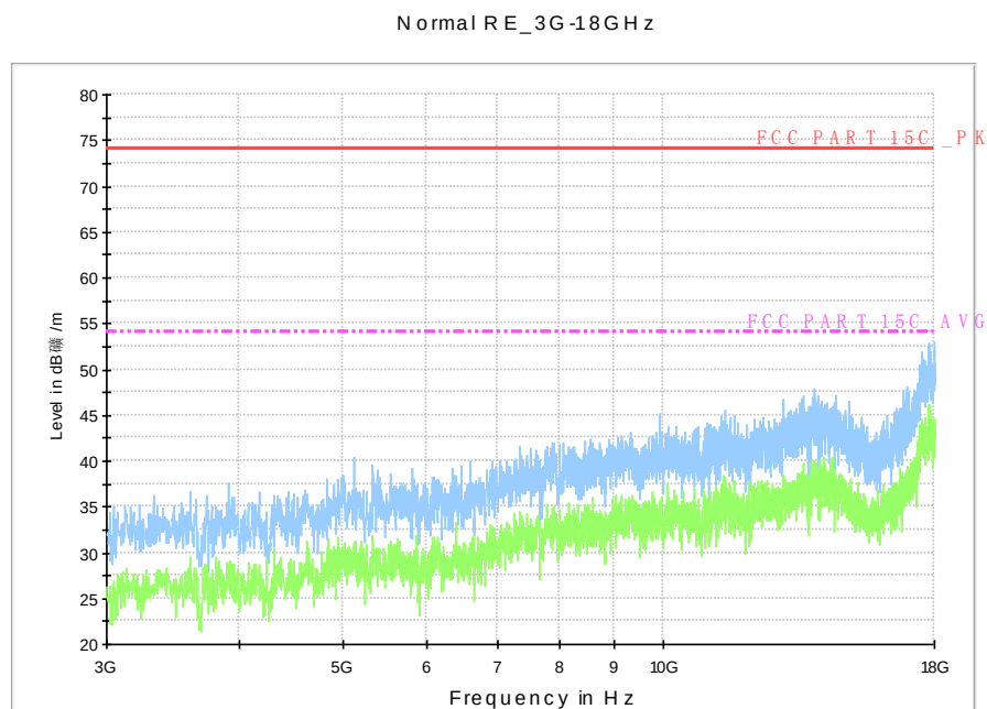
Fig.A.7.2.18 Radiated Spurious Emission (802.11g, Ch6, 3 GHz-18 GHz)
