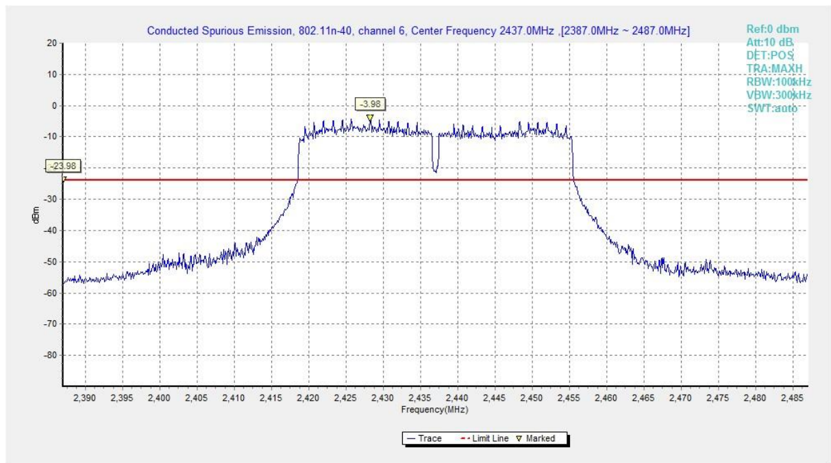
Fig.A.7.1.81 Conducted Spurious Emission (802.11n-HT40, Ch6, Center Frequency)
