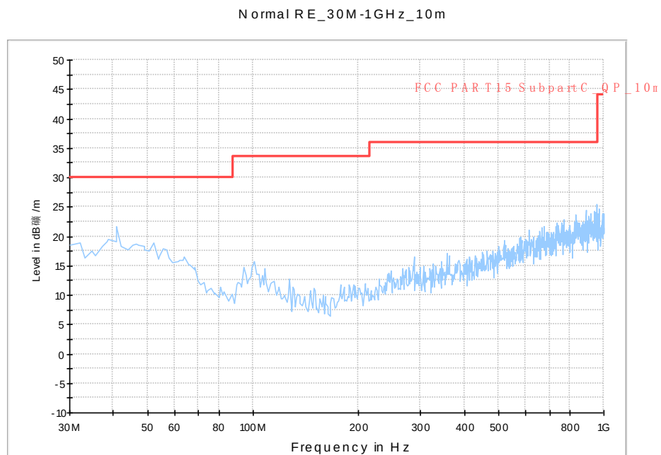
Fig.A.7.2.35 Radiated Spurious Emission (802.11n-HT40, ch3, 30 MHz-1 GHz)
