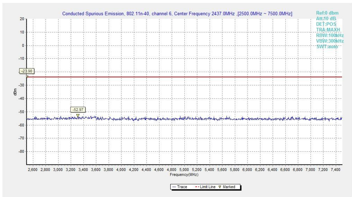
Fig.A.7.1.84 Conducted Spurious Emission (802.11n-HT40, Ch6, 2.5 GHz-7.5 GHz)
