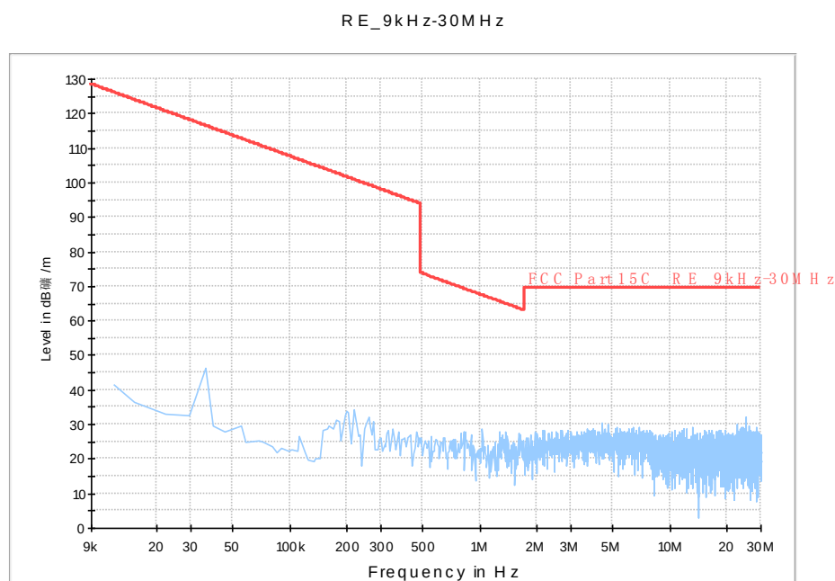
Fig.A.8.1 Radiated Spurious Emission (802.11b, 9 kHz ~30 MHz)
