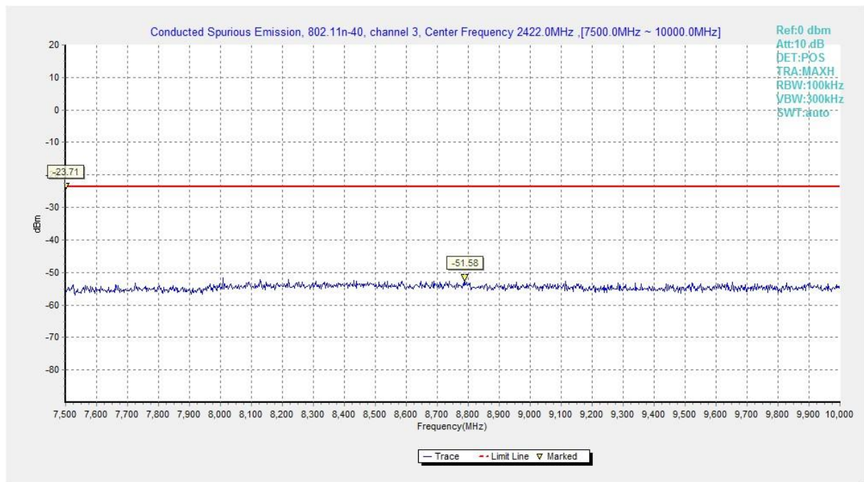
Fig.A.7.1.77 Conducted Spurious Emission (802.11n-HT40, Ch3, 7.5 GHz-10 GHz)
