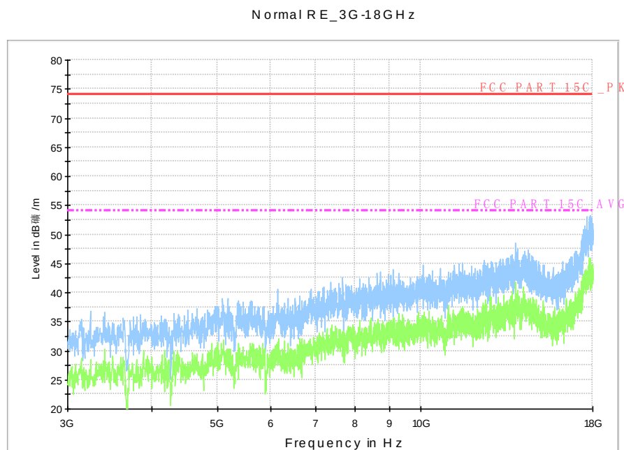
Fig.A.7.2.40 Radiated Spurious Emission (802.11n-HT40, Ch6, 3 GHz-18 GHz)
