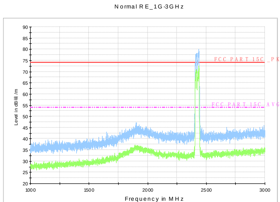
Fig.A.7.2.36 Radiated Spurious Emission (802.11n-HT40, ch3, 1 GHz-3 GHz)
