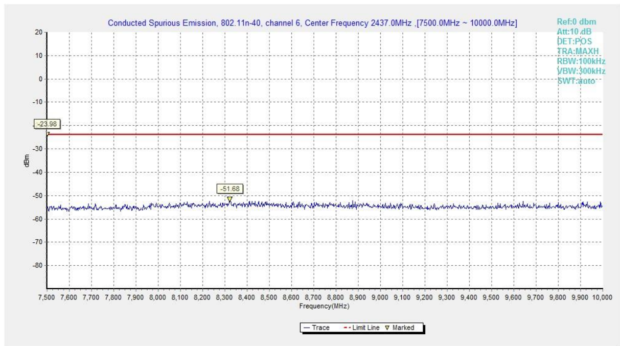
Fig.A.7.1.85 Conducted Spurious Emission (802.11n-HT40, Ch6, 7.5 GHz-10 GHz)
