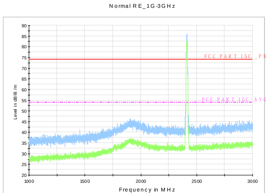
Fig.A.7.2.3 Radiated Spurious Emission (802.11b, Ch1, 1 GHz-3 GHz)
