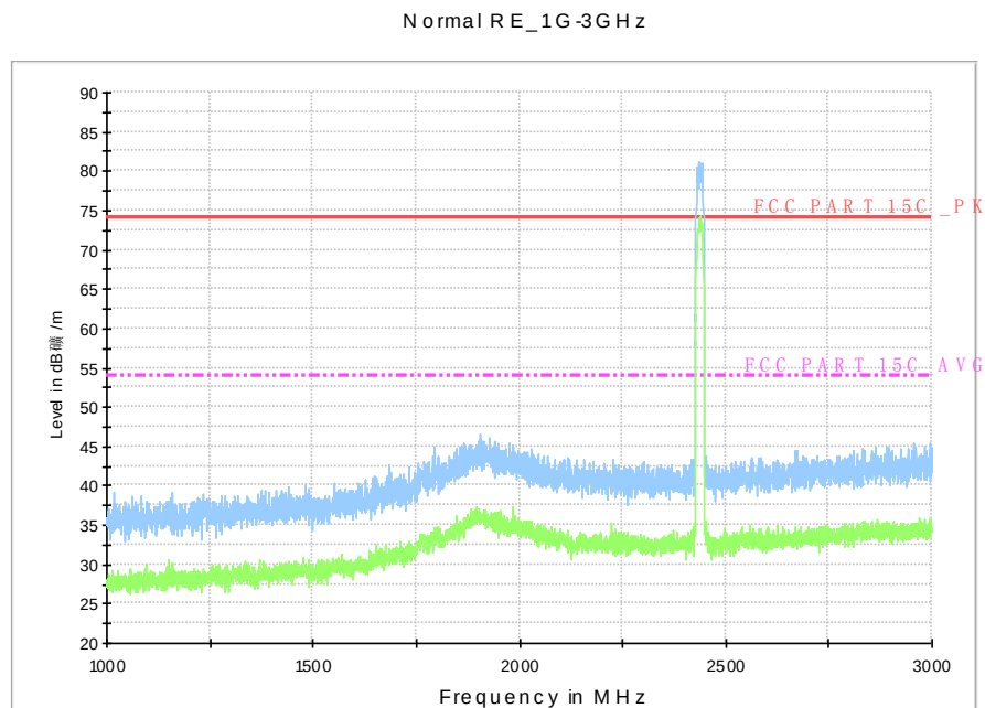
Fig.A.7.2.28 Radiated Spurious Emission (802.11n-HT20, Ch6, 1 GHz-3 GHz)
