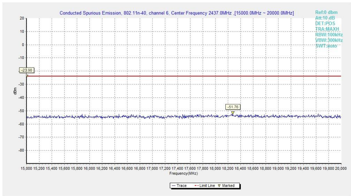
Fig.A.7.1.87 Conducted Spurious Emission (802.11n-HT40, Ch6, 15 GHz-20 GHz)
