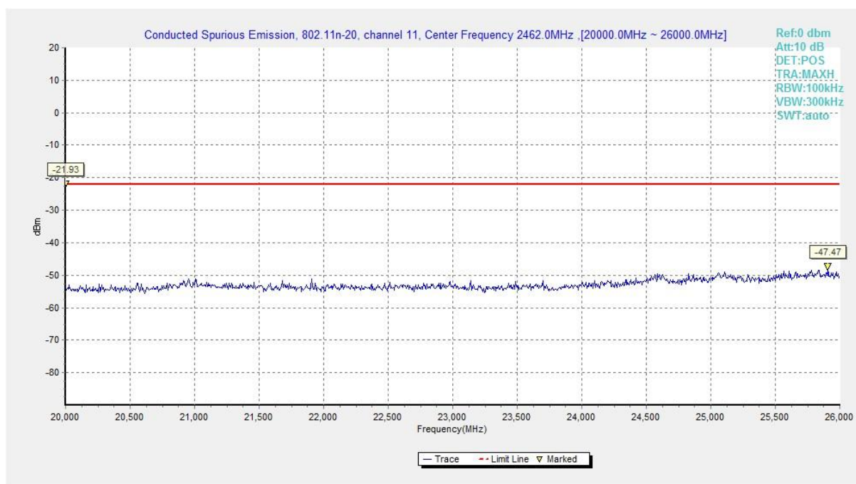
Fig.A.7.1.72 Conducted Spurious Emission (802.11n-HT20, Ch11, 20 GHz-26 GHz)
