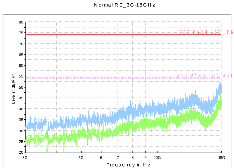
Fig.A.7.2.22 Radiated Spurious Emission (802.11g, Ch11, 3 GHz-18 GHz)
