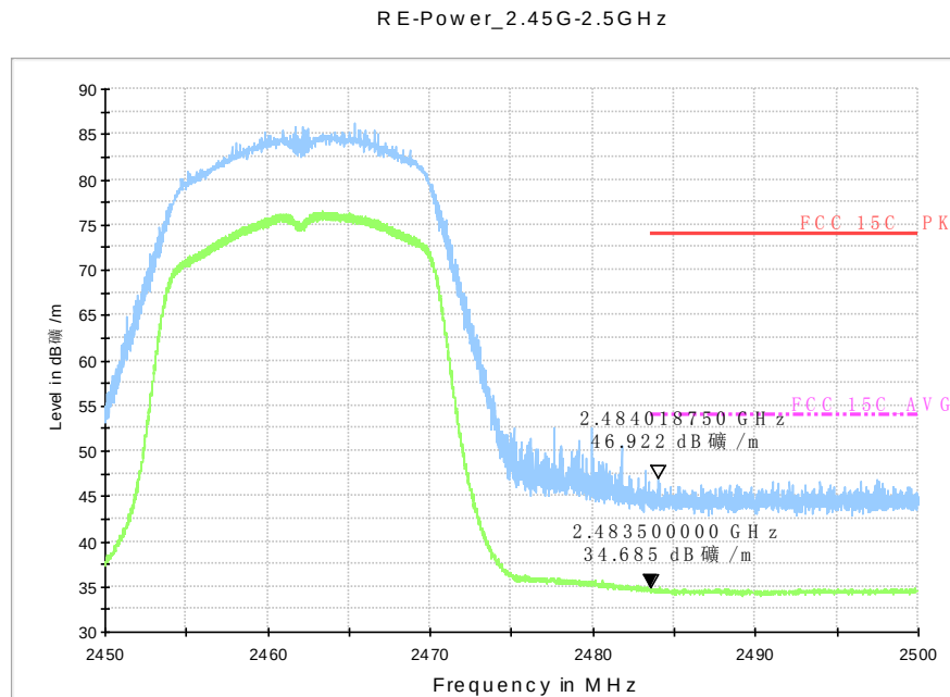
Fig.A.7.2.19 Radiated Spurious Emission (Power): 802.11g, ch11, 2.45 GHz - 2.50GHz
