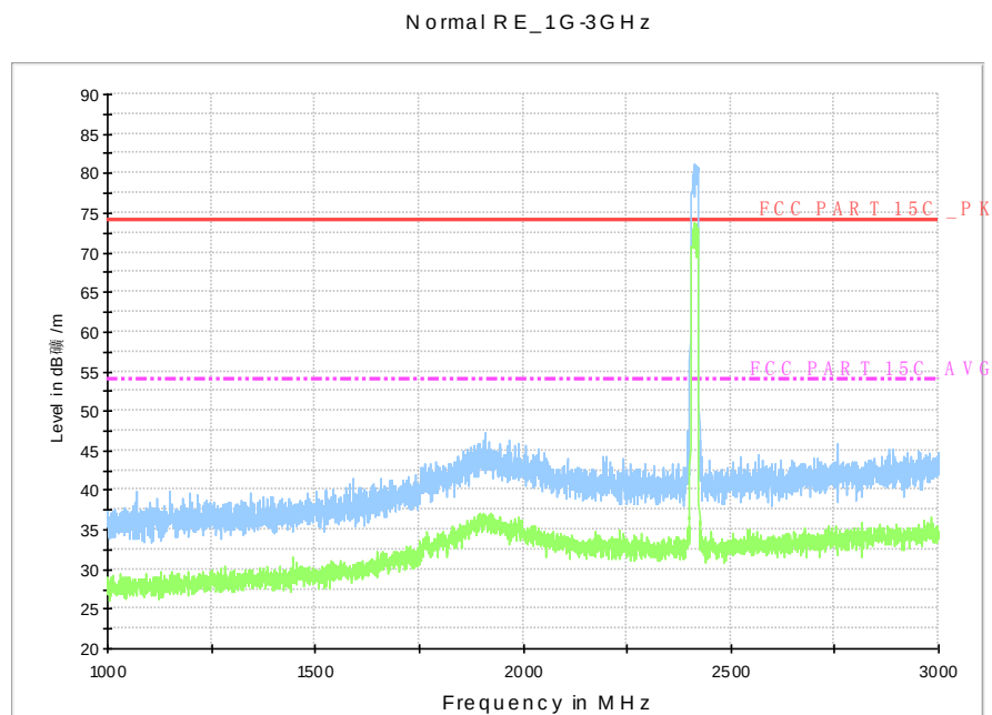
Fig.A.7.2.25 Radiated Spurious Emission (802.11n-HT20, Ch1, 1 GHz-3 GHz)
