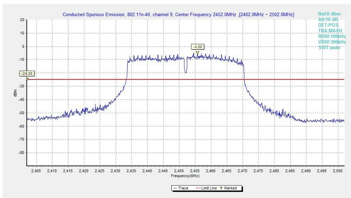
Fig.A.7.1.89 Conducted Spurious Emission (802.11n-HT40, Ch9, Center Frequency)
