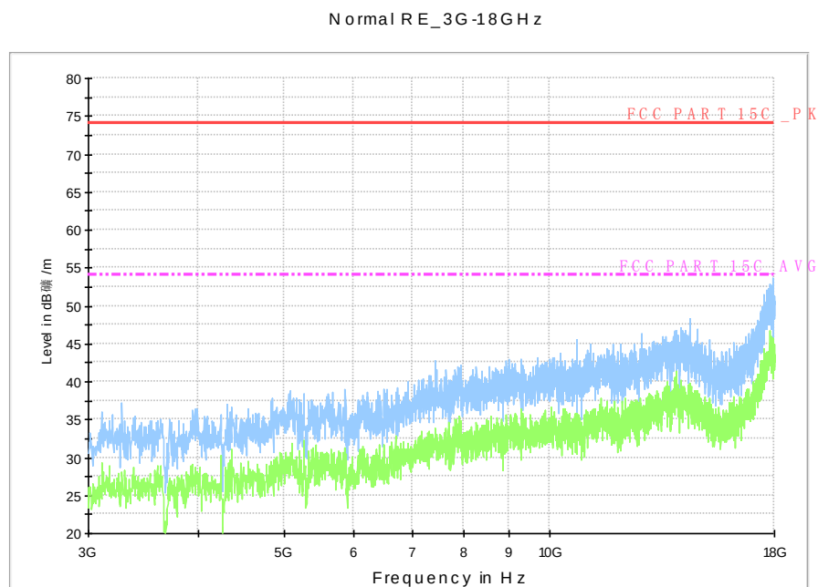
Fig.A.7.2.44 Radiated Spurious Emission (802.11n-HT40, ch9, 3 GHz-18 GHz)
