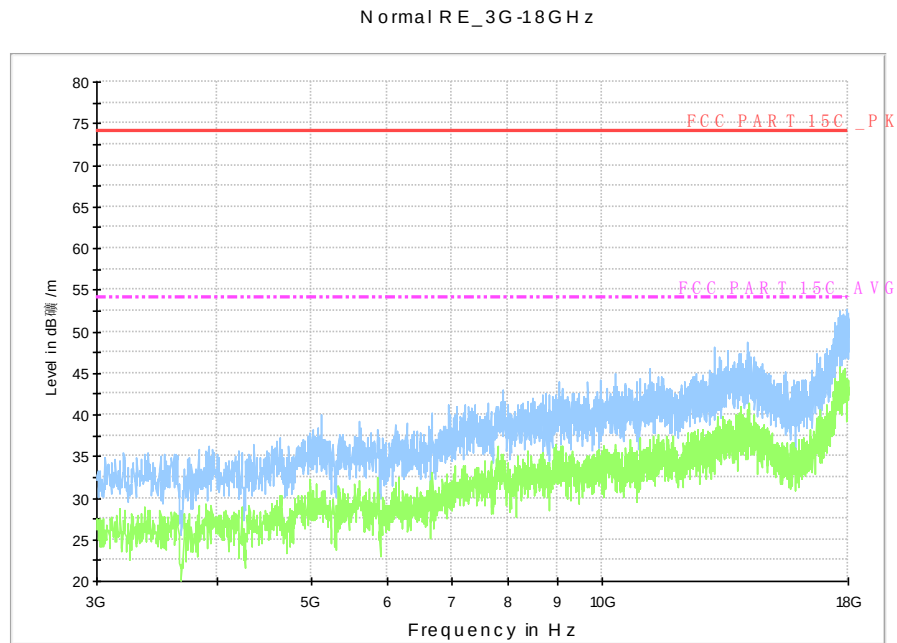
Fig.A.7.2.37 Radiated Spurious Emission (802.11n-HT40, ch3, 3 GHz-18 GHz)
