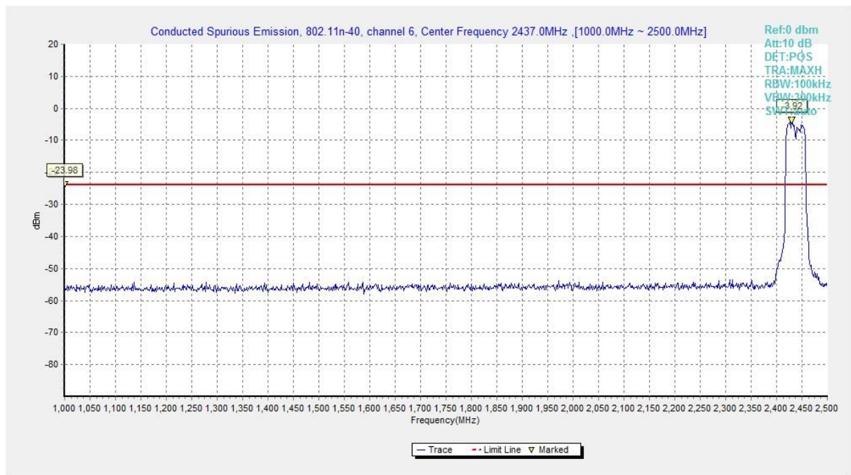
Fig.A.7.1.83 Conducted Spurious Emission (802.11n-HT40, Ch6, 1 GHz-2.5 GHz)
