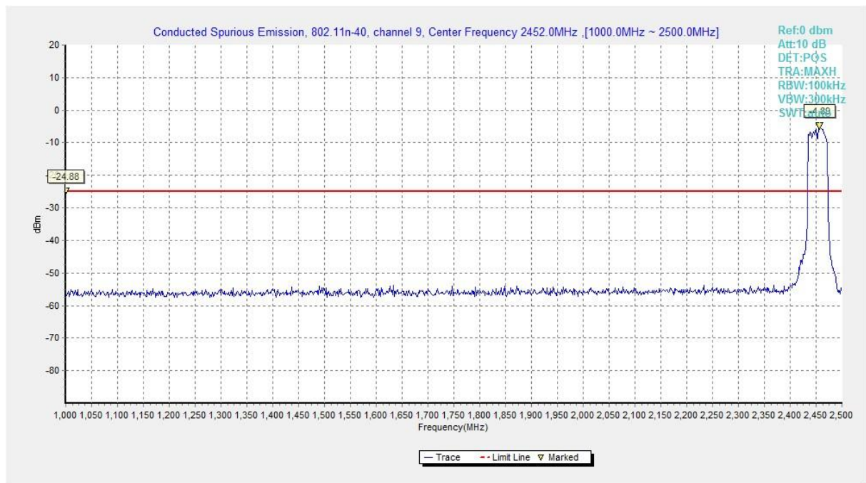
Fig.A.7.1.91 Conducted Spurious Emission (802.11n-HT40, Ch9, 1 GHz-2.5 GHz)
