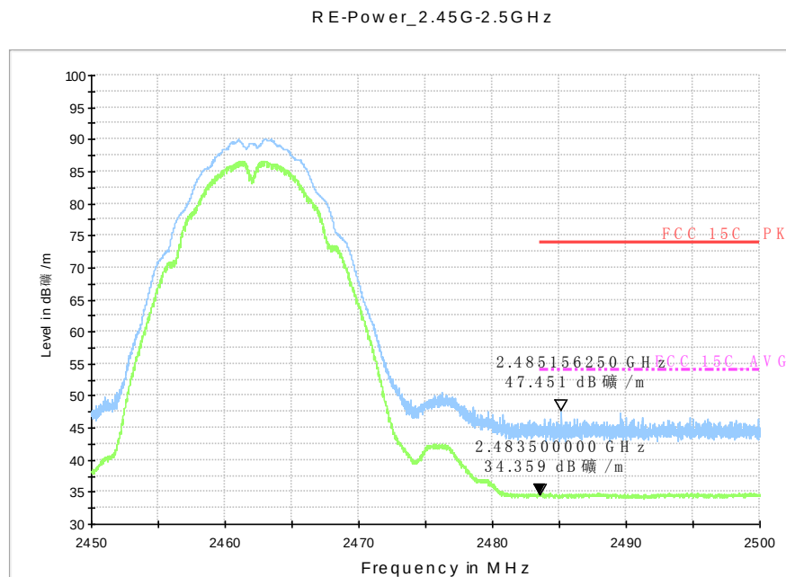
Fig.A.7.2.8 Radiated Spurious Emission (Power): 802.11b, ch11, 2.45 GHz - 2.50GHz
