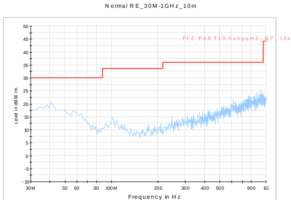
Fig.A.7.2.42 Radiated Spurious Emission (802.11n-HT40, ch9, 30 MHz-1 GHz)
