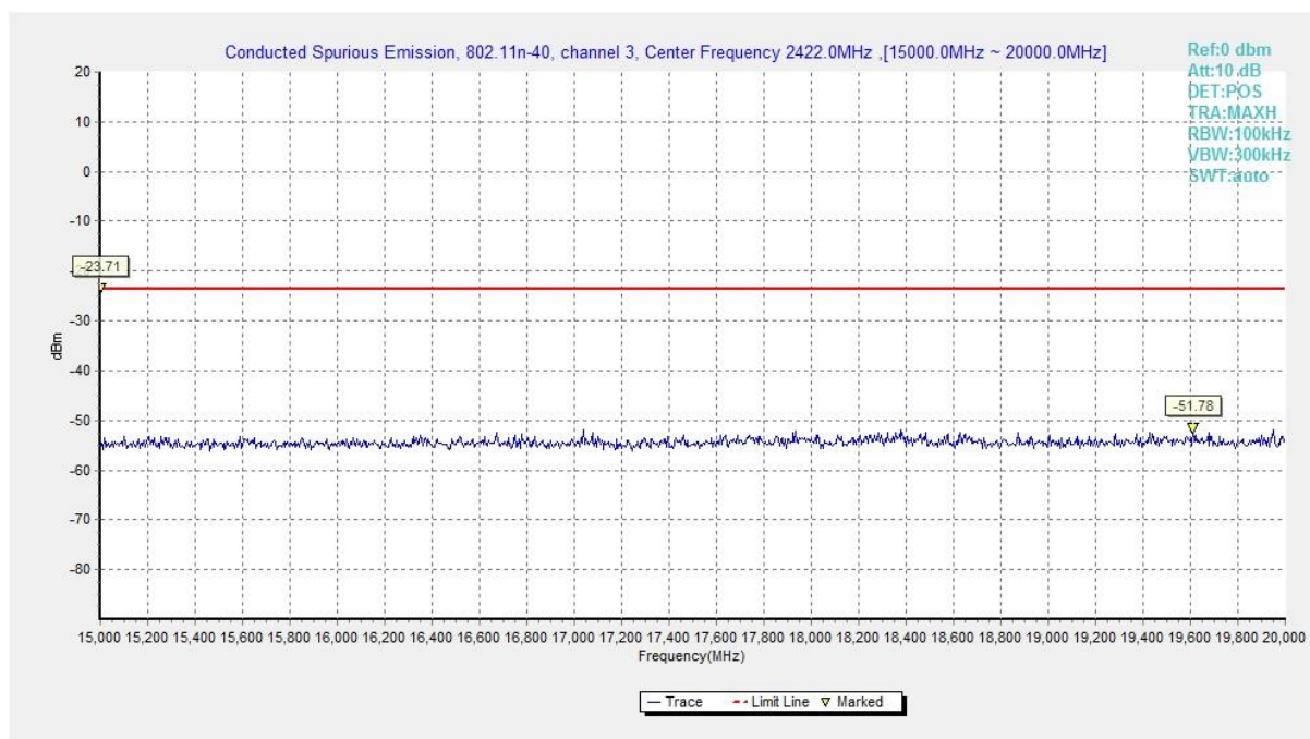
Fig.A.7.1.79 Conducted Spurious Emission (802.11n-HT40, Ch3, 15 GHz-20 GHz)
