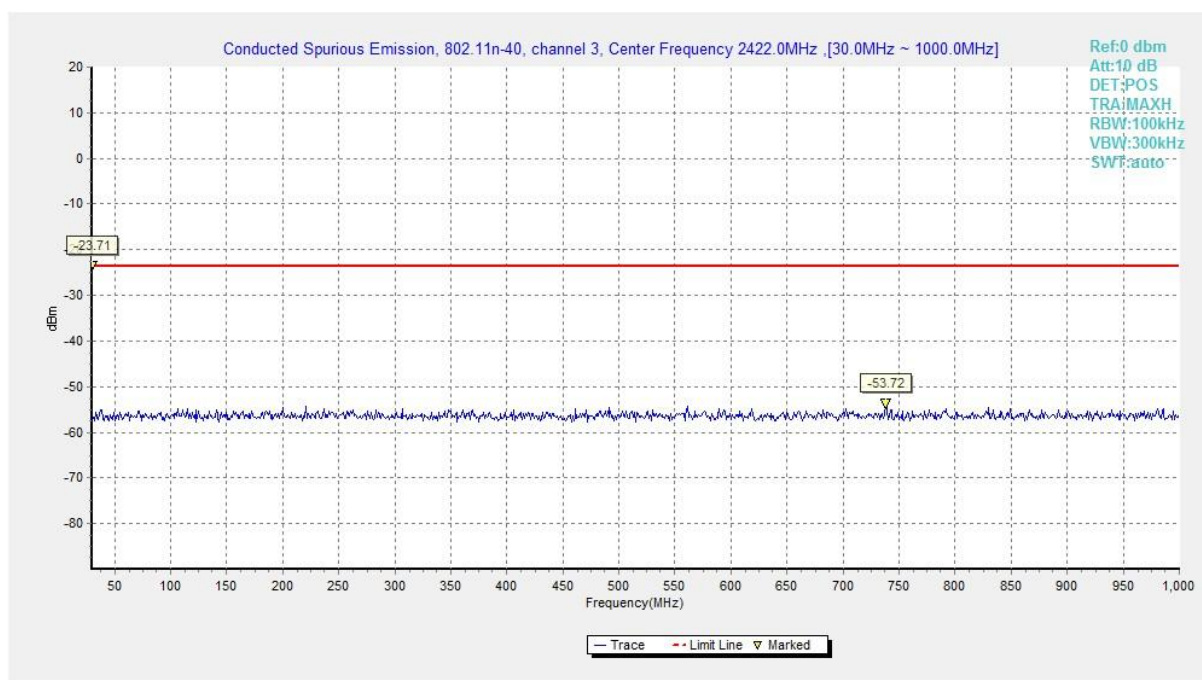
Fig.A.7.1.74 Conducted Spurious Emission (802.11n-HT40, Ch3, 30 MHz-1 GHz)
