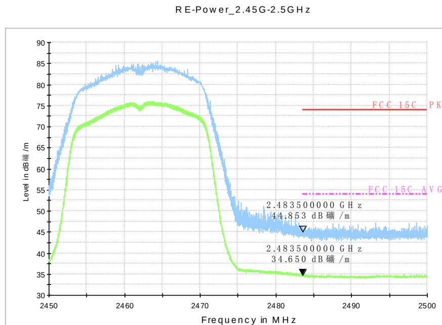
Fig.A.7.2.30 Radiated Spurious Emission (Power): 802.11n-HT20, ch11, 2.45 GHz - 2.50GHz
