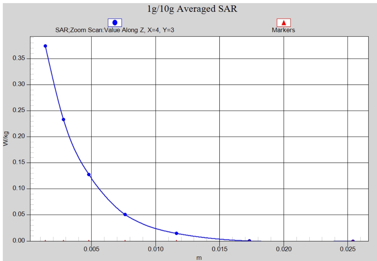
Fig. 24-1 Z-Scan at power reference point (5GHz CH48)
