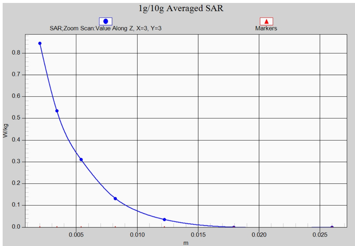
Fig. 25-1 Z-Scan at power reference point (5GHz CH52)
