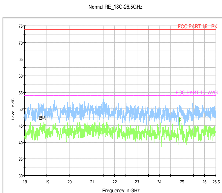
Fig.27. Radiated emission (Power) GFSK, high channel
