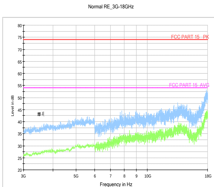
Fig.25. Radiated emission: GFSK, 2480MHz, 3 GHz - 18 GHz
