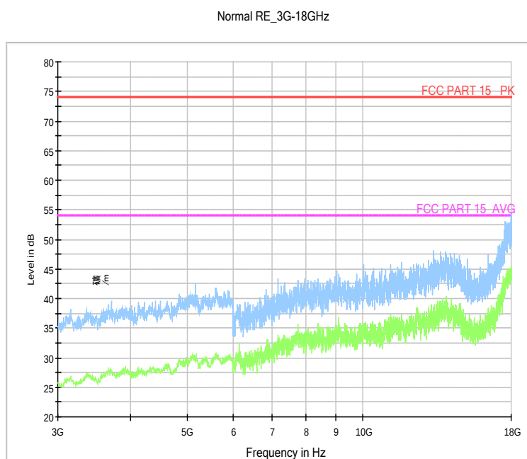
Fig.23. Radiated emission: GFSK, 2440MHz, 3 GHz - 18 GHz
