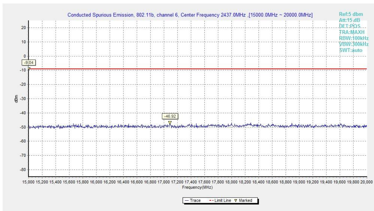
Fig.A.6.1.15 Conducted Spurious Emission (802.11b, Ch6, 15 GHz-20 GHz)
