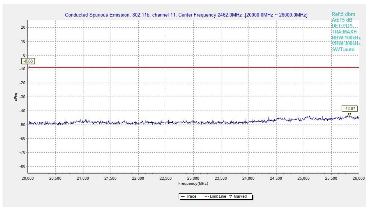
Fig.A.6.1.24 Conducted Spurious Emission (802.11b, Ch11, 20 GHz-26 GHz)
