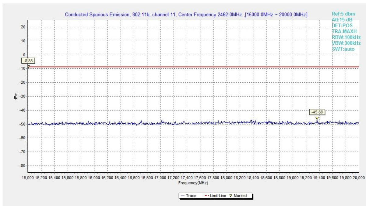
Fig.A.6.1.23 Conducted Spurious Emission (802.11b, Ch11, 15 GHz-20 GHz)
