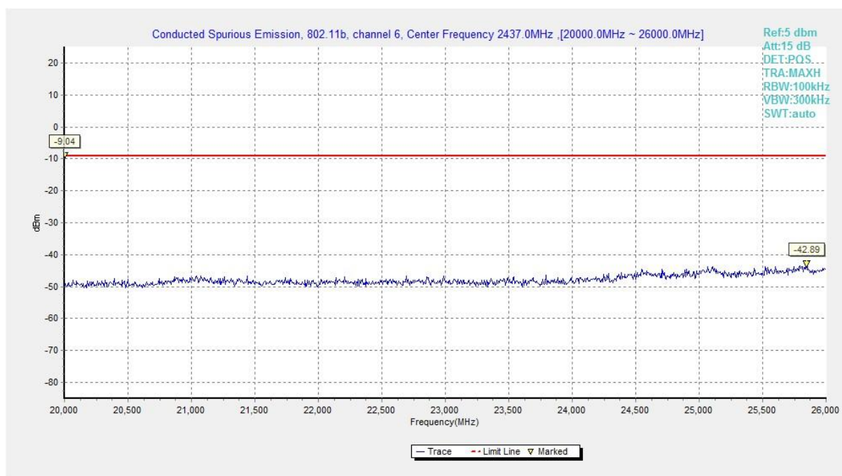
Fig.A.6.1.16 Conducted Spurious Emission (802.11b, Ch6, 20 GHz-26 GHz)
