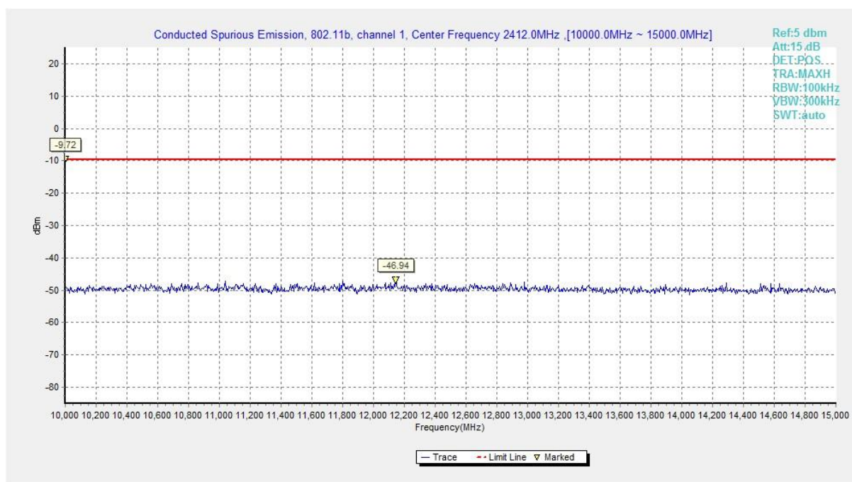
Fig.A.6.1.6 Conducted Spurious Emission (802.11b, Ch1, 10 GHz-15 GHz)
