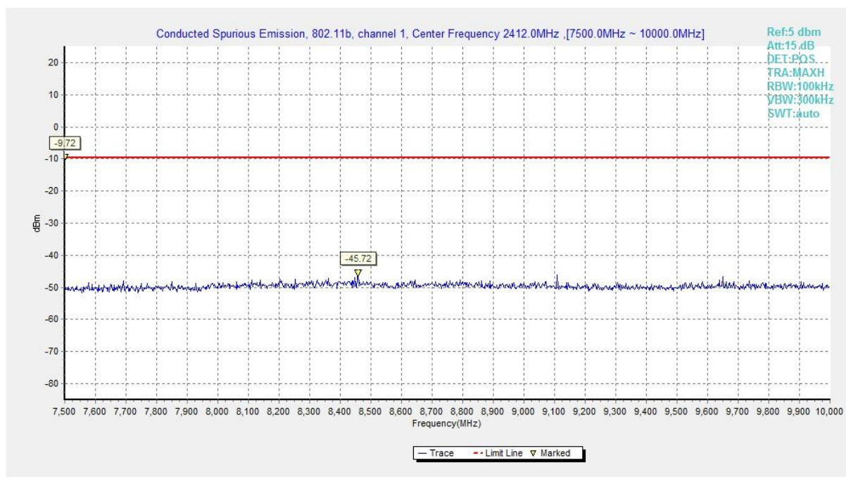
Fig.A.6.1.5 Conducted Spurious Emission (802.11b, Ch1, 7.5 GHz-10 GHz)
