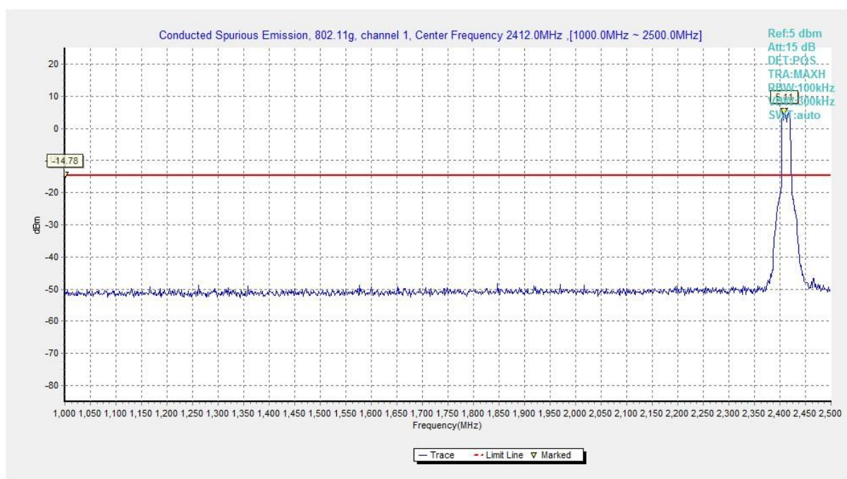
Fig.A.6.1.27 Conducted Spurious Emission (802.11g, Ch1, 1 GHz-2.5 GHz)
