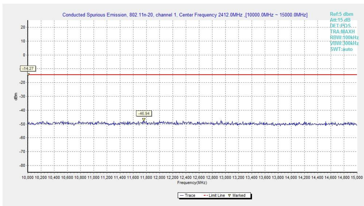
Fig.A.6.1.54 Conducted Spurious Emission (802.11n-HT20, Ch1, 10 GHz-15 GHz)
