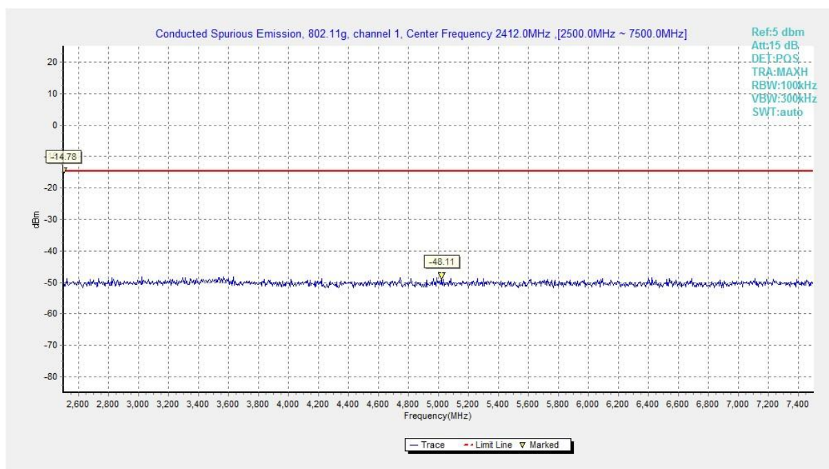
Fig.A.6.1.28 Conducted Spurious Emission (802.11g, Ch1, 2.5 GHz-7.5 GHz)
