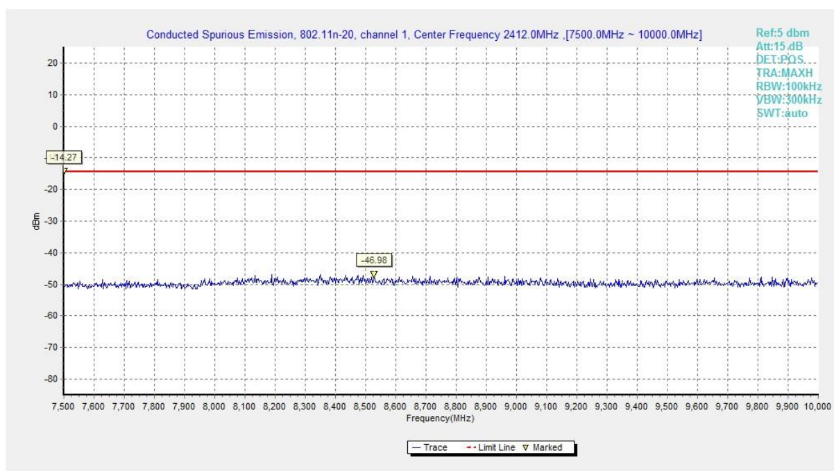
Fig.A.6.1.53 Conducted Spurious Emission (802.11n-HT20, Ch1, 7.5 GHz-10 GHz)
