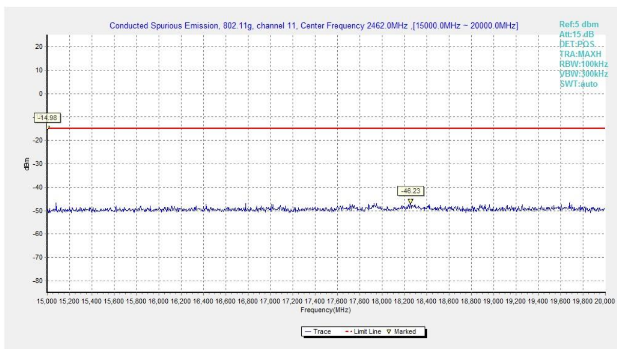
Fig.A.6.1.47 Conducted Spurious Emission (802.11g, Ch11, 15 GHz-20 GHz)
