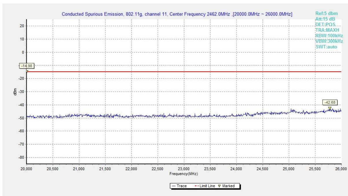
Fig.A.6.1.48 Conducted Spurious Emission (802.11g, Ch11, 20 GHz-26 GHz)
