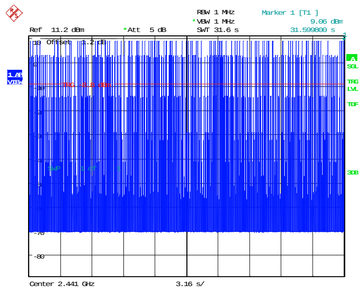
Fig.102. Time of occupancy (Dwell Time): Channel 39, 8DPSK -DH3
