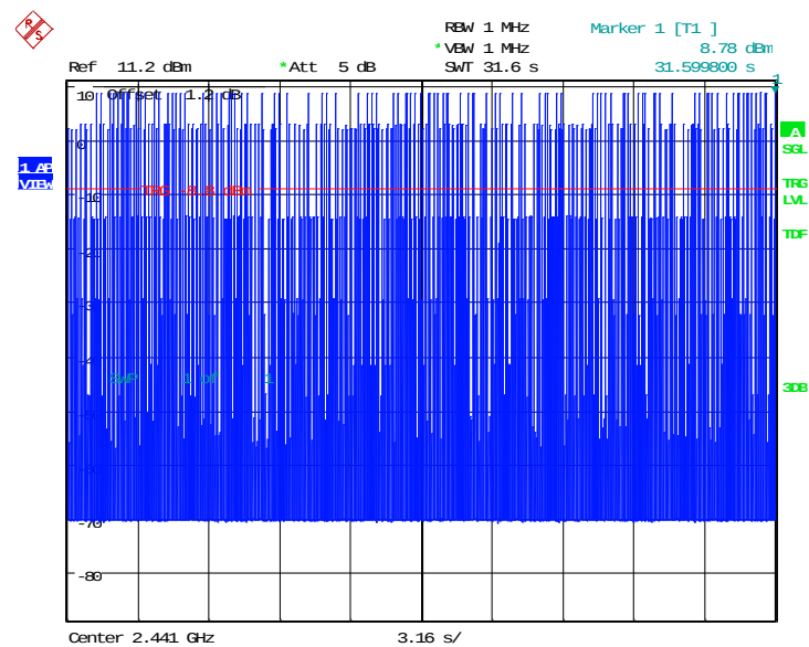
Fig.96. Time of occupancy (Dwell Time): Channel 39, \pi/4 DQPSK -DH3
