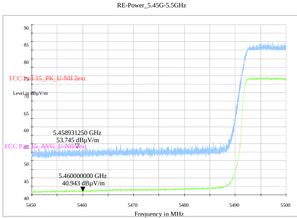
Fig. 49 Band Edges (802.11n-HT40, 5510MHz)
