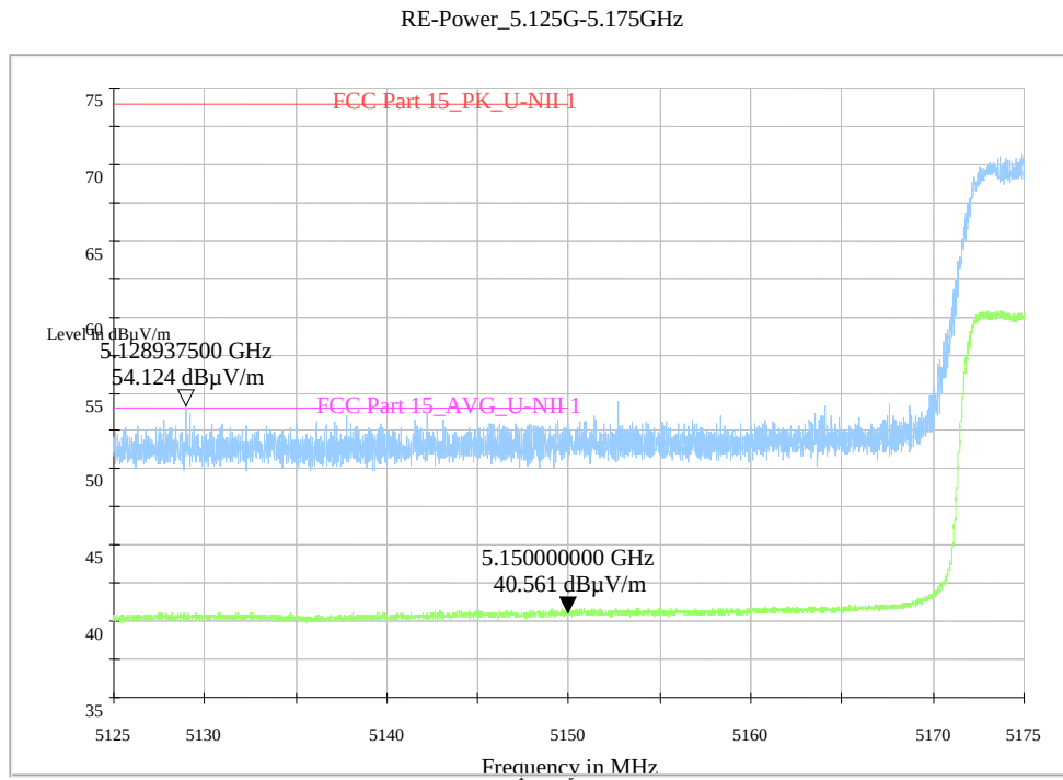
Fig. 50 Band Edges (802.11ac-HT80, 5210MHz)
