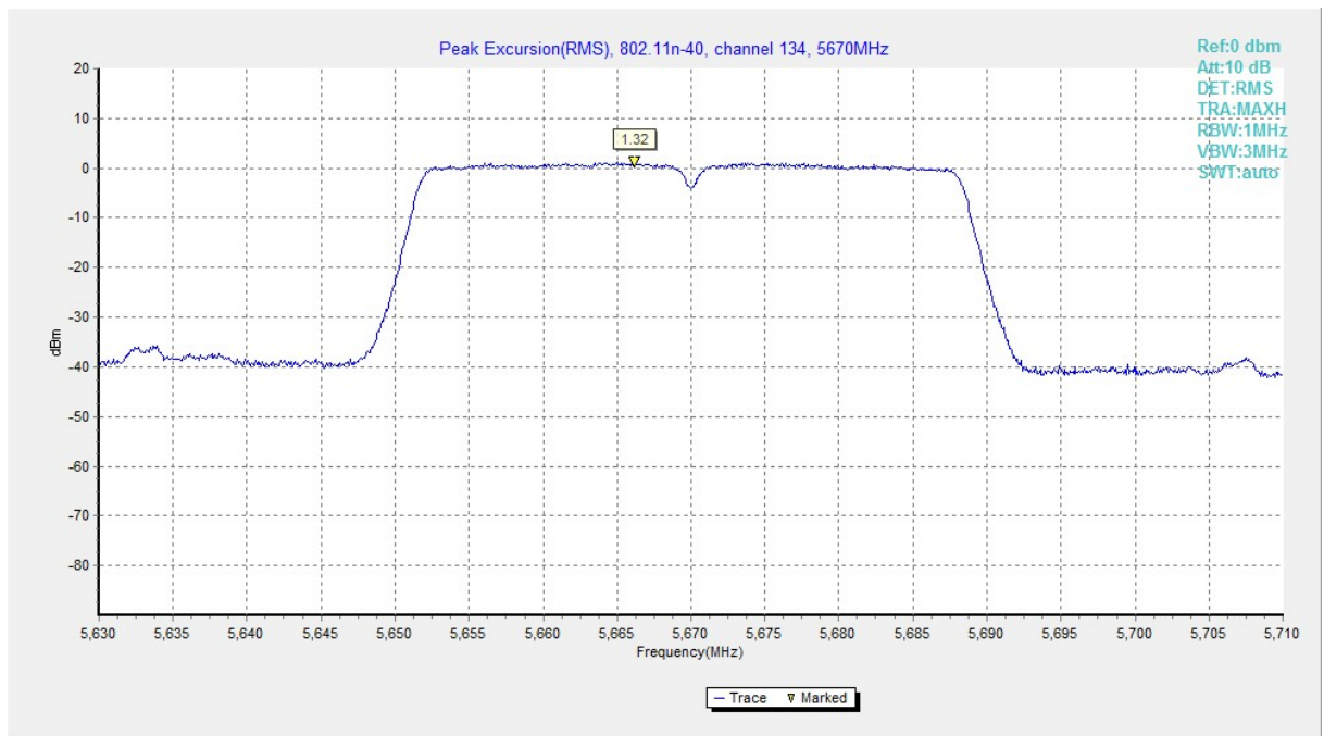
Fig. 189 Peak Excursions (802.11n-HT40, ch134, average)
