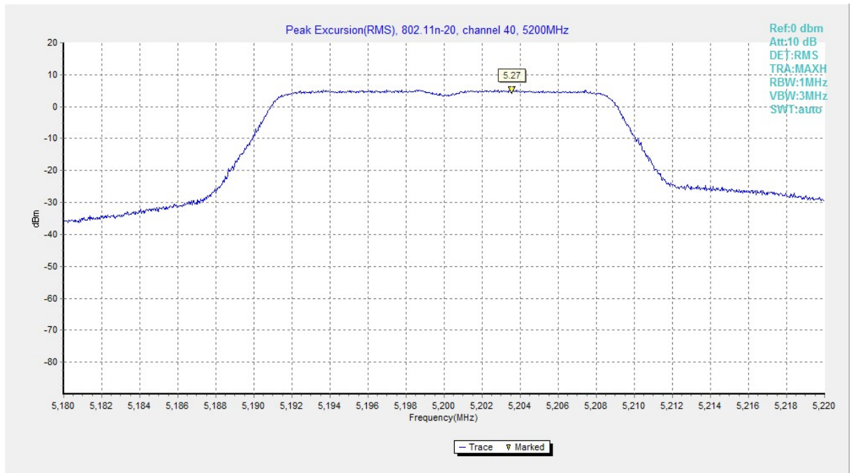
Fig. 162 Peak Excursions (802.11n-HT20, ch40, average)
