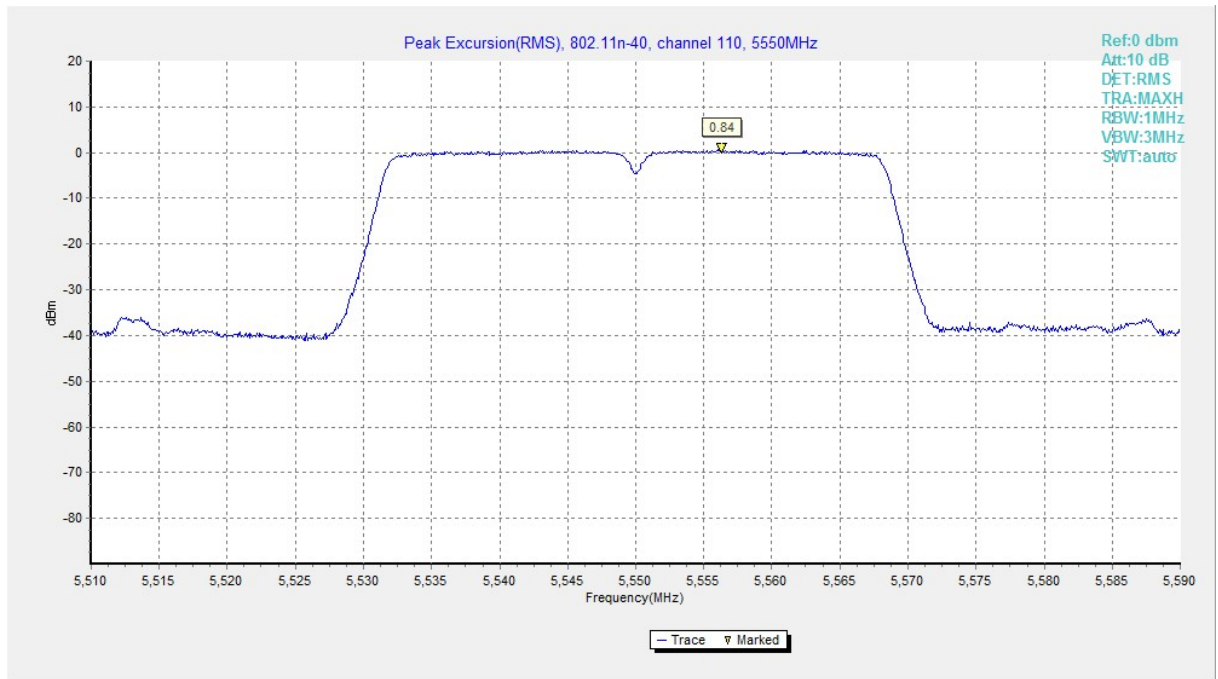
Fig. 188 Peak Excursions (802.11n-HT40, ch110, average)
