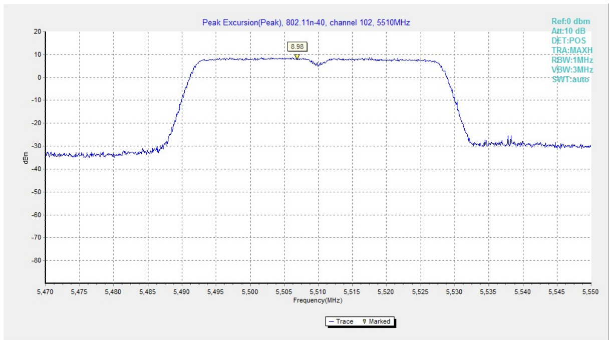
Fig. 184 Peak Excursions (802.11n-HT40, ch102, peak)
