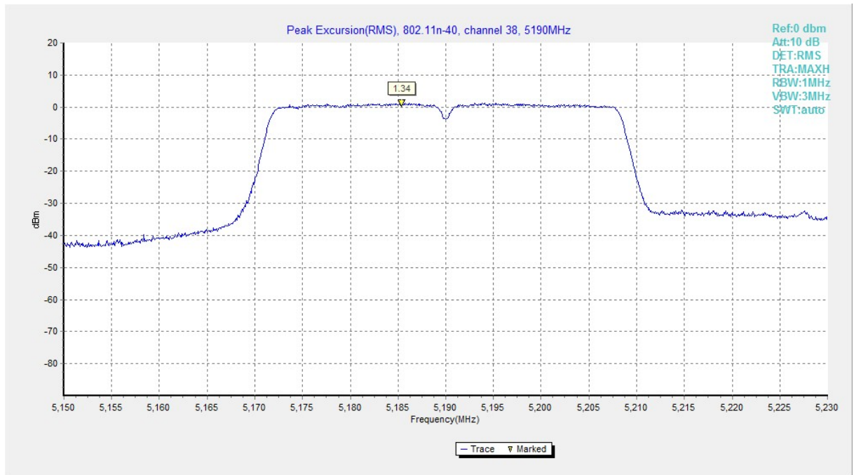
Fig. 180 Peak Excursions (802.11n-HT40, ch38, average)
