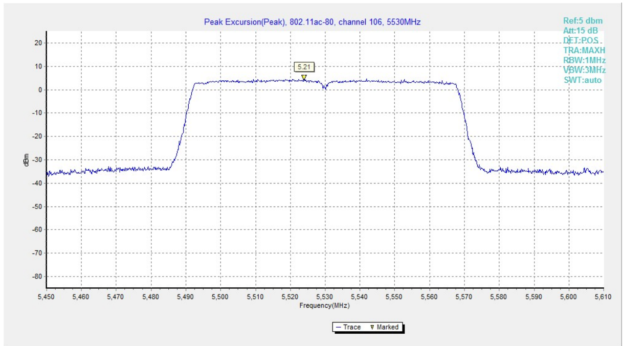
Fig. 192 Peak Excursions (802.11ac-HT80, ch106, peak)
