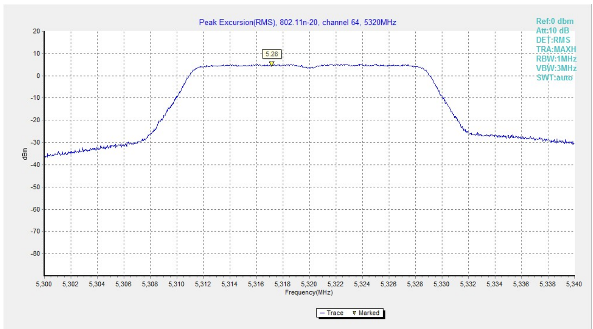
Fig. 169 Peak Excursions (802.11n-HT20, ch64, average)
