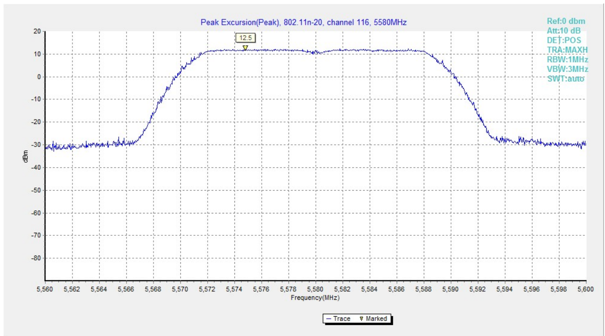
Fig. 171 Peak Excursions (802.11n-HT20, ch116, peak)
