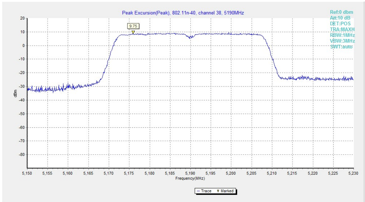
Fig. 176 Peak Excursions (802.11n-HT40, ch38, peak)
