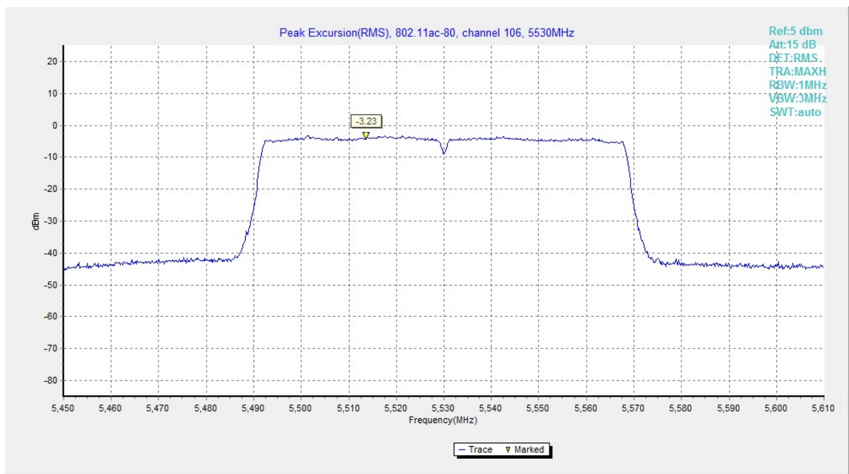
Fig. 195 Peak Excursions (802.11ac-HT80, ch106, average)
