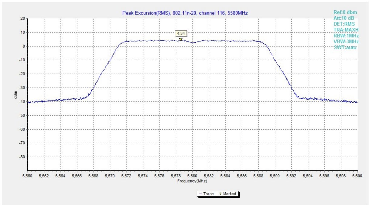
Fig. 174 Peak Excursions (802.11n-HT20, ch116, average)
