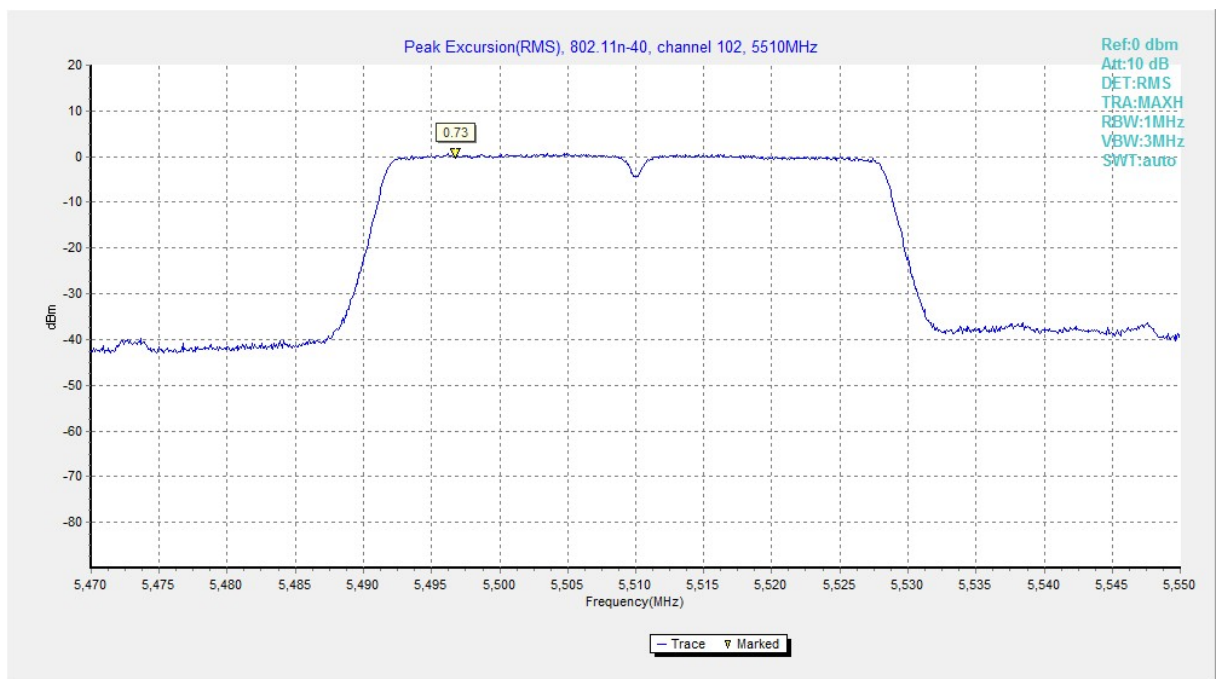
Fig. 187 Peak Excursions (802.11n-HT40, ch102, average)
