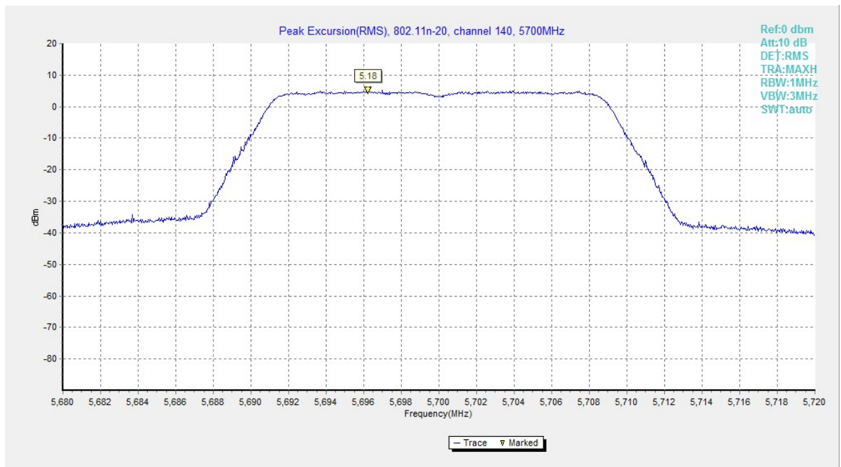
Fig. 175 Peak Excursions (802.11n-HT20, ch140, average)
