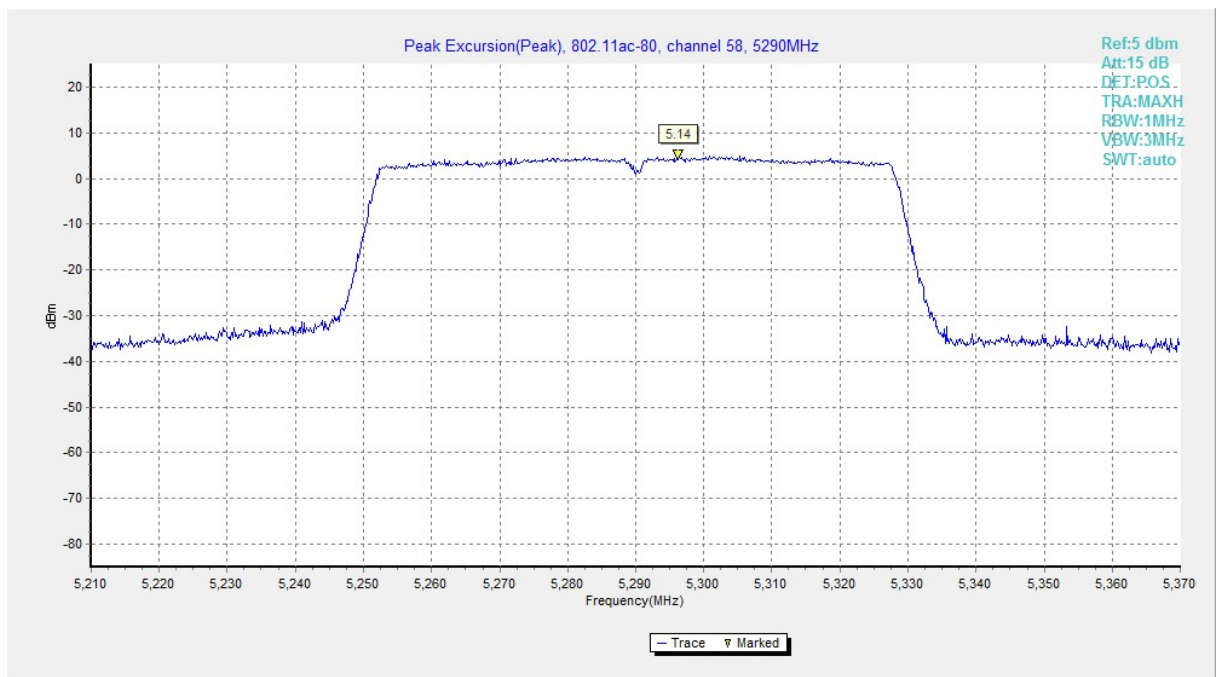
Fig. 191 Peak Excursions (802.11ac-HT80, ch58, peak)
