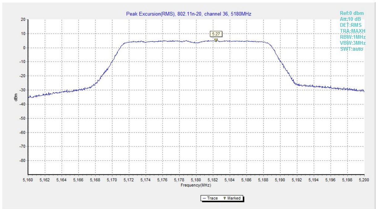
Fig. 161 Peak Excursions (802.11n-HT20, ch36, average)
