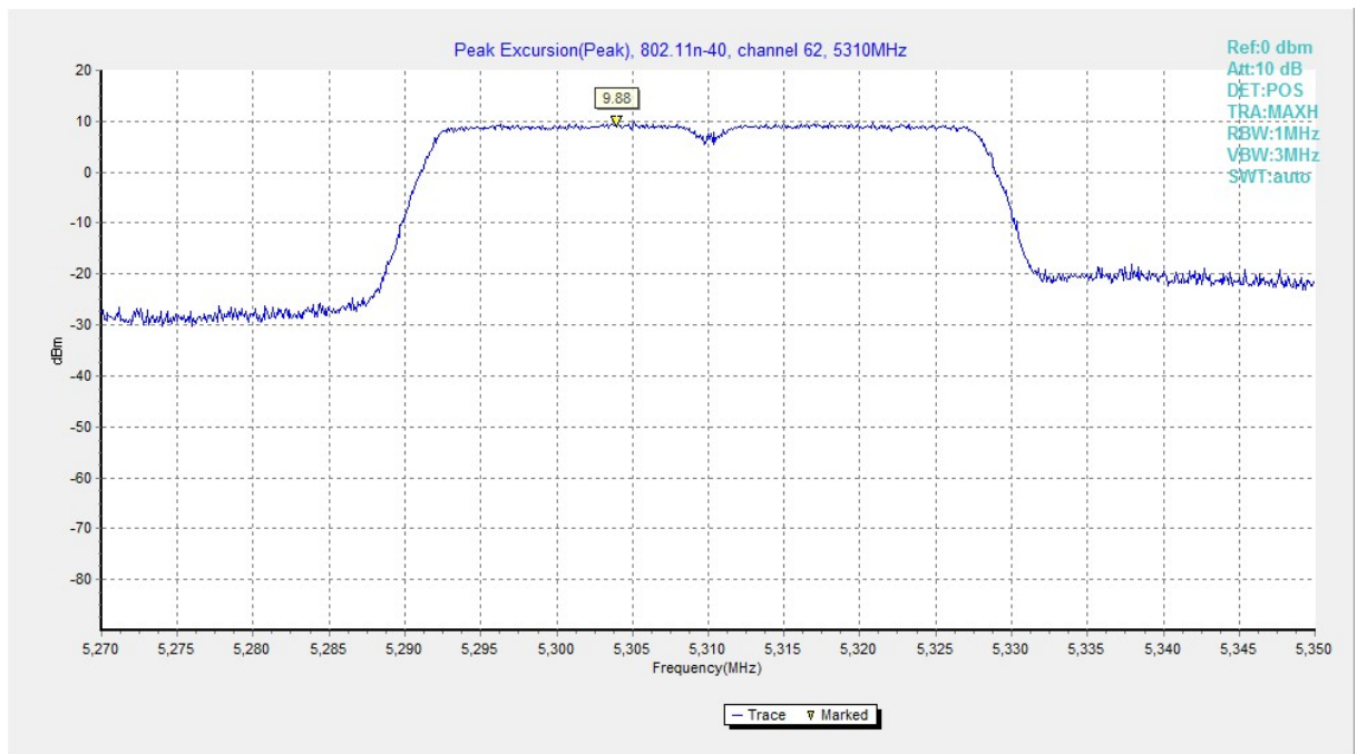
Fig. 179 Peak Excursions (802.11n-HT40, ch62, peak)
