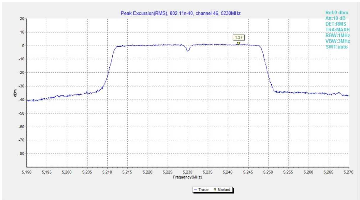
Fig. 181 Peak Excursions (802.11n-HT40, ch46, average)
