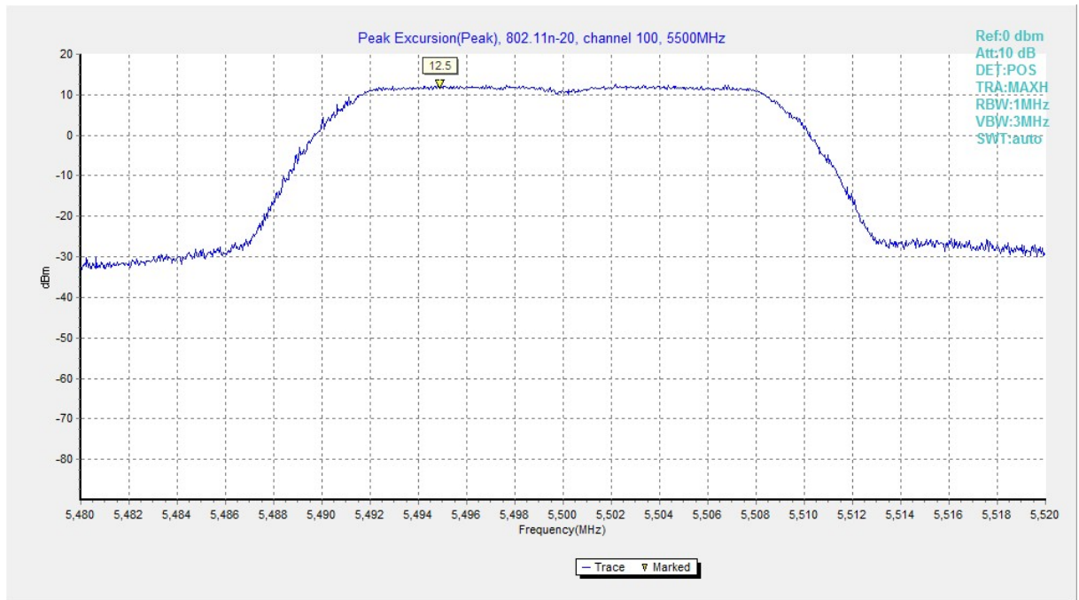
Fig. 170 Peak Excursions (802.11n-HT20, ch100, peak)
