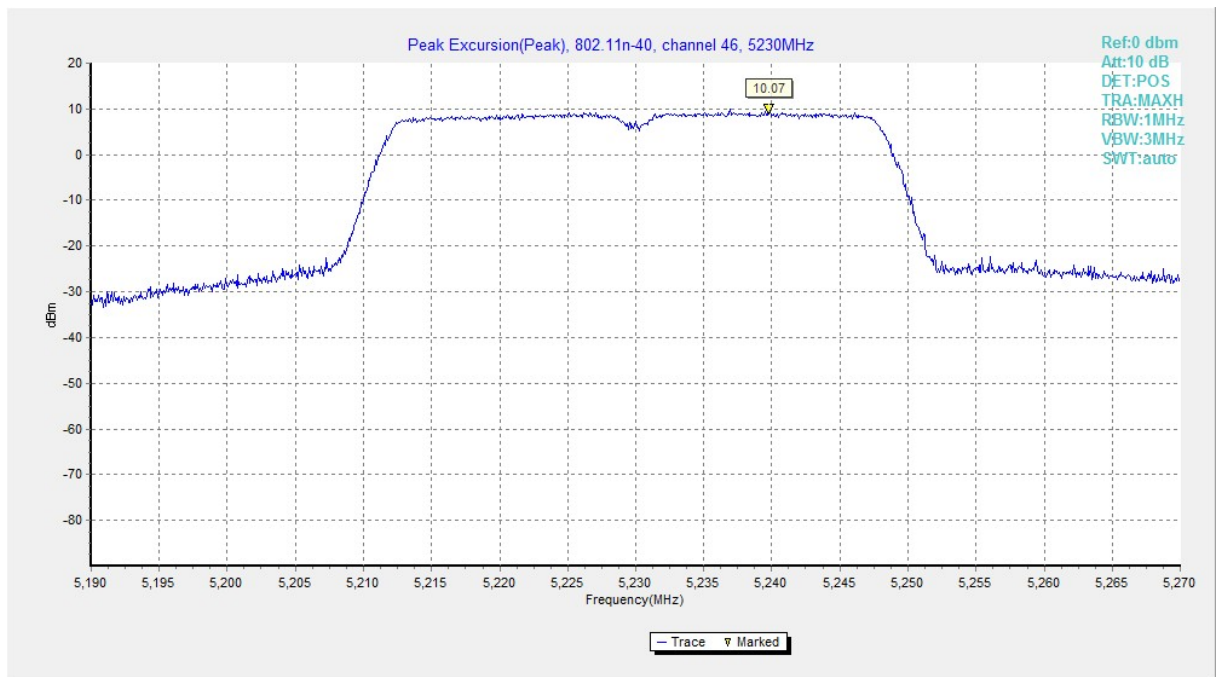
Fig. 177 Peak Excursions (802.11n-HT40, ch46, peak)
