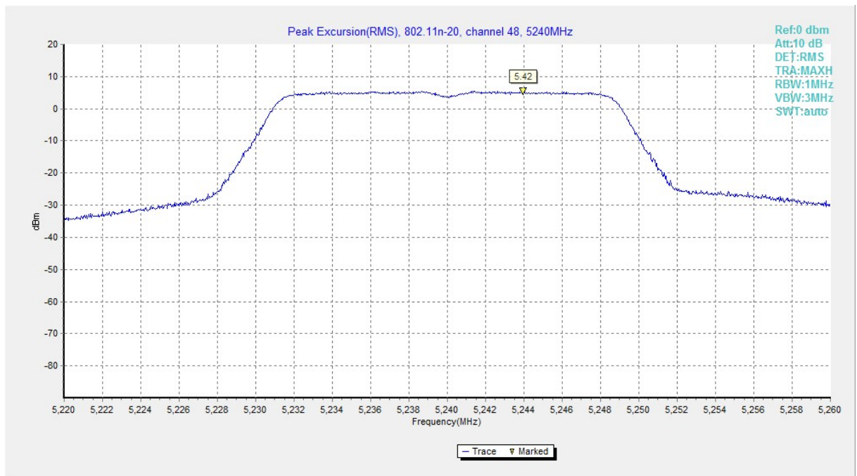
Fig. 163 Peak Excursions (802.11n-HT20, ch48, average)
