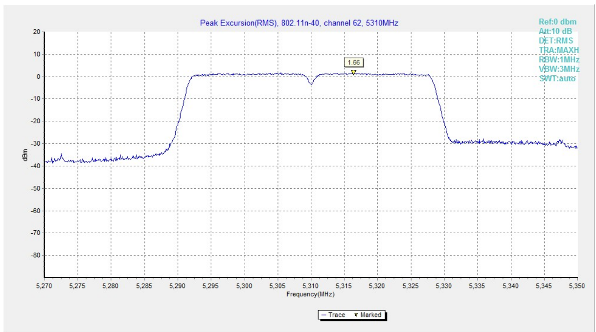
Fig. 183 Peak Excursions (802.11n-HT40, ch62, average)
