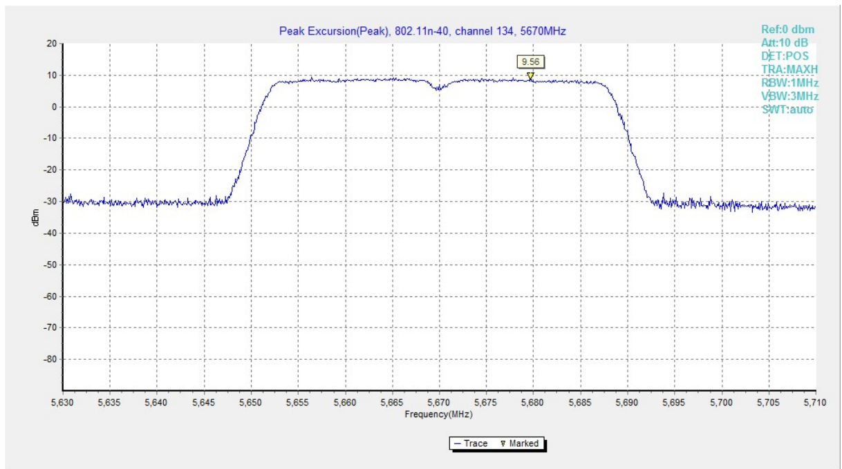
Fig. 186 Peak Excursions (802.11n-HT40, ch134, peak)
