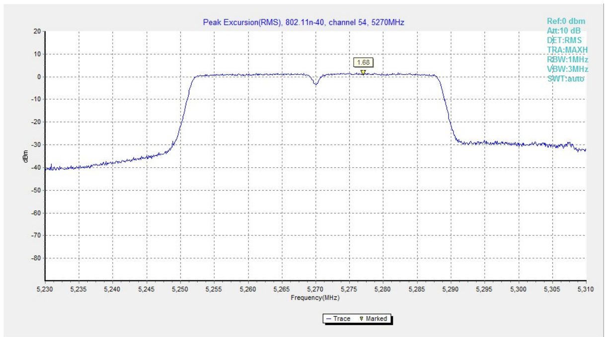
Fig. 182 Peak Excursions (802.11n-HT40, ch54, average)
