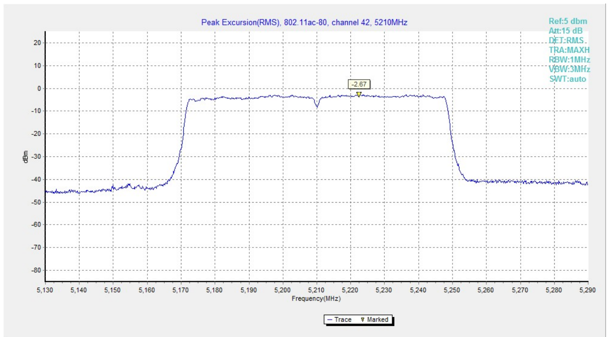
Fig. 193 Peak Excursions (802.11ac-HT80, ch42, average)
