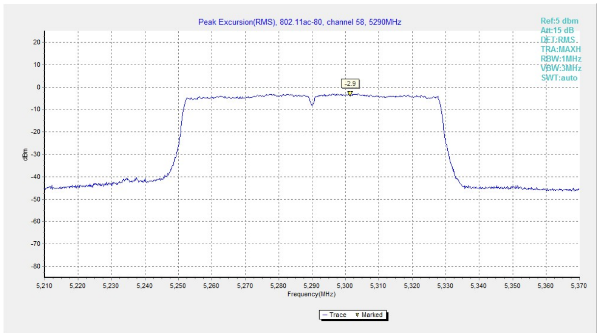
Fig. 194 Peak Excursions (802.11ac-HT80, ch58, average)
