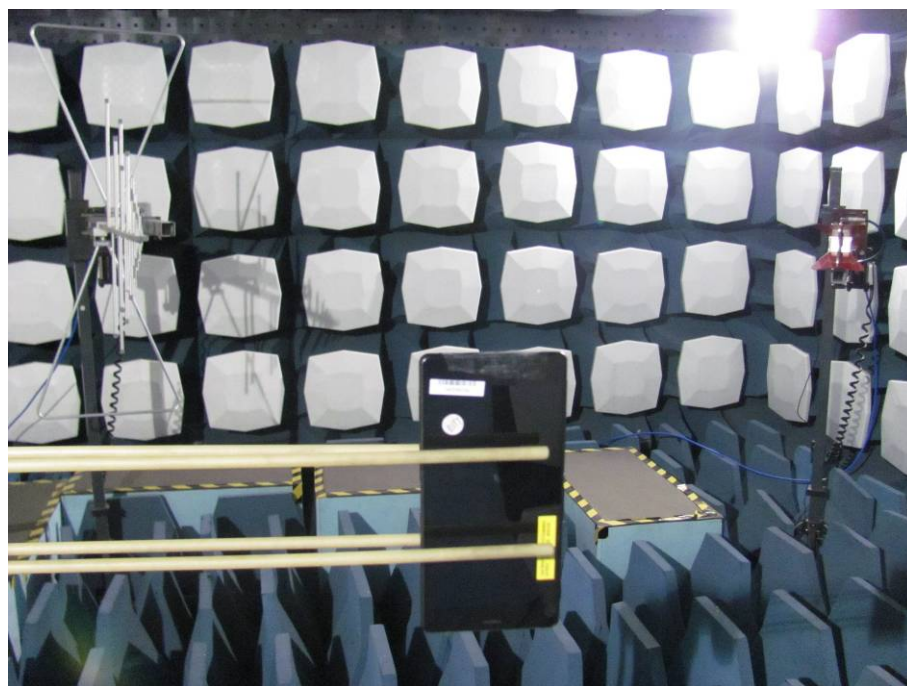
Picture C-4: Radiated spurious emission (PART22/24/27)
