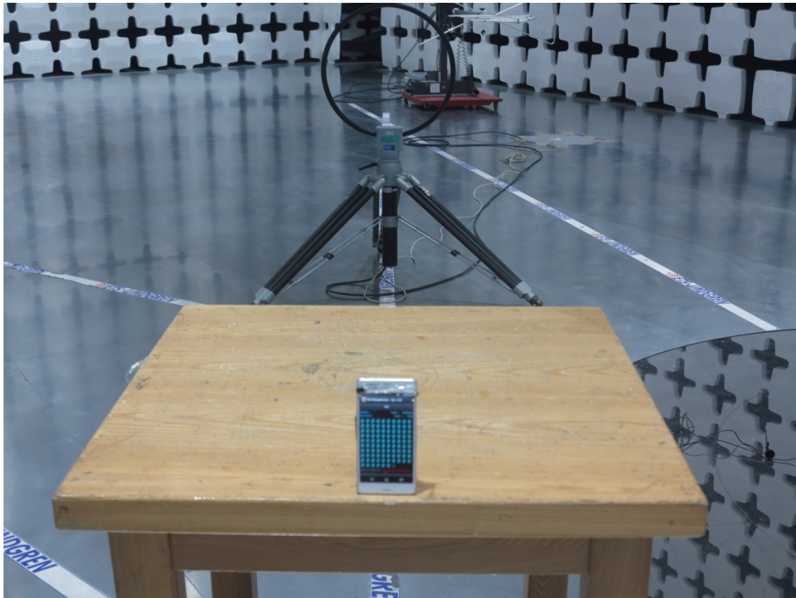
Picture C-1: Field Strength Measurements (Below 30MHz) (PART15C)
