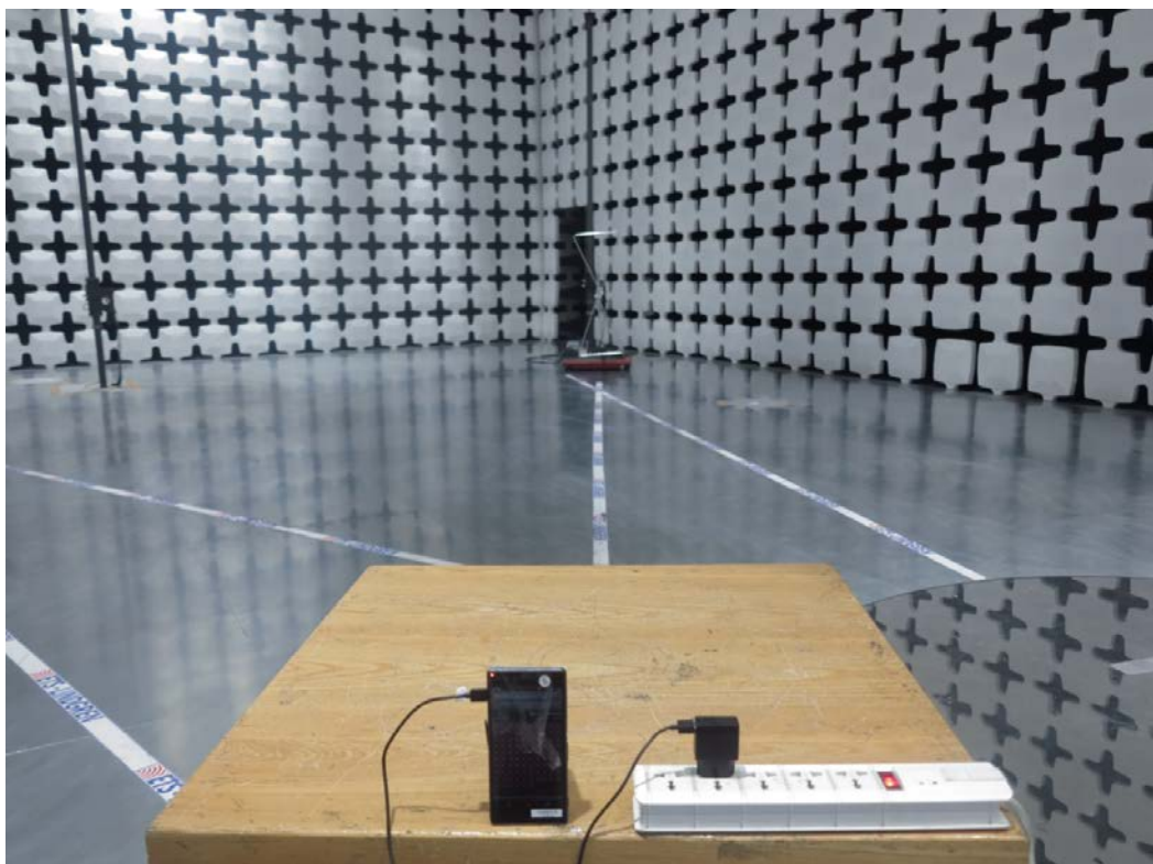
Picture C-2: Field Strength Measurements (Above 30MHz) (PART15C)
