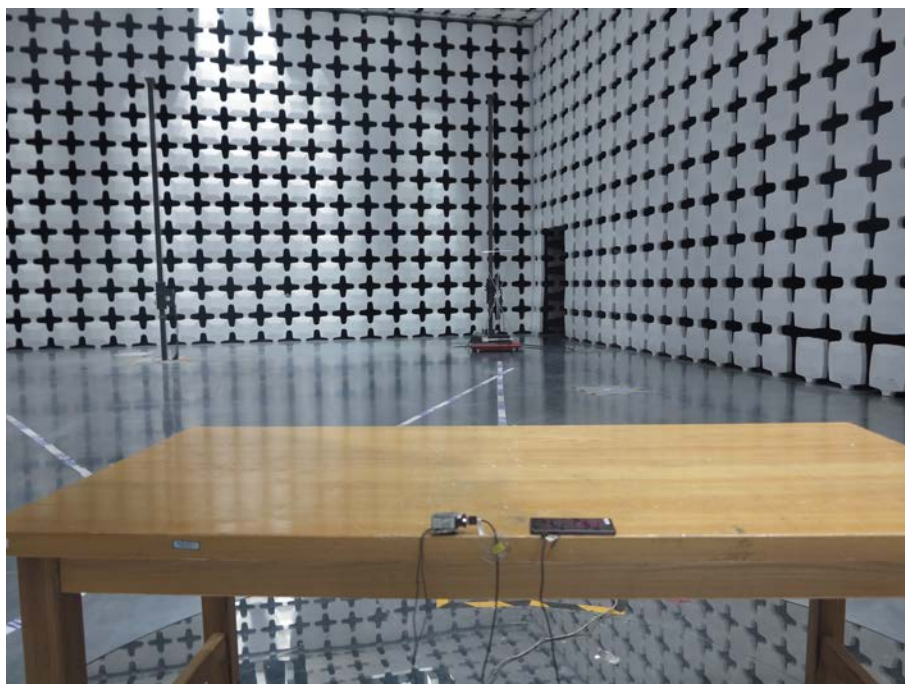
Picture C-6: Radiated emission (PART15B)
