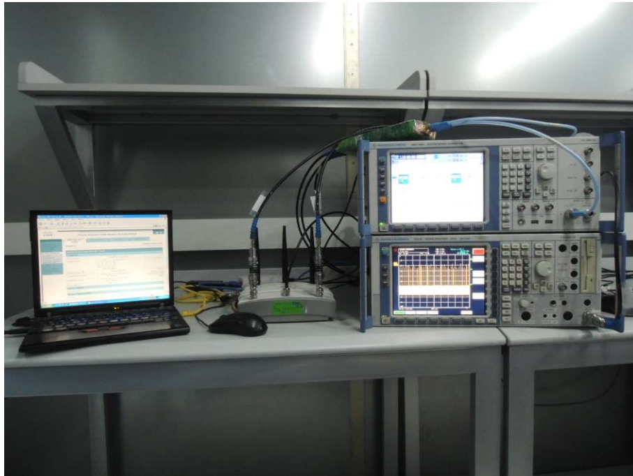
Picture C-13: Conducted test(PART15C)
