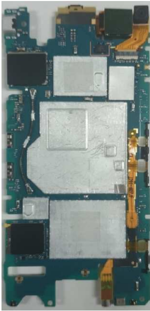
Internal PWB with Shield cases (Front-side)
