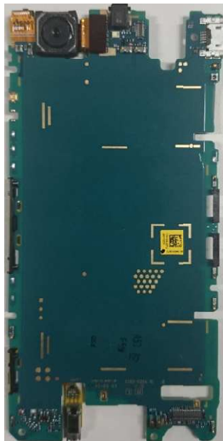
Internal PWB with Shield cases (Rear-side)
