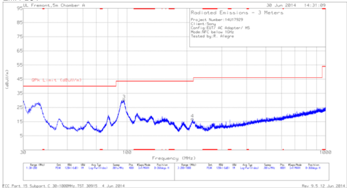
EMI PLOT
