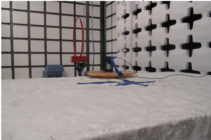
RADIATED EMISSIONS BELOW 30MHz (BACK)
