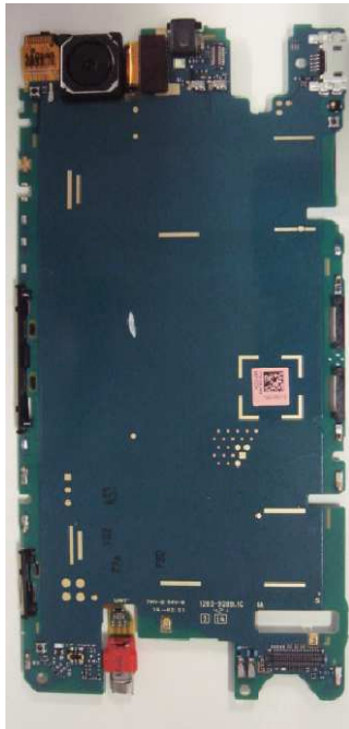
Internal PWB with Shield cases (Rear-side)
