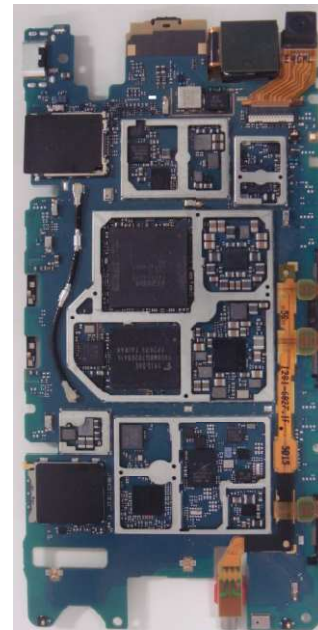
Internal PWB without Shield cases (Front-side)
