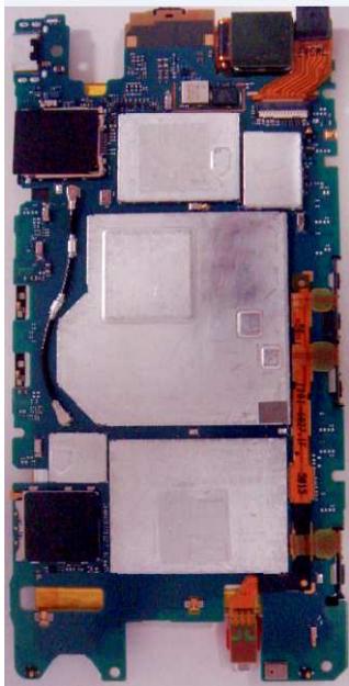
Internal PWB with Shield cases (Front-side)
