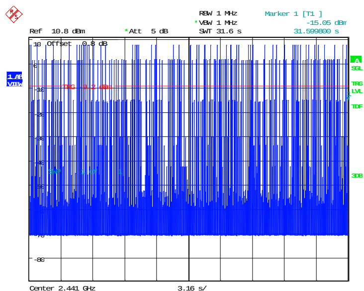
Fig.98. Time of occupancy (Dwell Time): Channel 39, \pi/4 DQPSK -DH5
