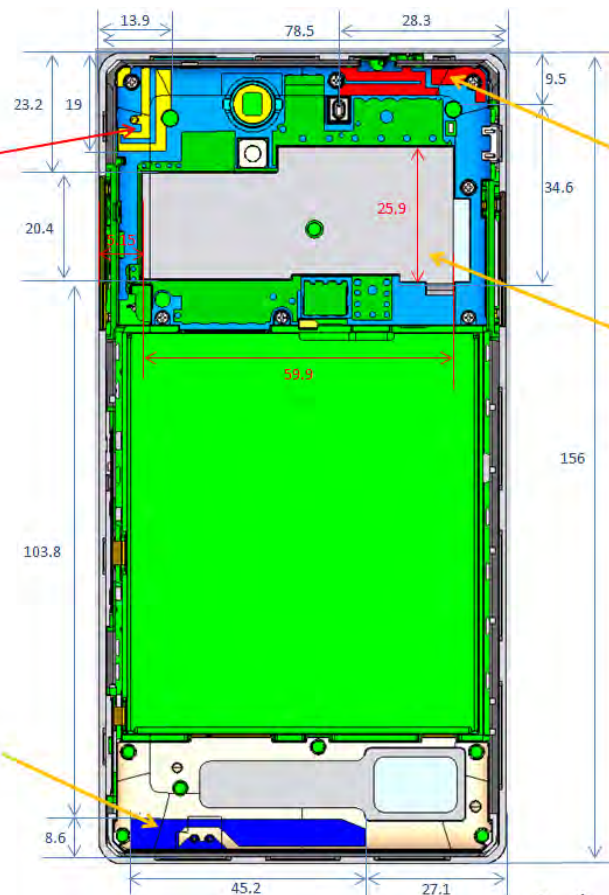
Antenna positioning diagram with separation distance
