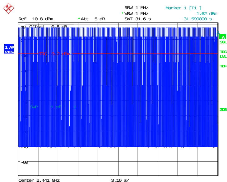
Fig.94. Time of occupancy (Dwell Time): Channel 39, \pi/4 DQPSK -DH1
