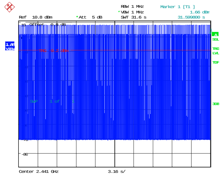
Fig.100. Time of occupancy (Dwell Time): Channel 39, 8DPSK-DH1
