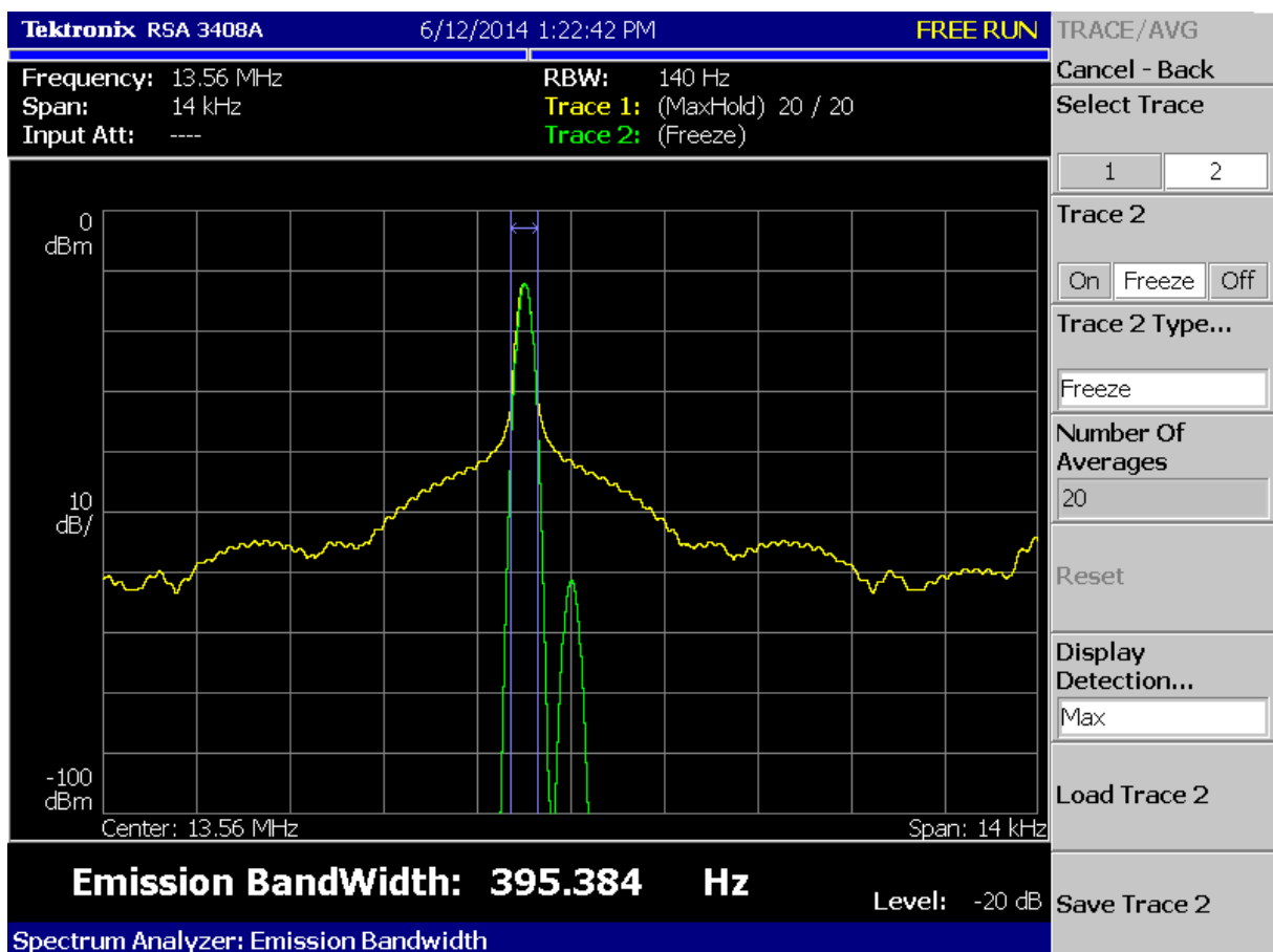
Figure A-5: Test result of EUT1 at test set. NFC02
