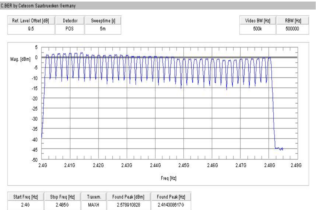
Plot 1: Number of hopping channels
