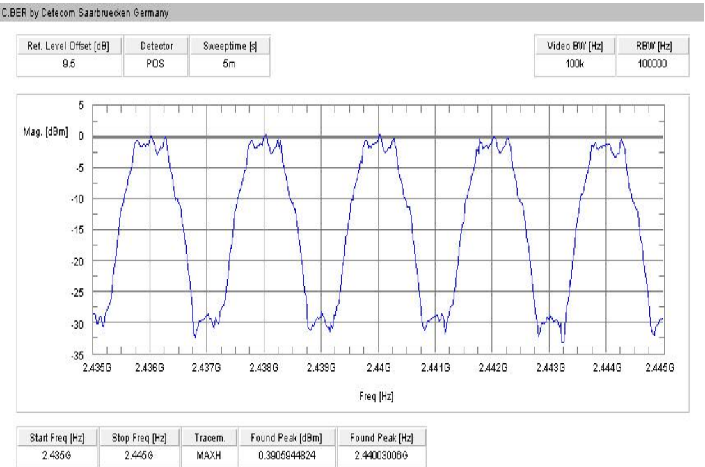
Plot 1: Carrier Frequency Separation
