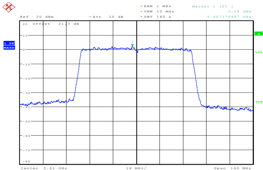
Plot 4: 5610 MHz
