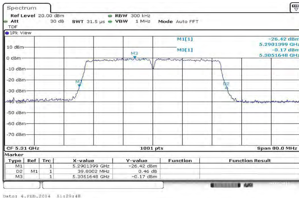
Plot 4: 5310 MHz
