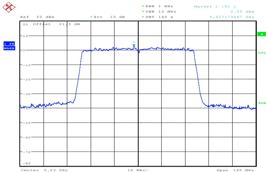
Plot 3: 5530 MHz
