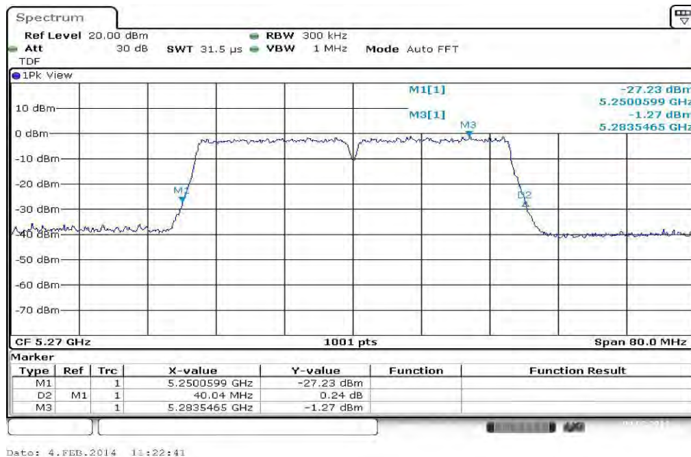
Plot 3: 5270 MHz
