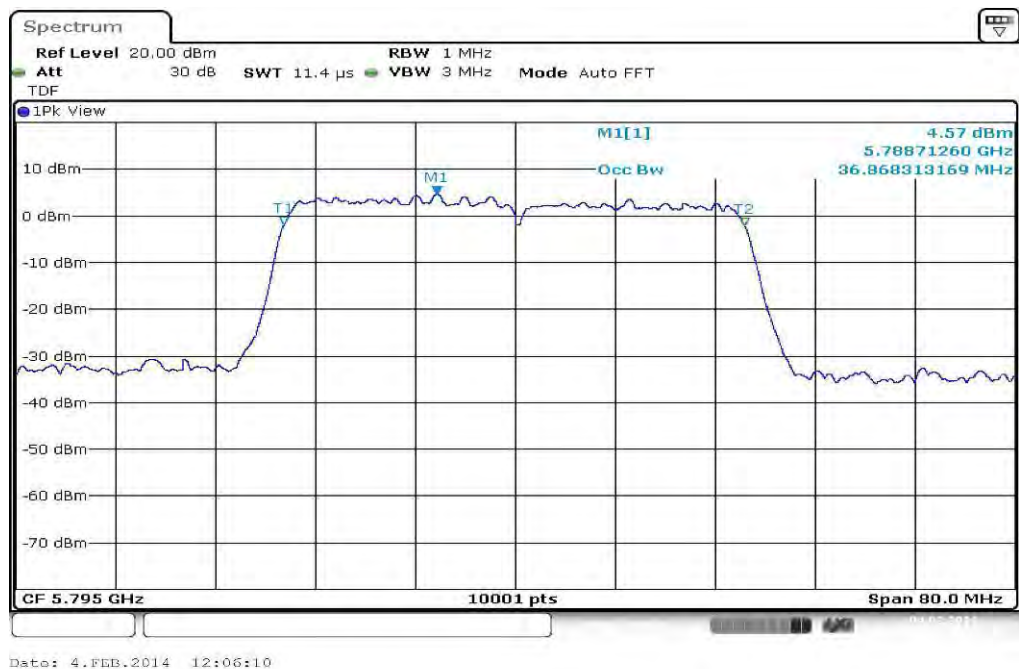
Plot 2: TX mode, highest channel
