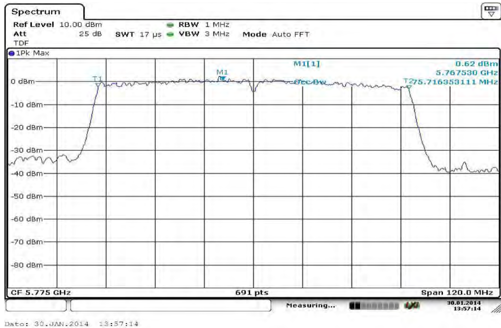
Plot 1: TX mode, mid channel
