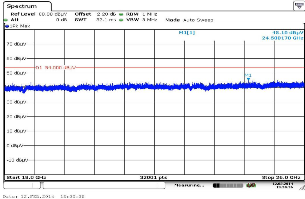
Plot 14: 18 GHz to 26 GHz, 5530 MHz, vertical & horizontal polarization
