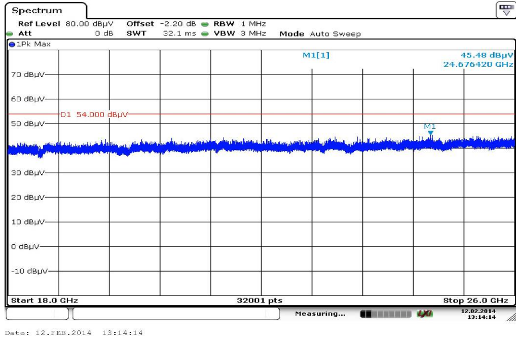
Plot 29: 18 GHz to 26 GHz, 5670 MHz, vertical & horizontal polarization
