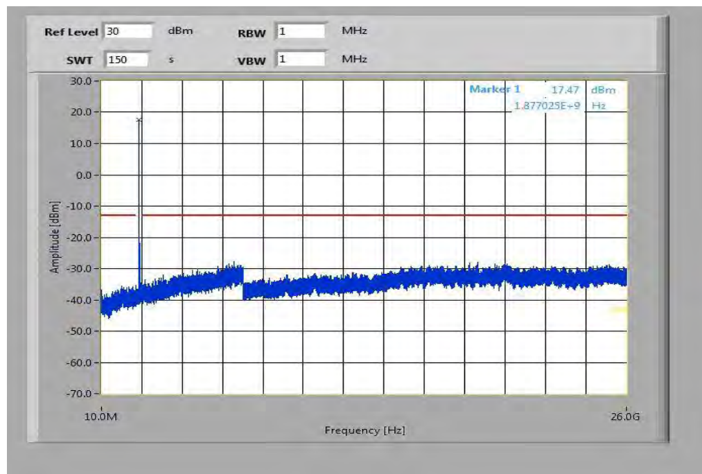
Plot 2: Middle Channel (10 MHz - 26 GHz)
