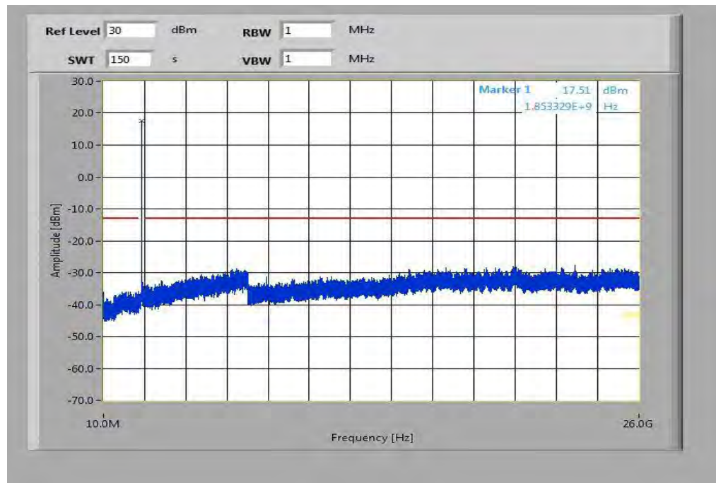
Plot 1: Lowest Channel (10 MHz - 26 GHz)
