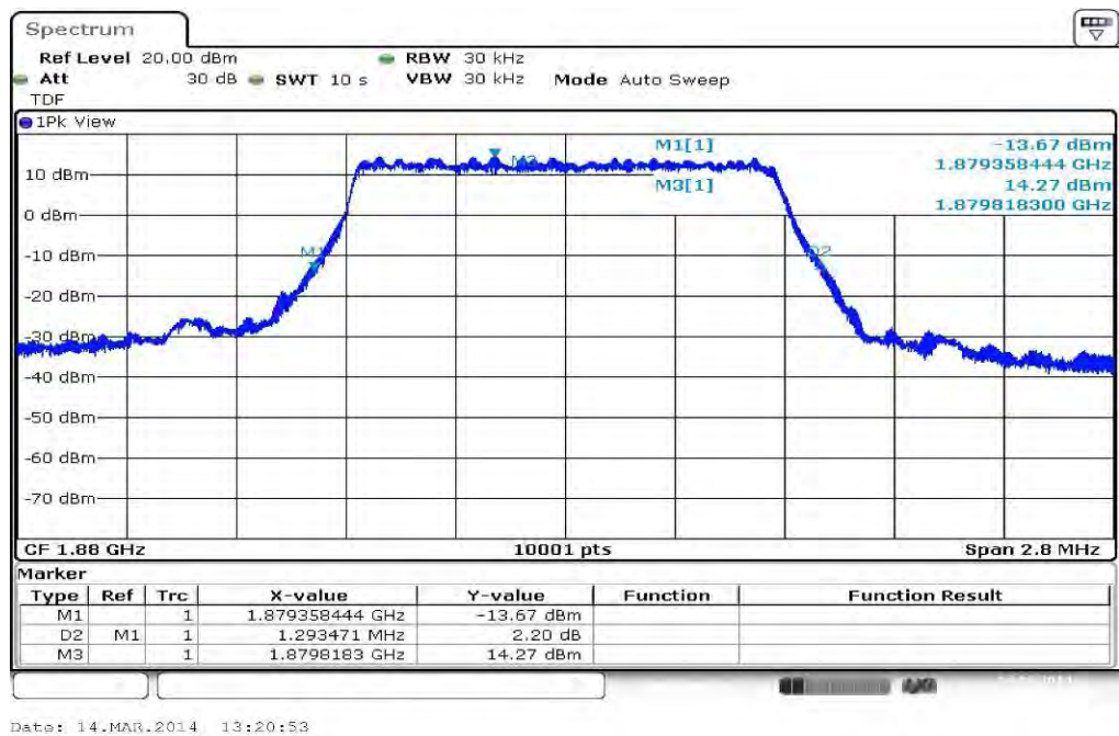
Plot 2: 1.4 MHz (-26 dBc BW)
