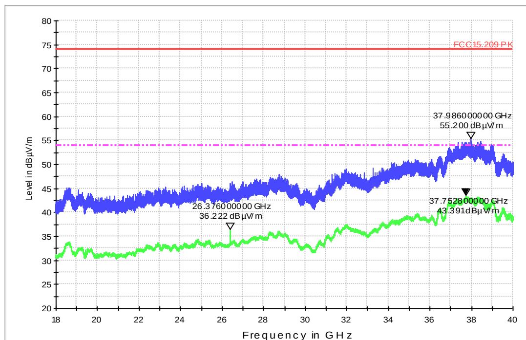
EMI Scan_18_40GHz_Pre_fast_500us
