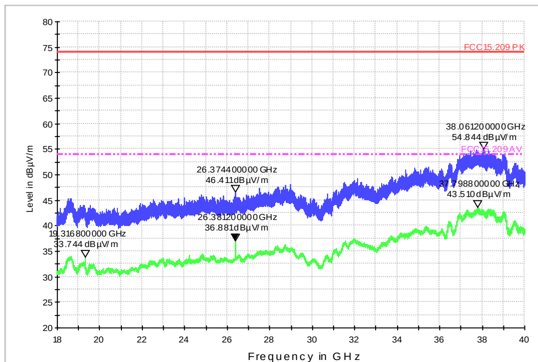
EMI Scan_18_40GHz_Pre_fast_500us
