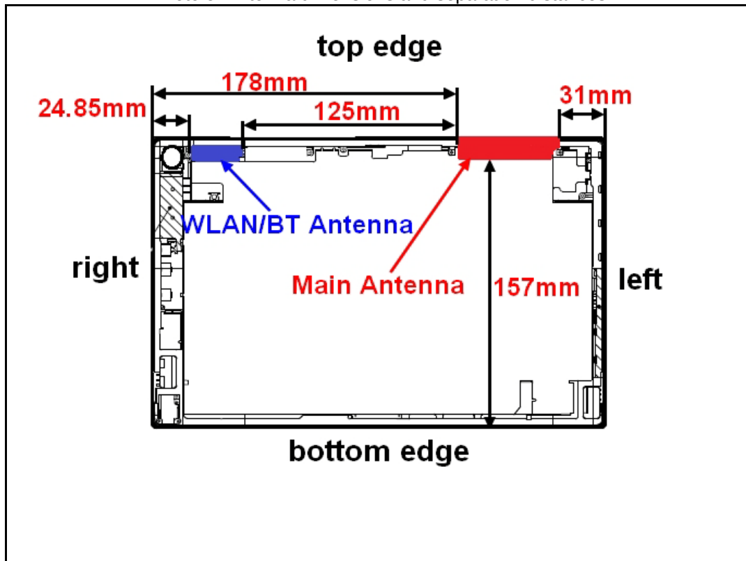
Photo 5: Antenna dimensions and separation distances
