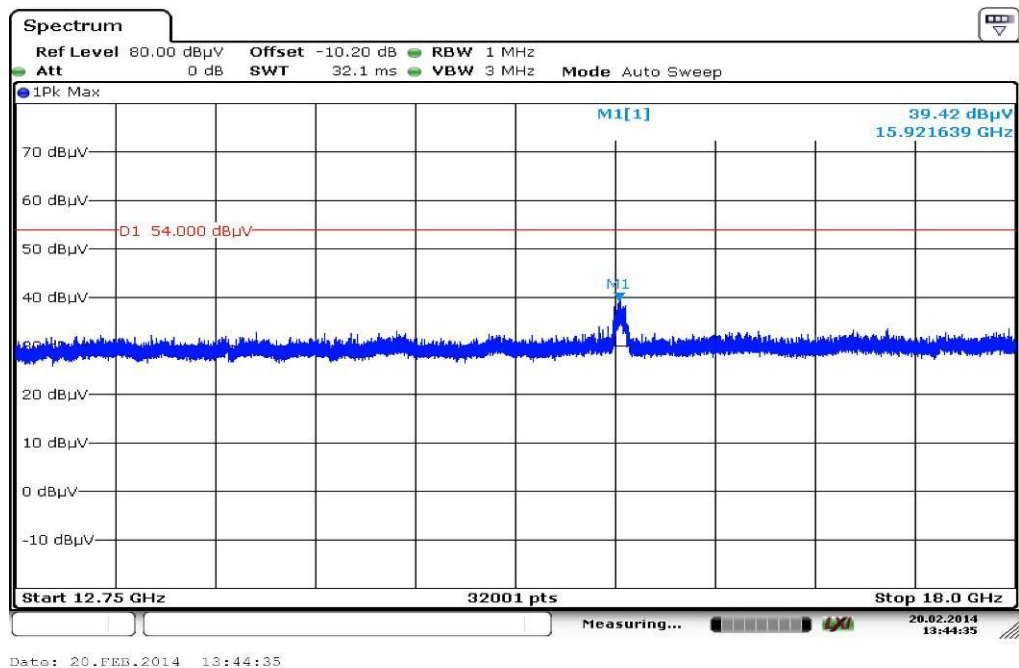
Plot 18: 12 GHz to 18 GHz, channel 62, vertical & horizontal polarization
