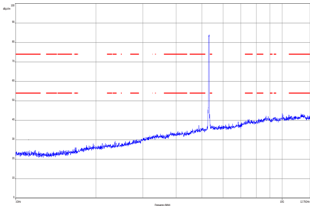
Plot 17: 1 GHz to 12.75 GHz, channel 62, vertical & horizontal polarization
