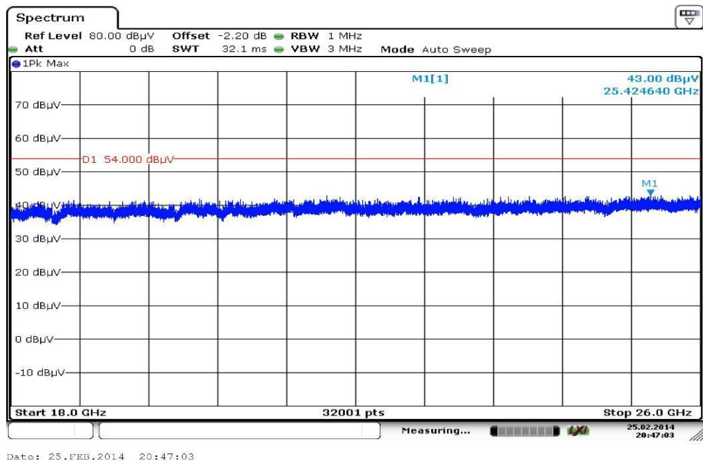
Plot 4: 18 GHz to 26 GHz, vertical &amp; horizontal polarization
