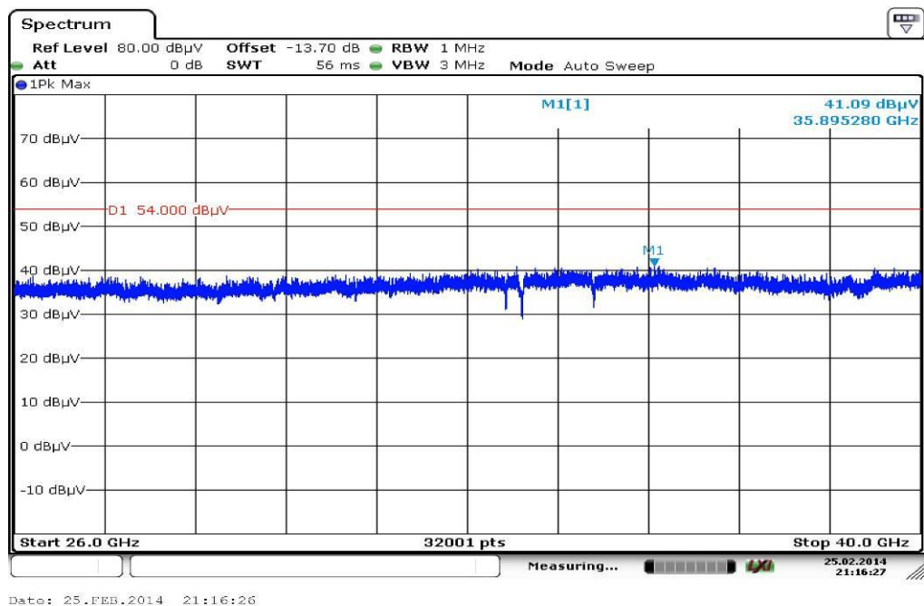
Plot 5: 26 GHz to 40 GHz, vertical &amp; horizontal polarization
