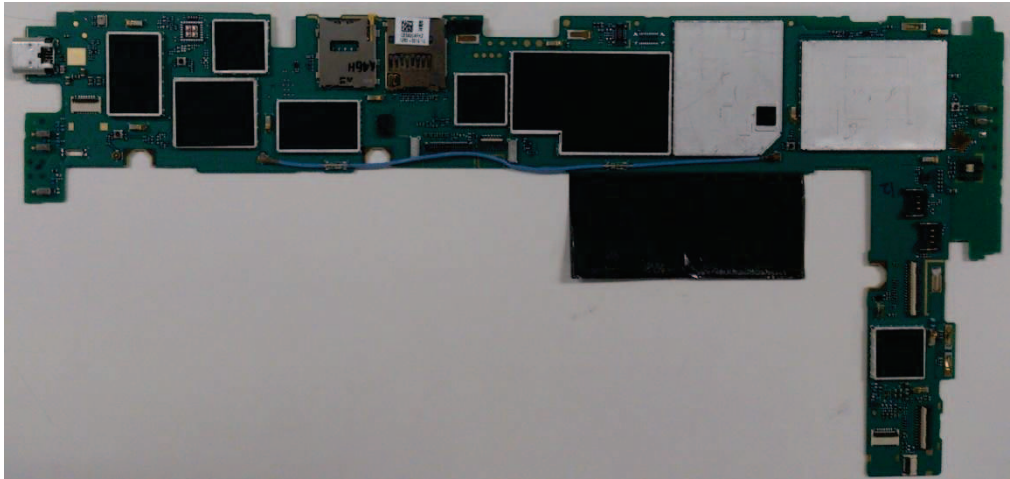
Internal PWB with Shield cases (Front-side)
