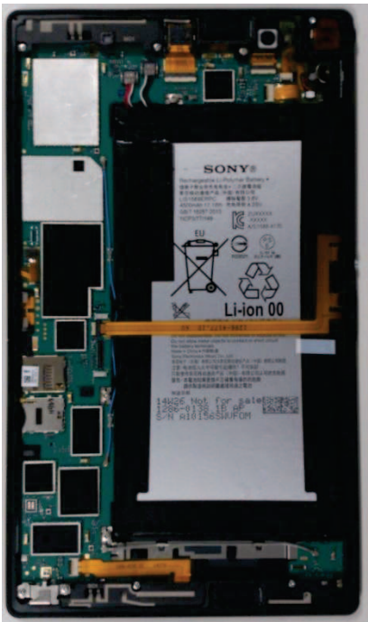
Without Rear Panel
