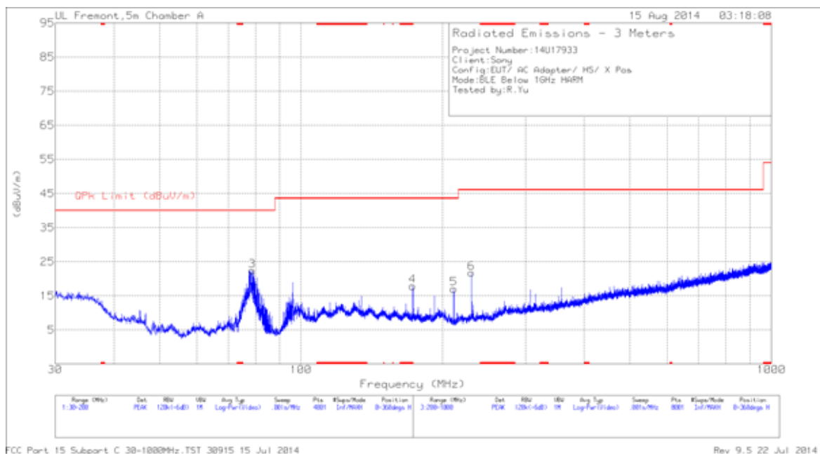
HORIZONTAL PLOT
