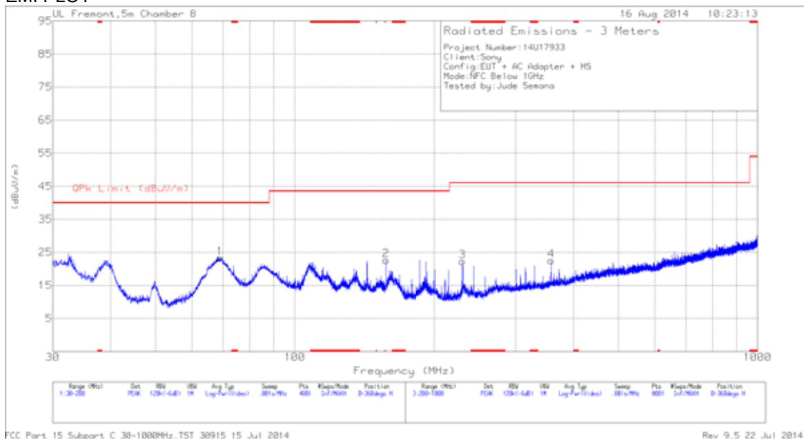
EMI PLOT
