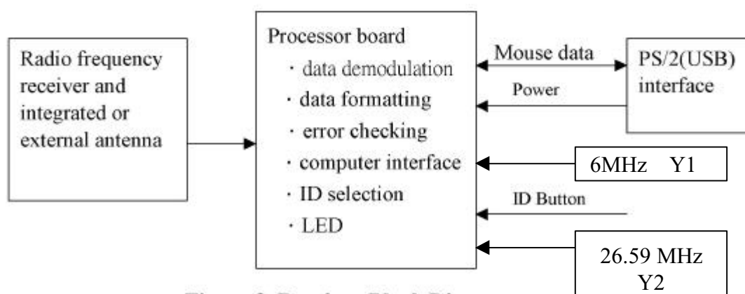
Figure 3. Receiver Block Diagram
