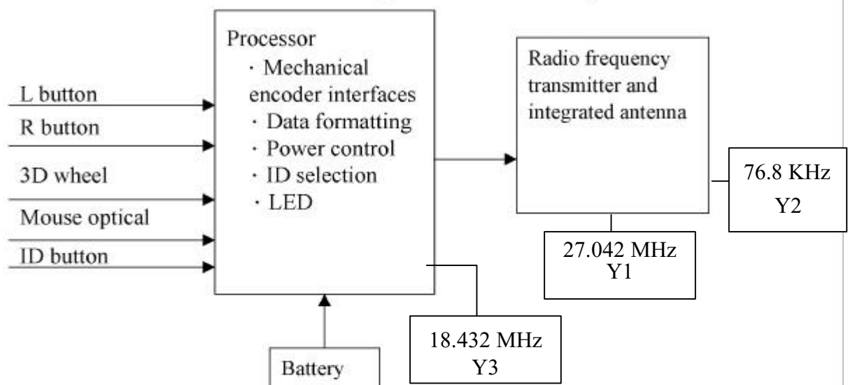
Figure 2. Mouse Unit Block Diagram
