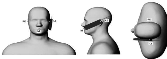
Fig. 5.1.1. Cheek/Touch position
