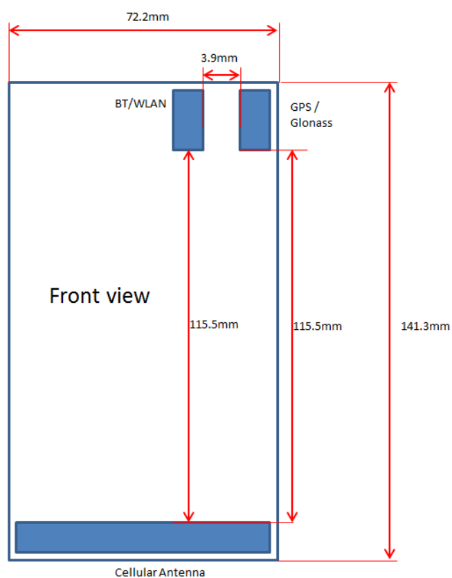
Photo 24: Antenna location
