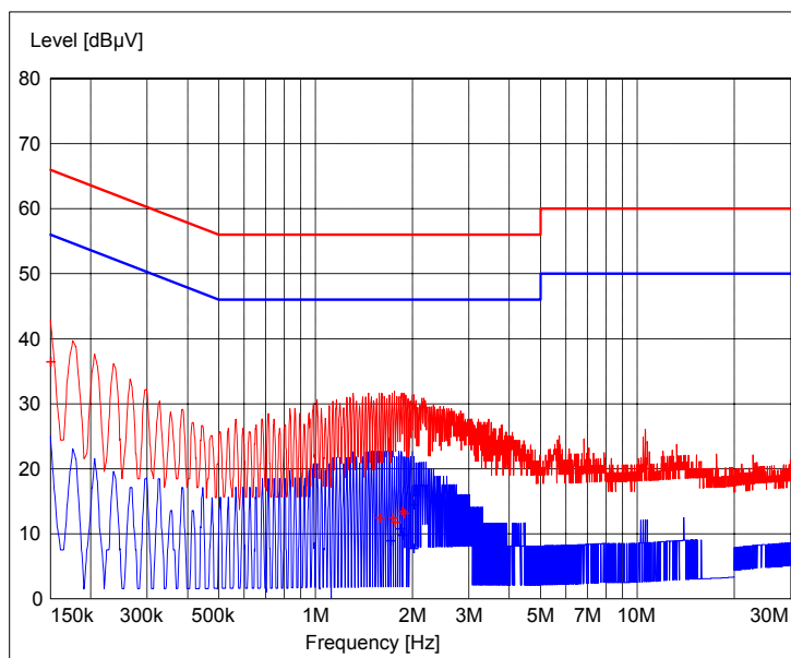
Picture 15. AC powerline emissions
