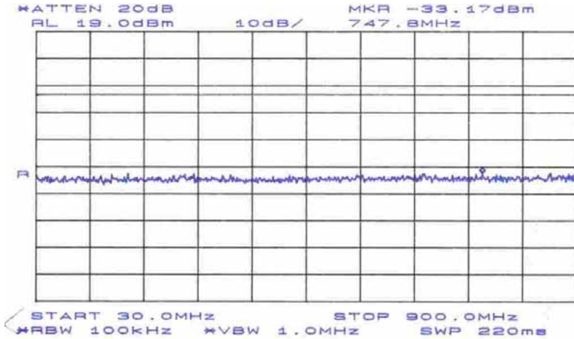
Figure 4-24. Low Power Conducted Spurious Emissions, High Channel 30 - 900MHz
