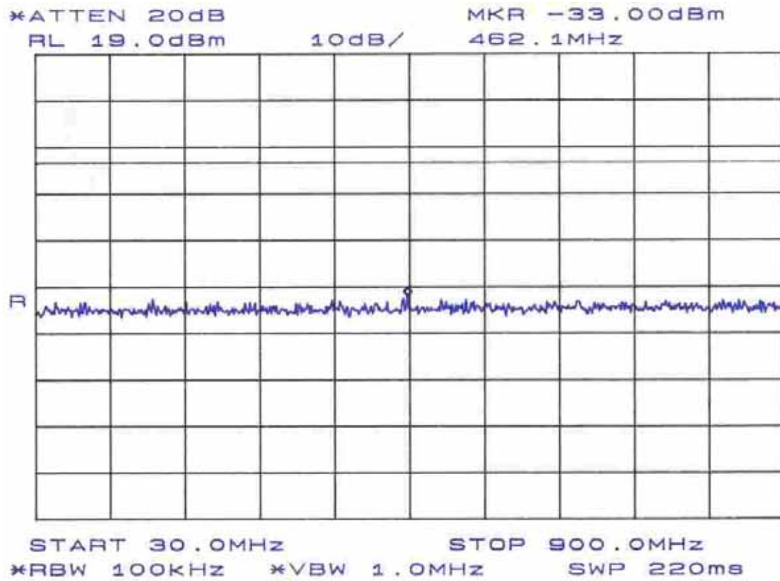
Figure 4-20. Low Power Conducted Spurious Emissions, Mid Channel 30 - 900MHz
