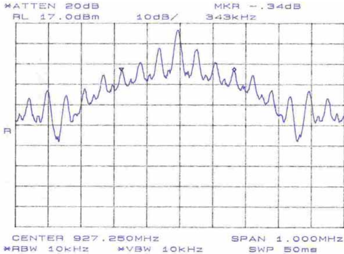
Figure 4-10. Low Power Occupied Bandwidth, High Channel
