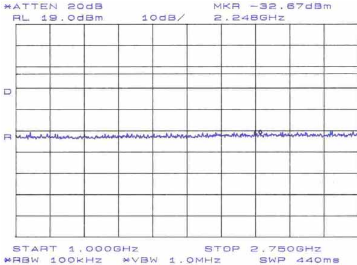
Figure 4-26. Low Power Conducted Spurious Emissions, High Channel 1 – 2.75GHz
