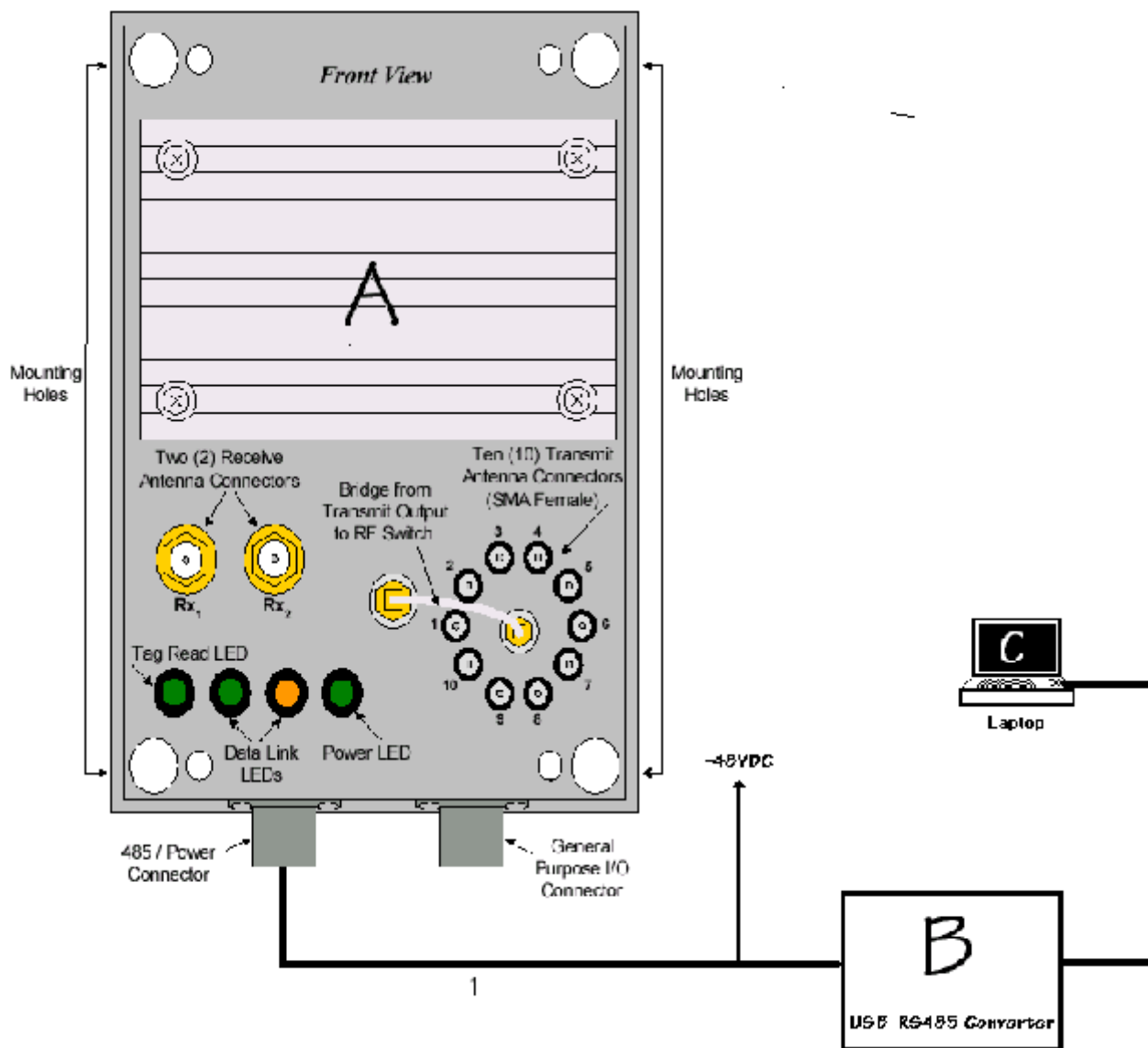
Figure 1. Test Configuration
