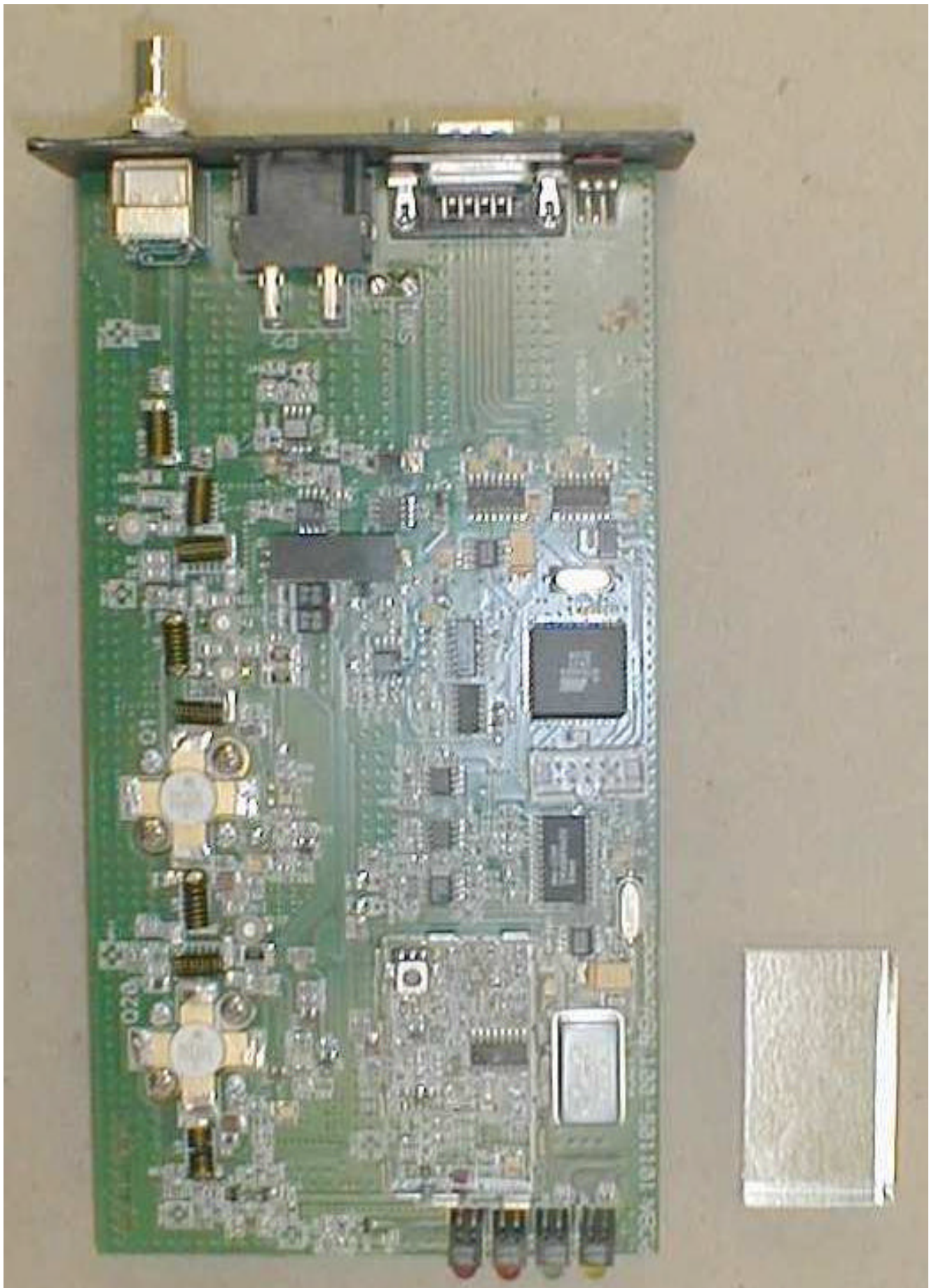
PCB Top, Shield Removed
