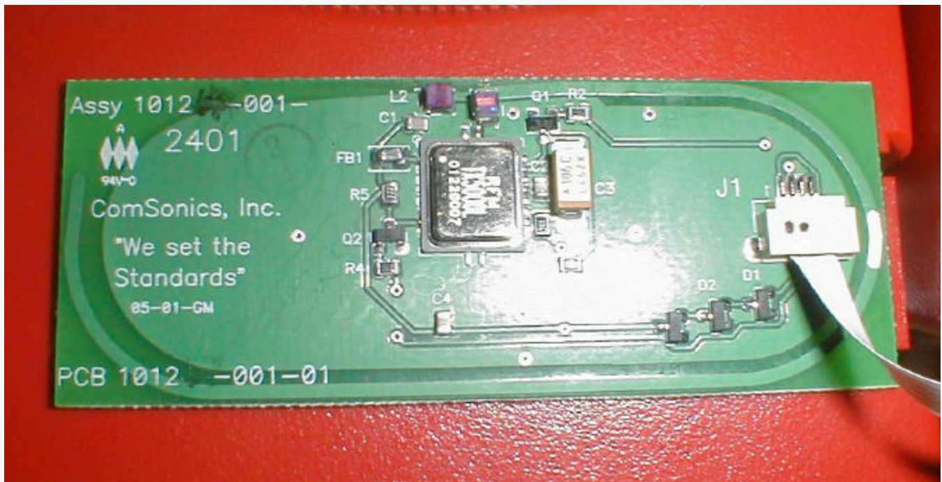
Transmitter Module Bottom View
