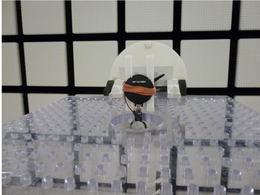
Photo 3 (RSE Setup 9 kHz to 30 MHz & 1 GHz to 12.75 GHz):
