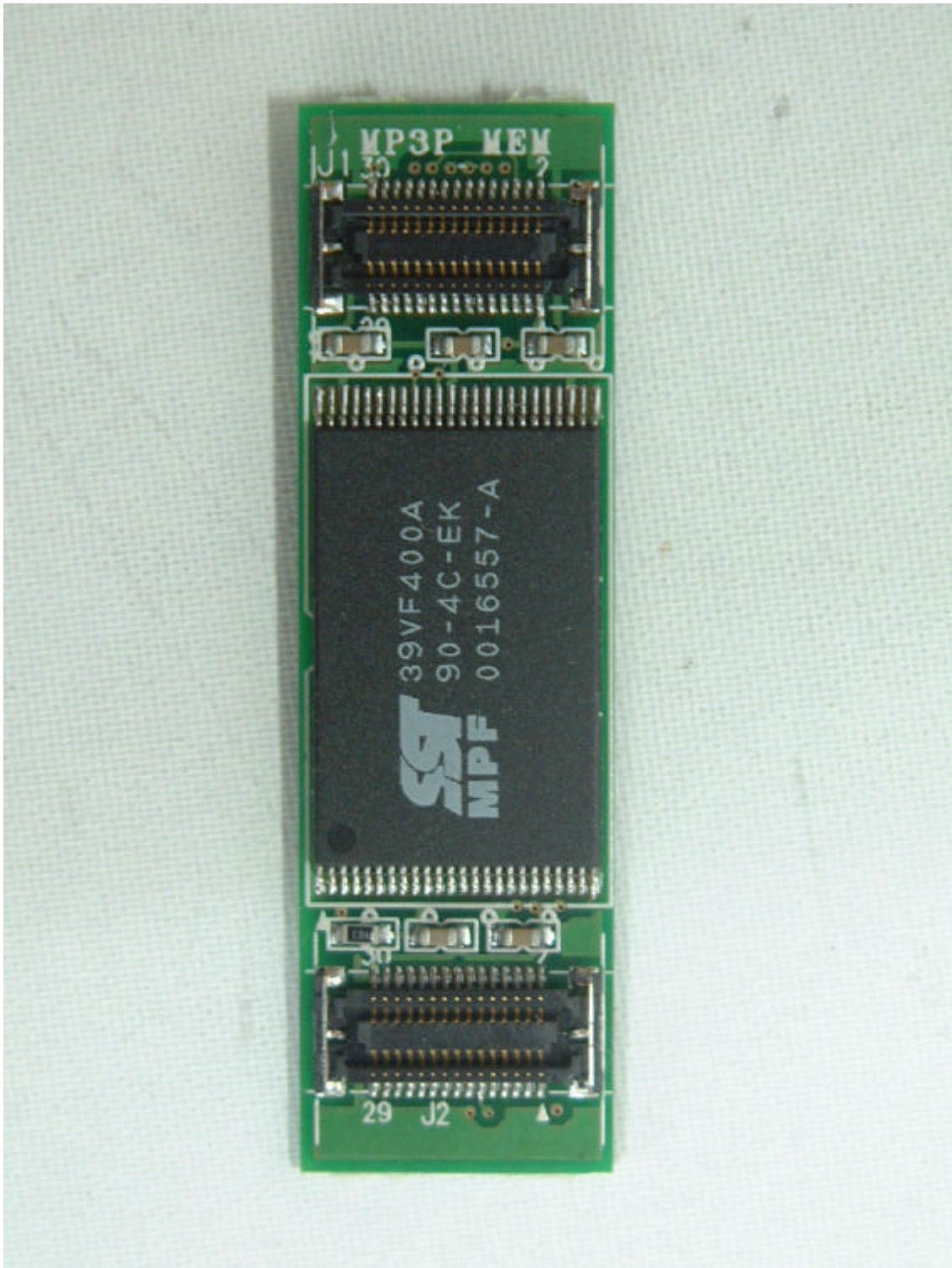
<FRONT VIEW OF MEMORY>
