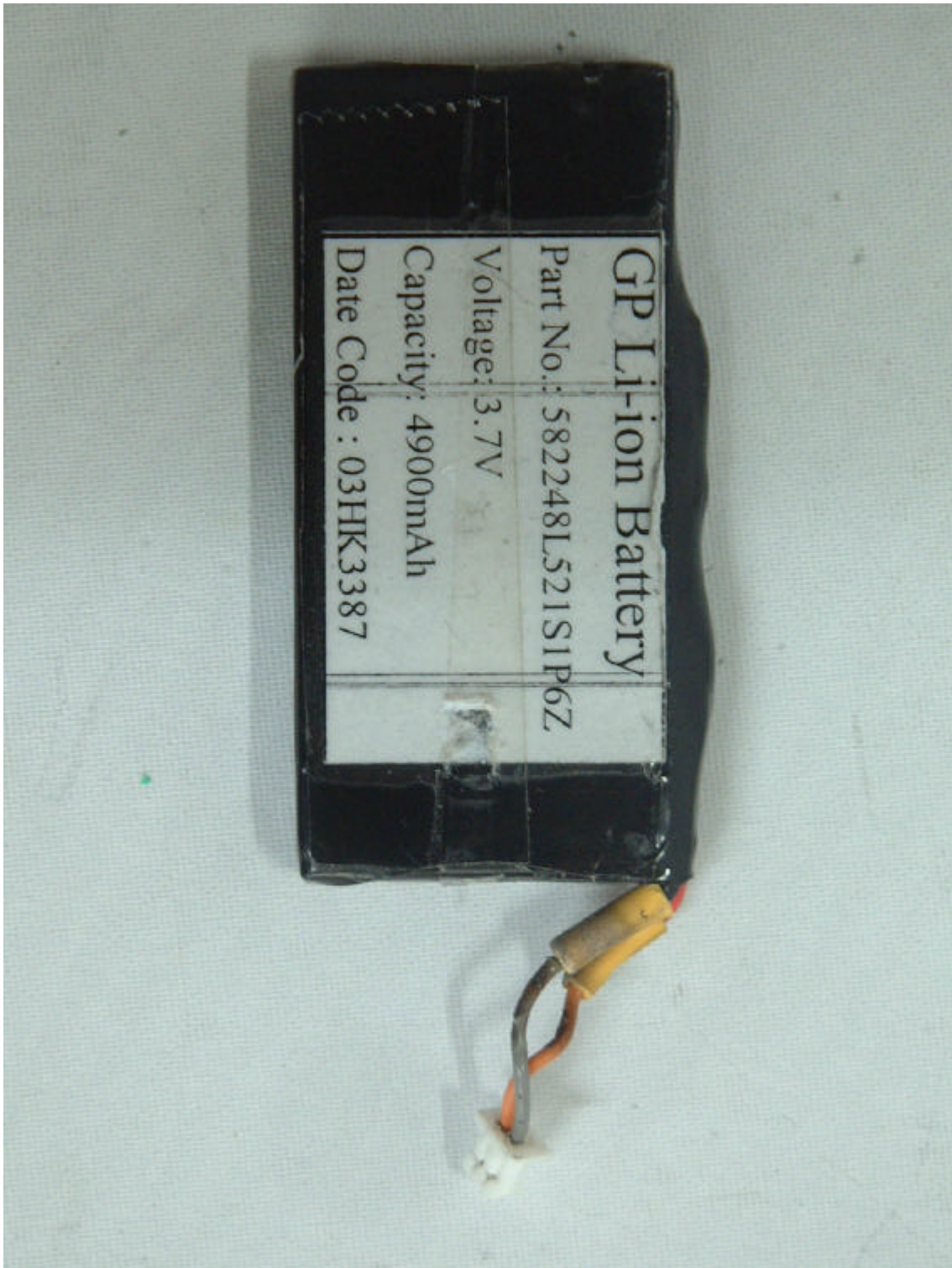
<FRONT VIEW OF BATTERY>
