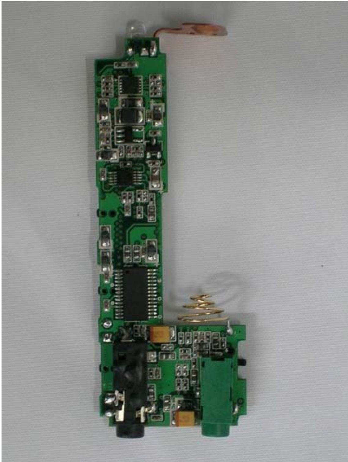
<REAR VIEW OF SUB BOARD>
