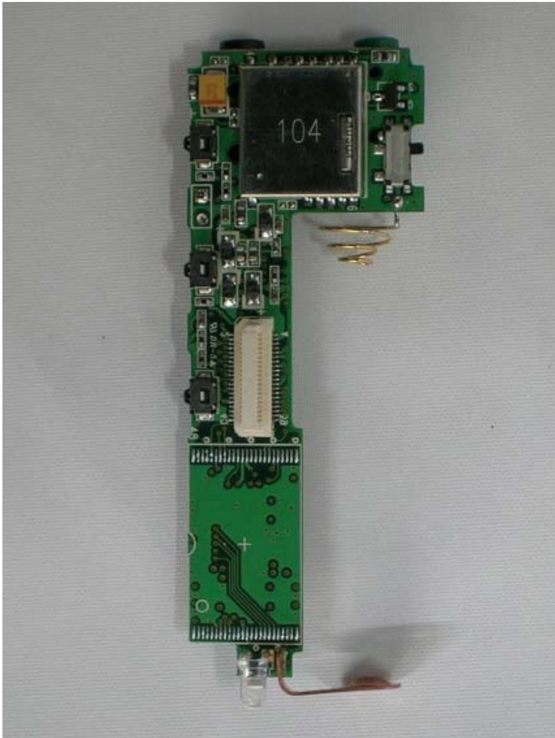
<FRONT VIEW OF SUB BOARD>
