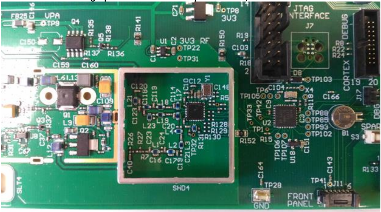
Photograph of PC Board: Component Side, Shield removed
