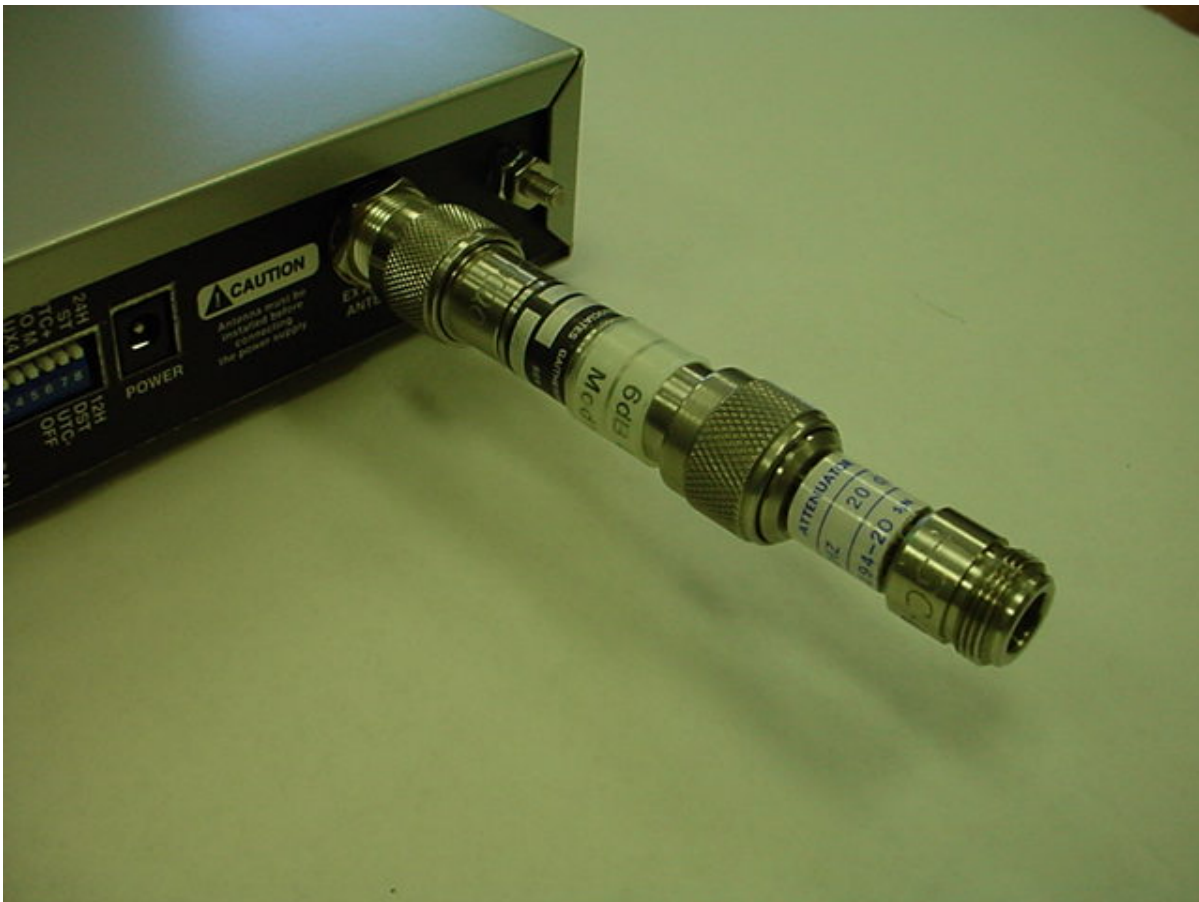
Photo Six – External Antenna Port with Dummy Load for Testing
