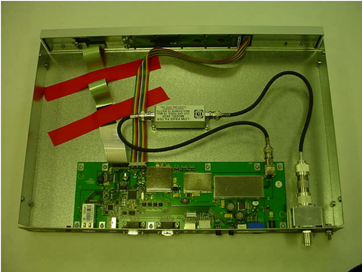
Photo Seven – External Routing of Antenna
