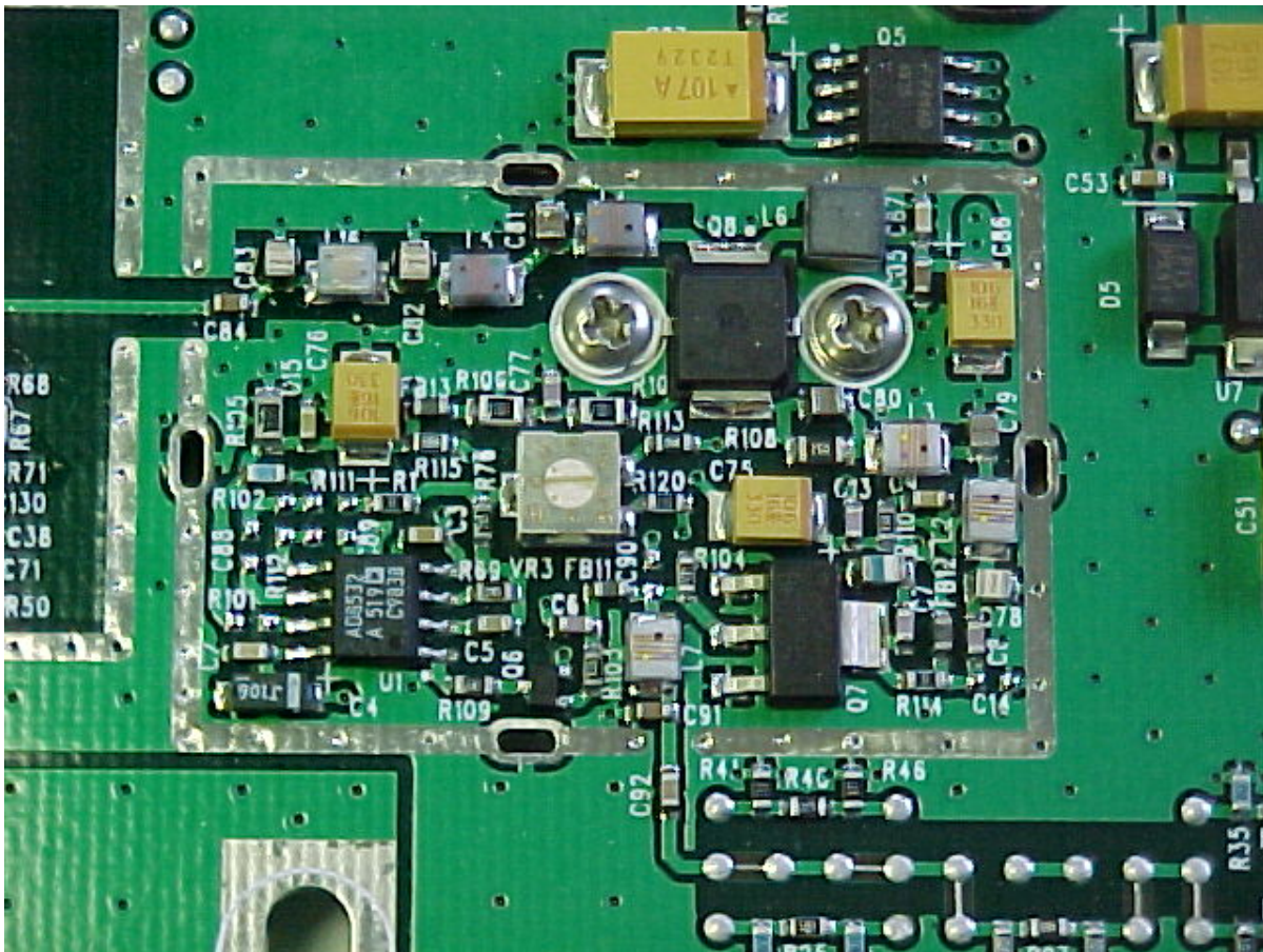
Photo Six – Internal Central Area – Shield Off
