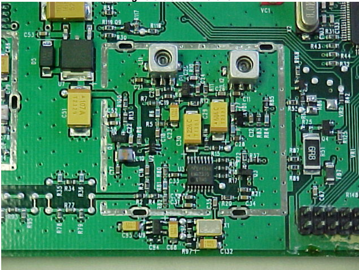
Photo Seven – Internal Right Side – Shield Off
