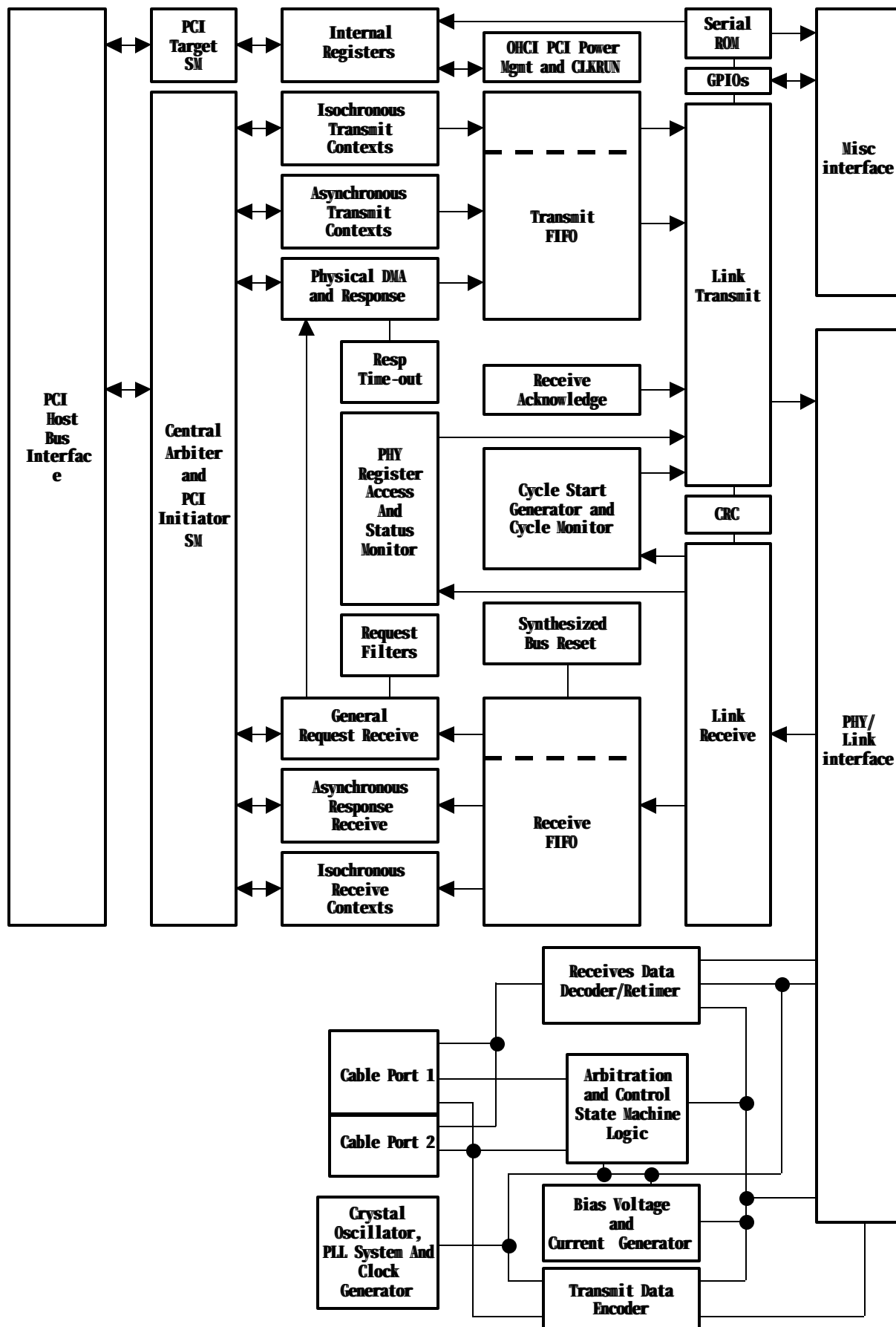
SFW-1112 Block Diagram
