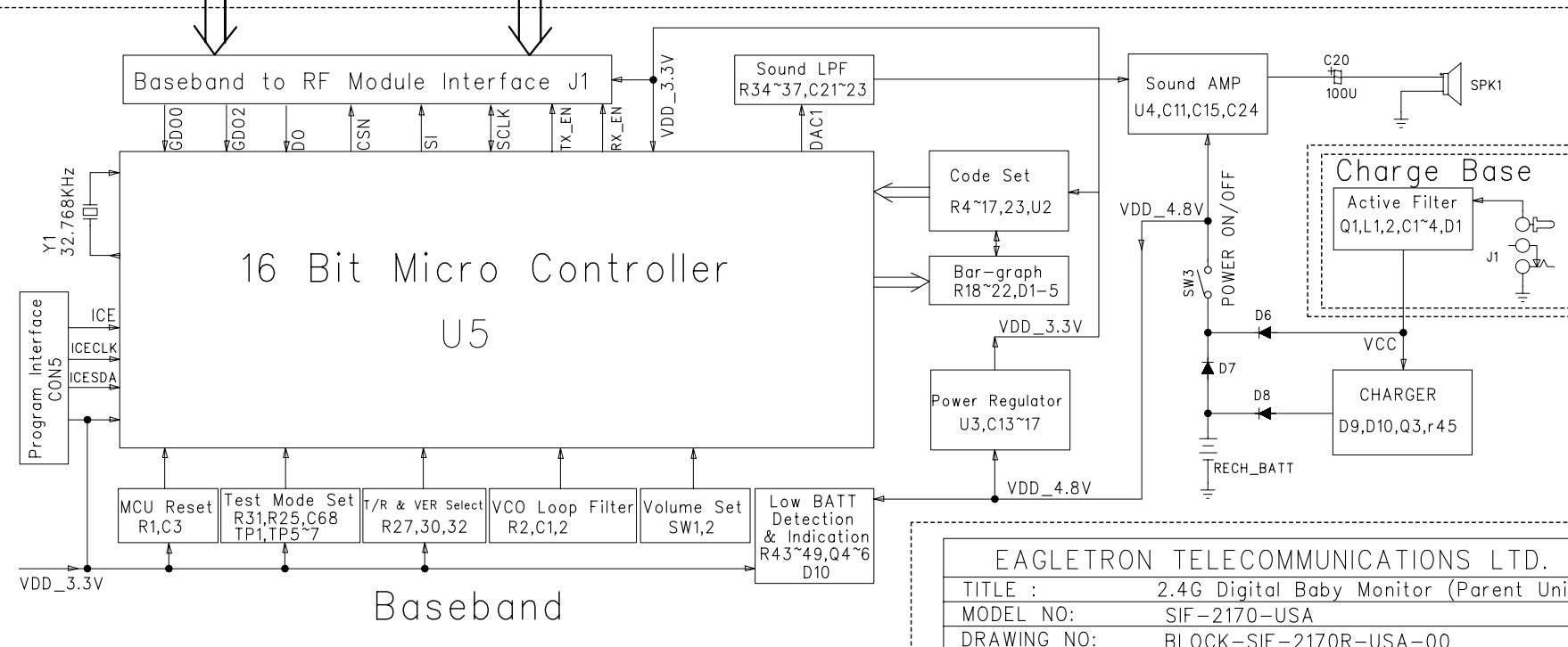
SIF-2170-USA Parent Unit Block Diagram
