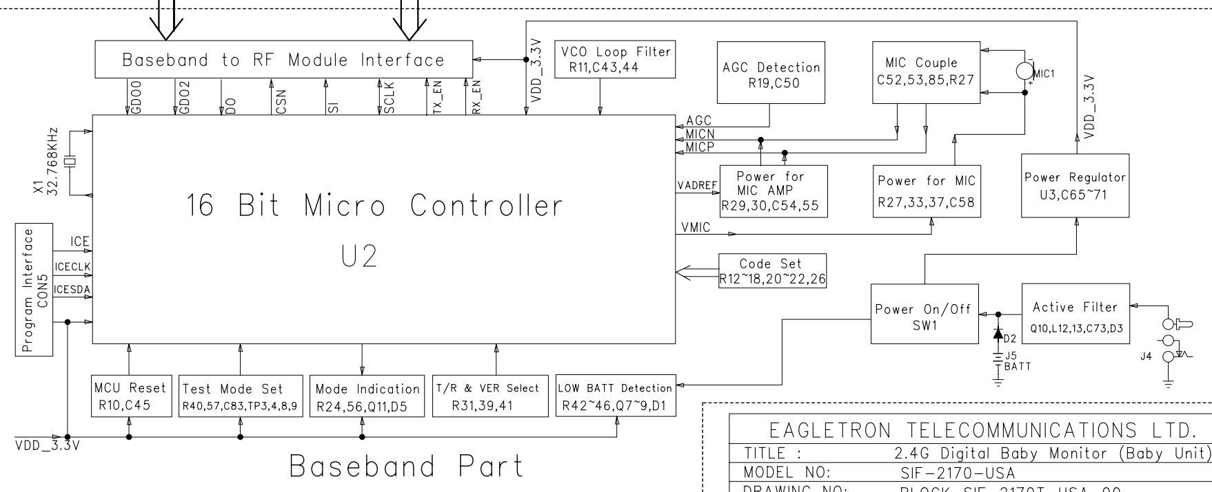
SIF-2170-USA Baby Unit Block Diagram
