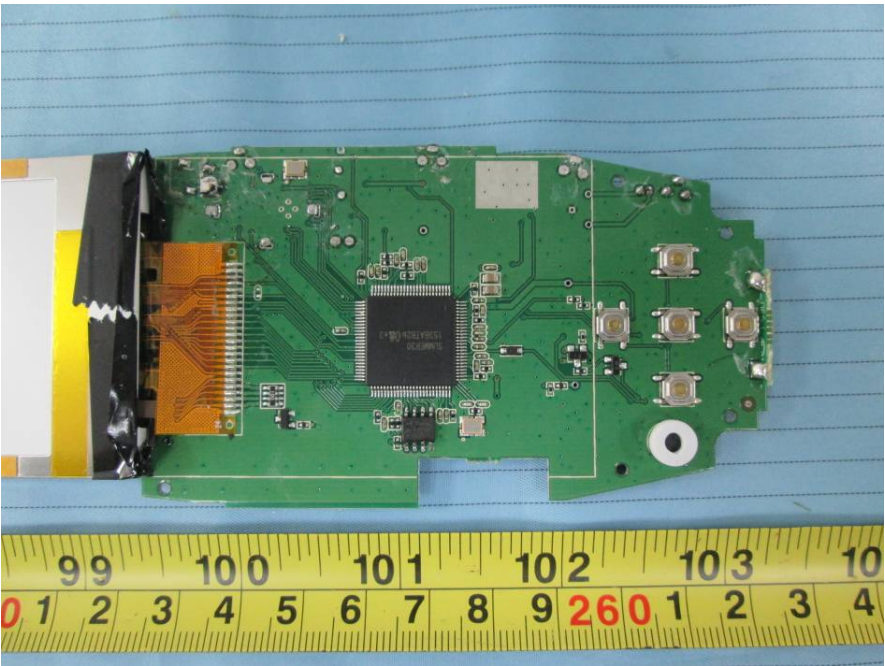
EUT –Main Board 2 Bottom View 1
