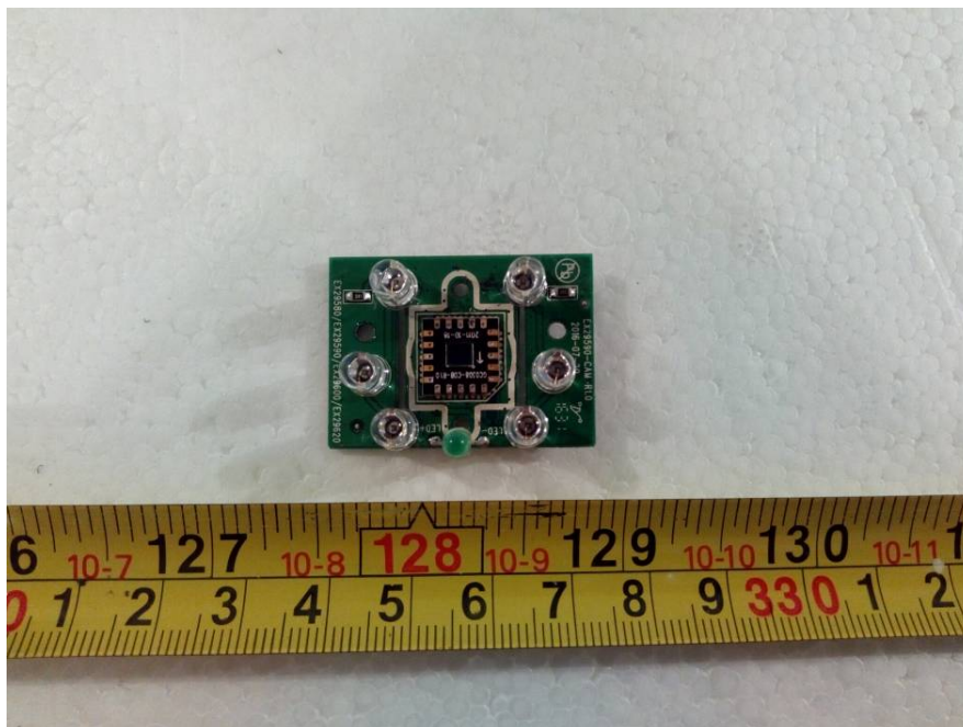
EUT – Main Board 2 Top View 2
