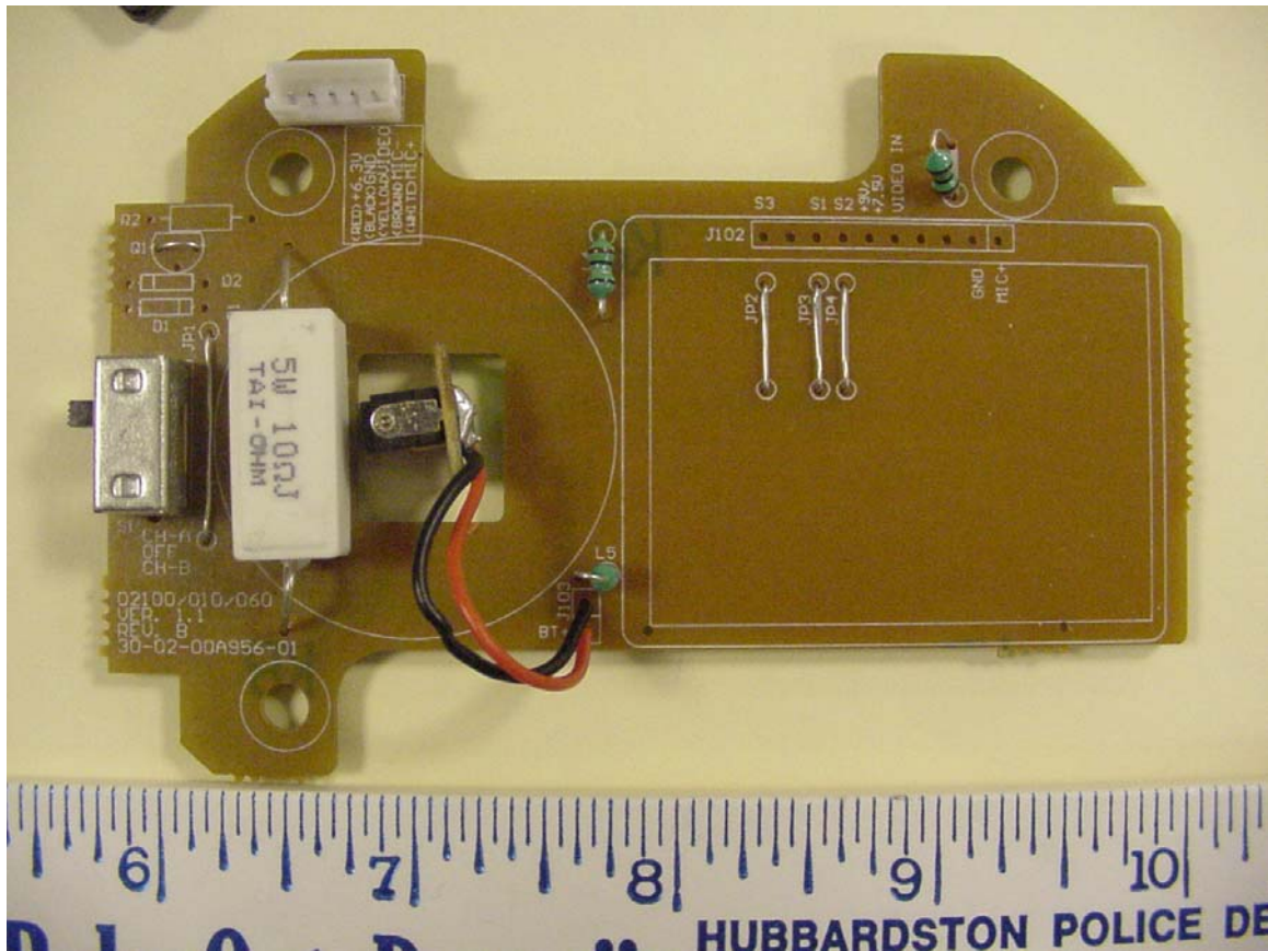
Main board with RF board removed
