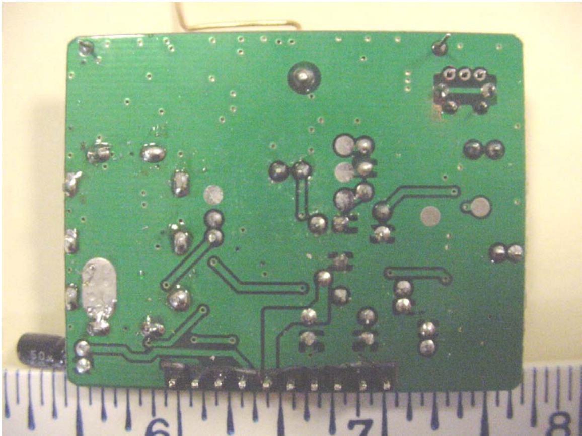
RF board Solder Side, removed from main board.
