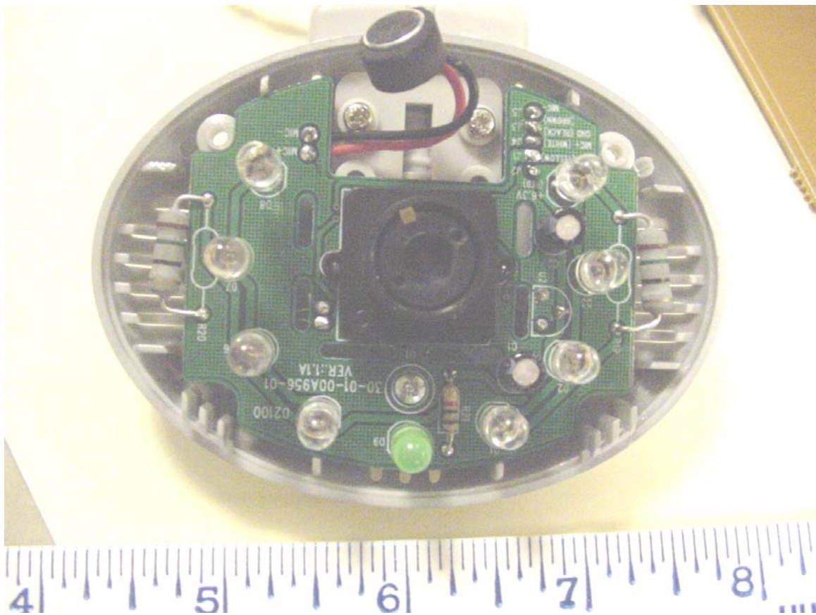
Component side of video board and microphone.
