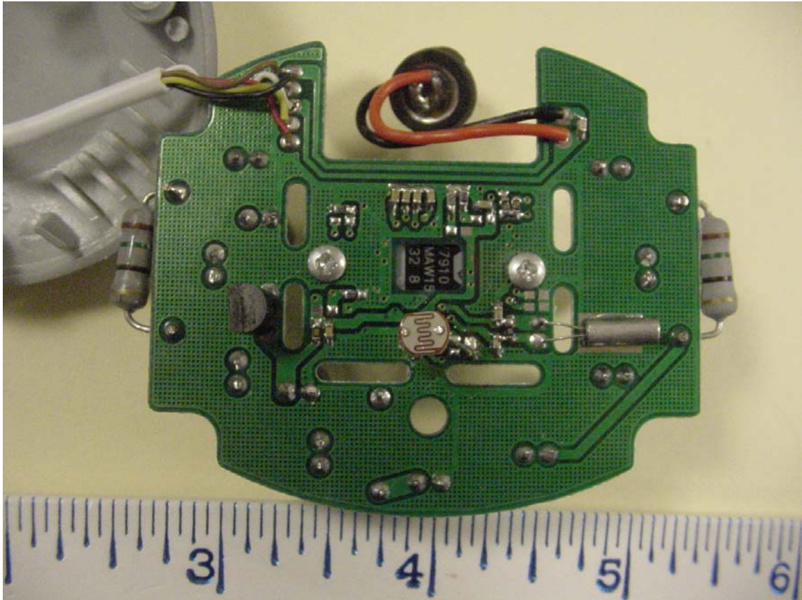
Rear of video board, LED dimmer control and microphone.
