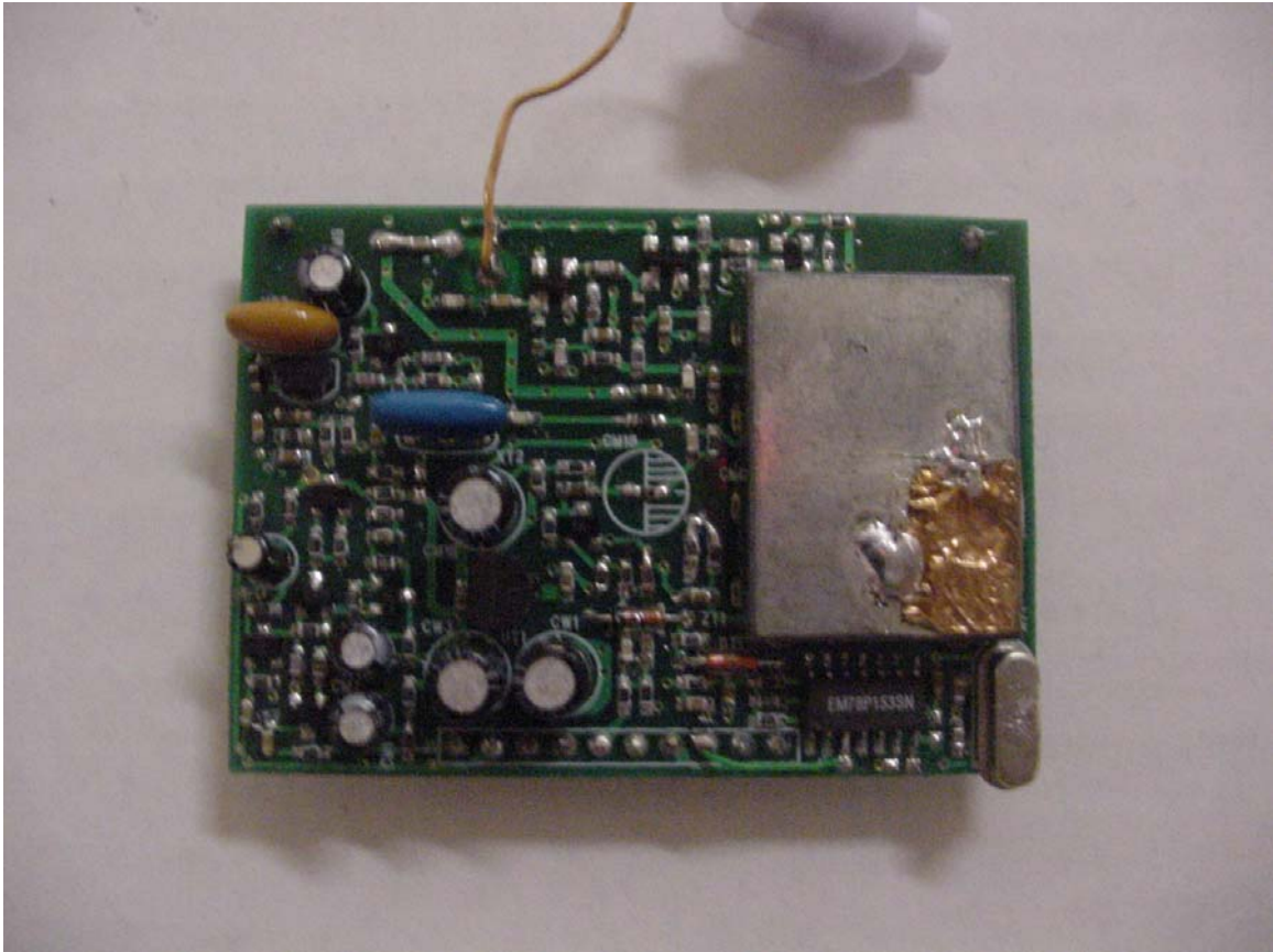
Small PCB board, Top
